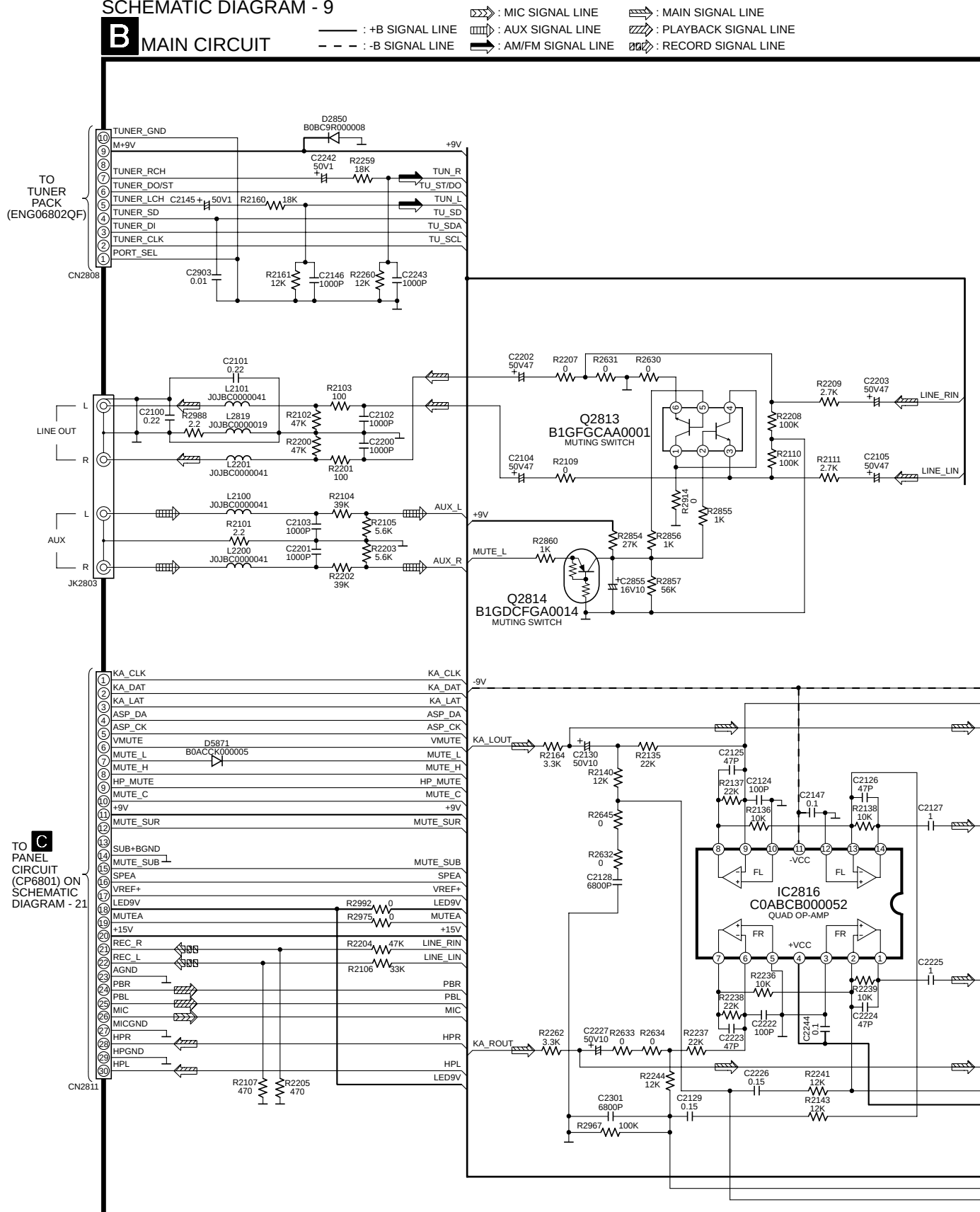
SCHEMATIC DIAGRAM - 9
