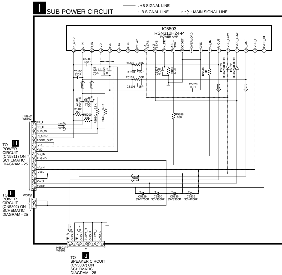
SCHEMATIC DIAGRAM - 26
