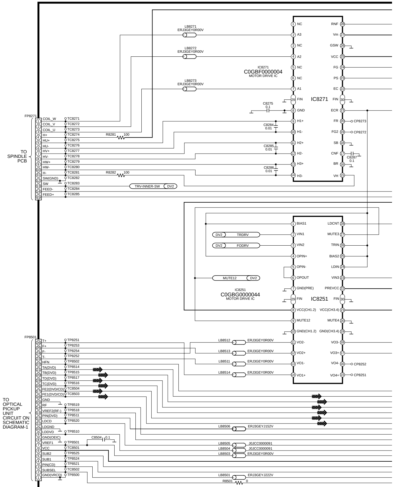
SCHEMATIC DIAGRAM - 2
