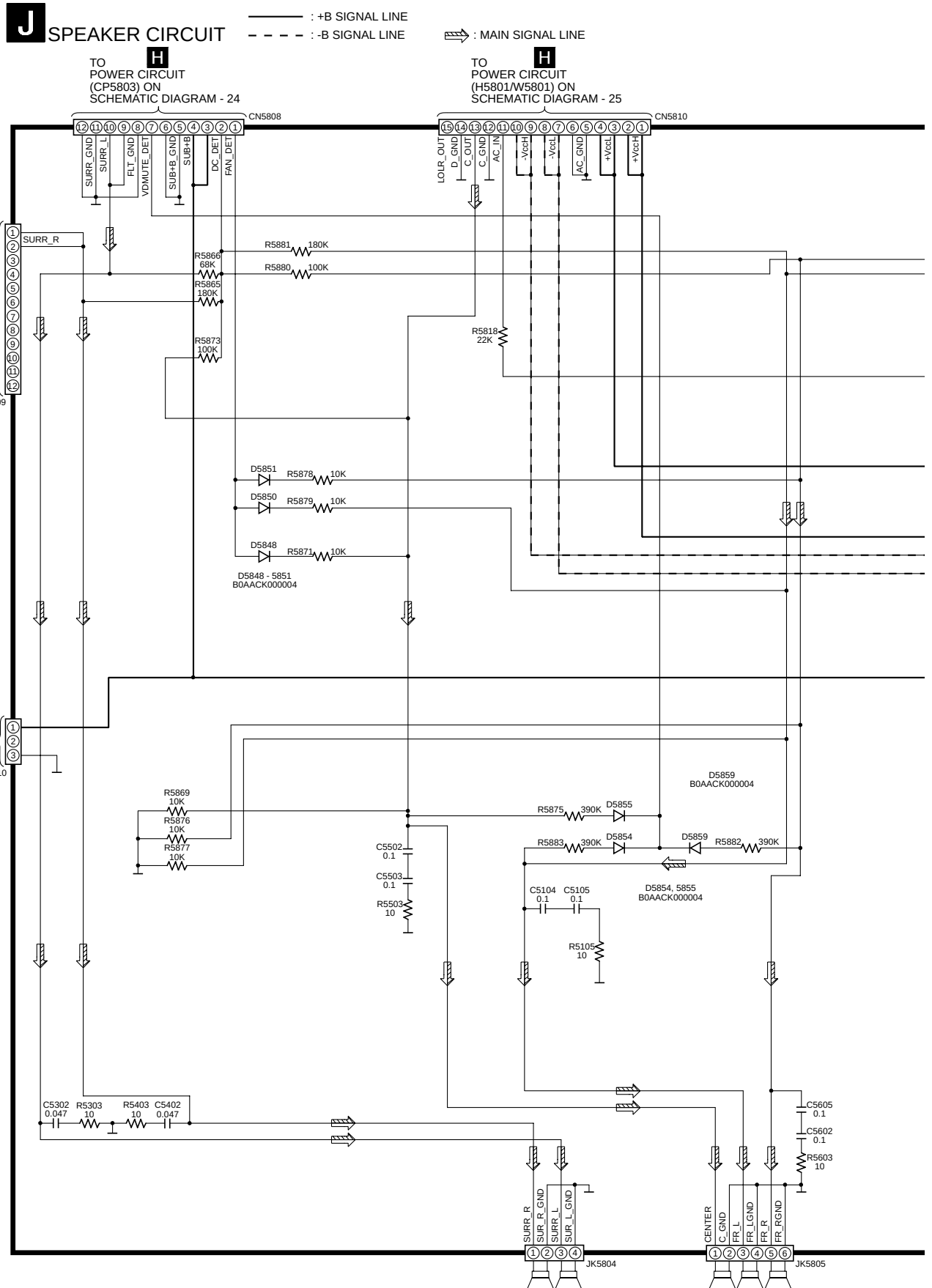
SCHEMATIC DIAGRAM - 27
