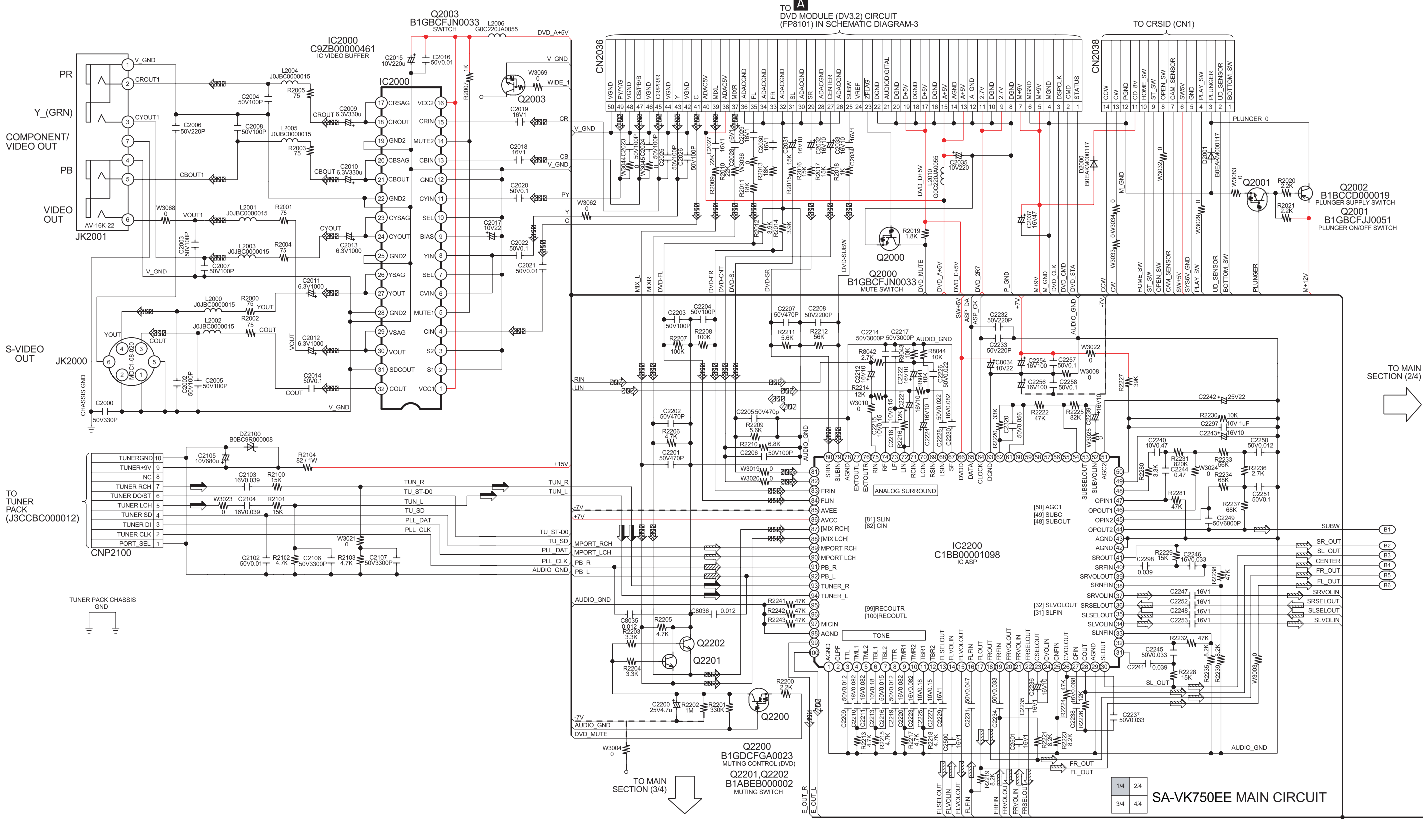
SCHEMATIC DIAGRAM - 6
