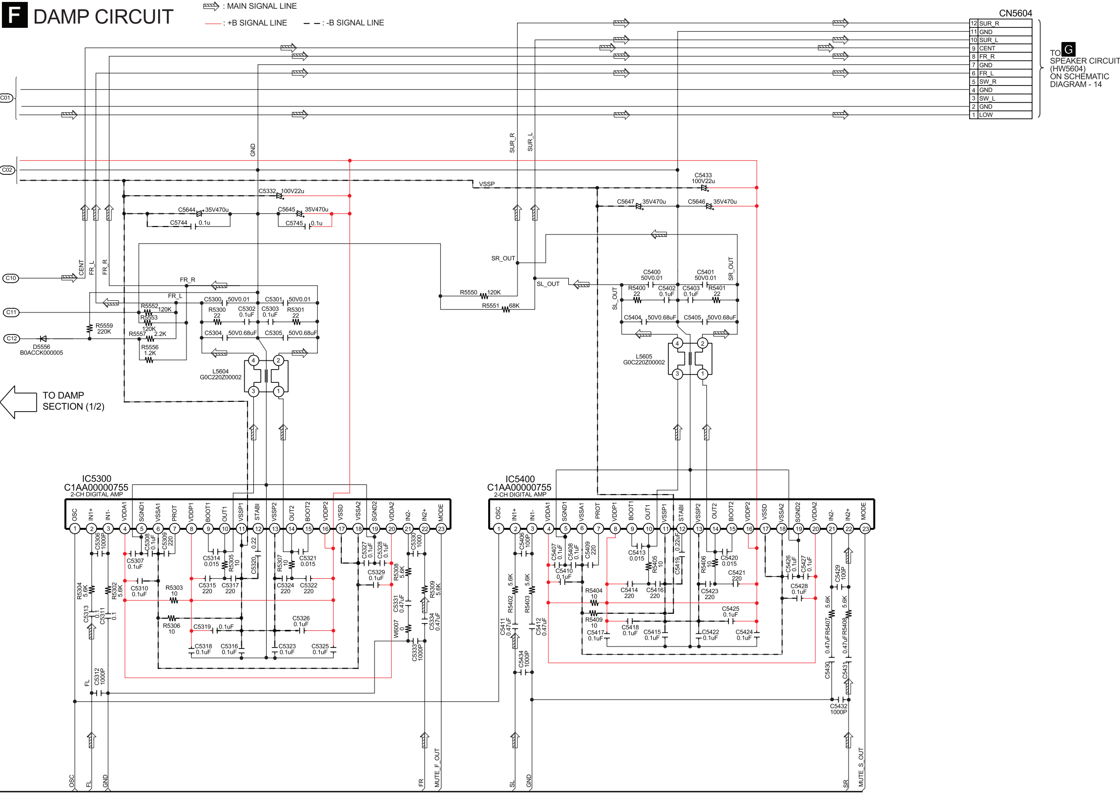
SCHEMATIC DIAGRAM - 13
