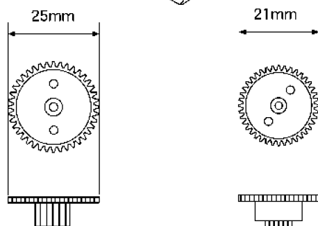
UD. speed down gear No.1 (White)
