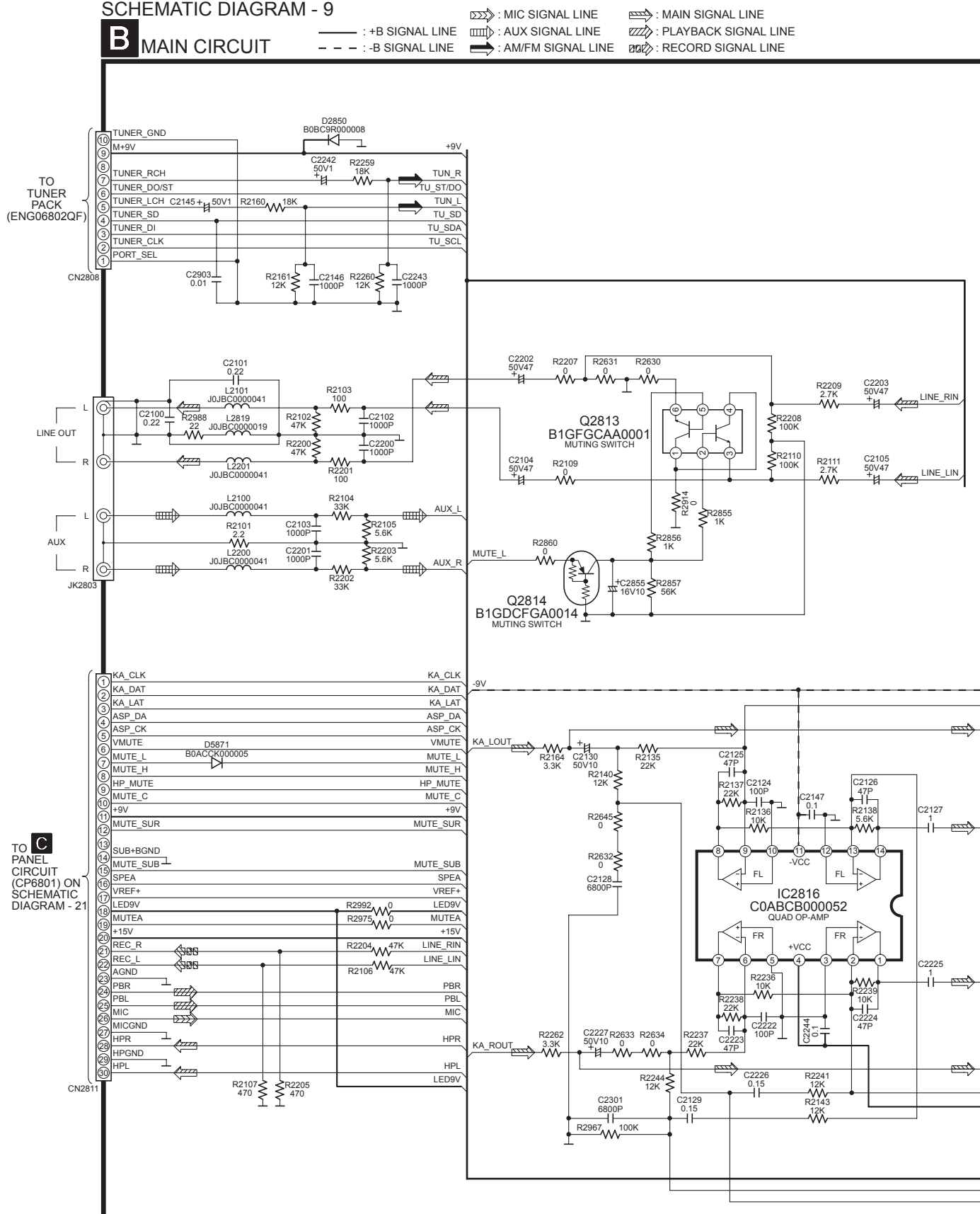
SCHEMATIC DIAGRAM - 9
