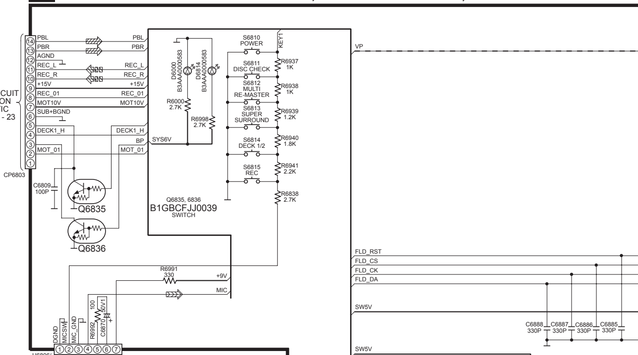
SCHEMATIC DIAGRAM - 18
