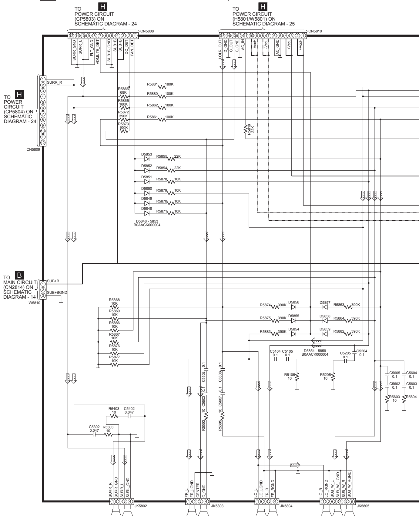
SCHEMATIC DIAGRAM - 27
