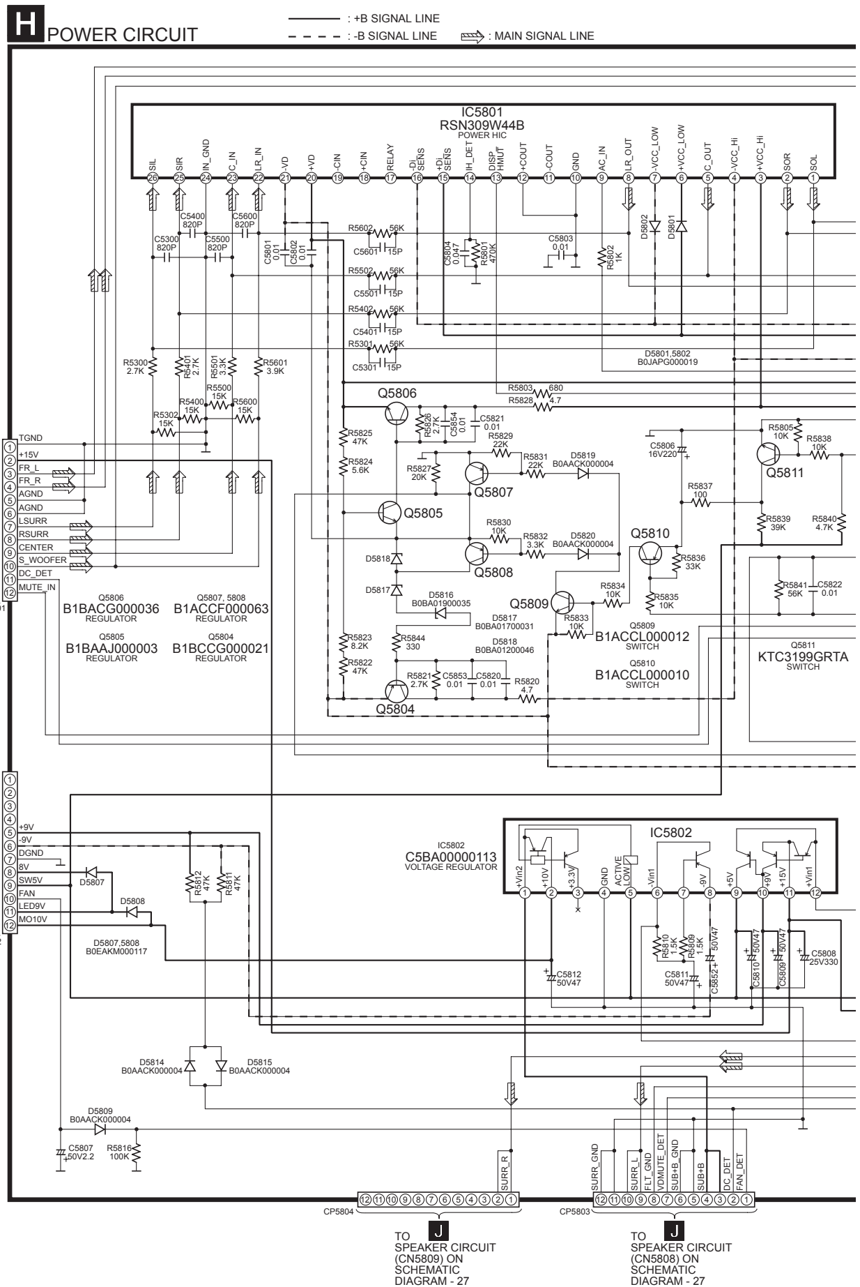
SCHEMATIC DIAGRAM - 24
