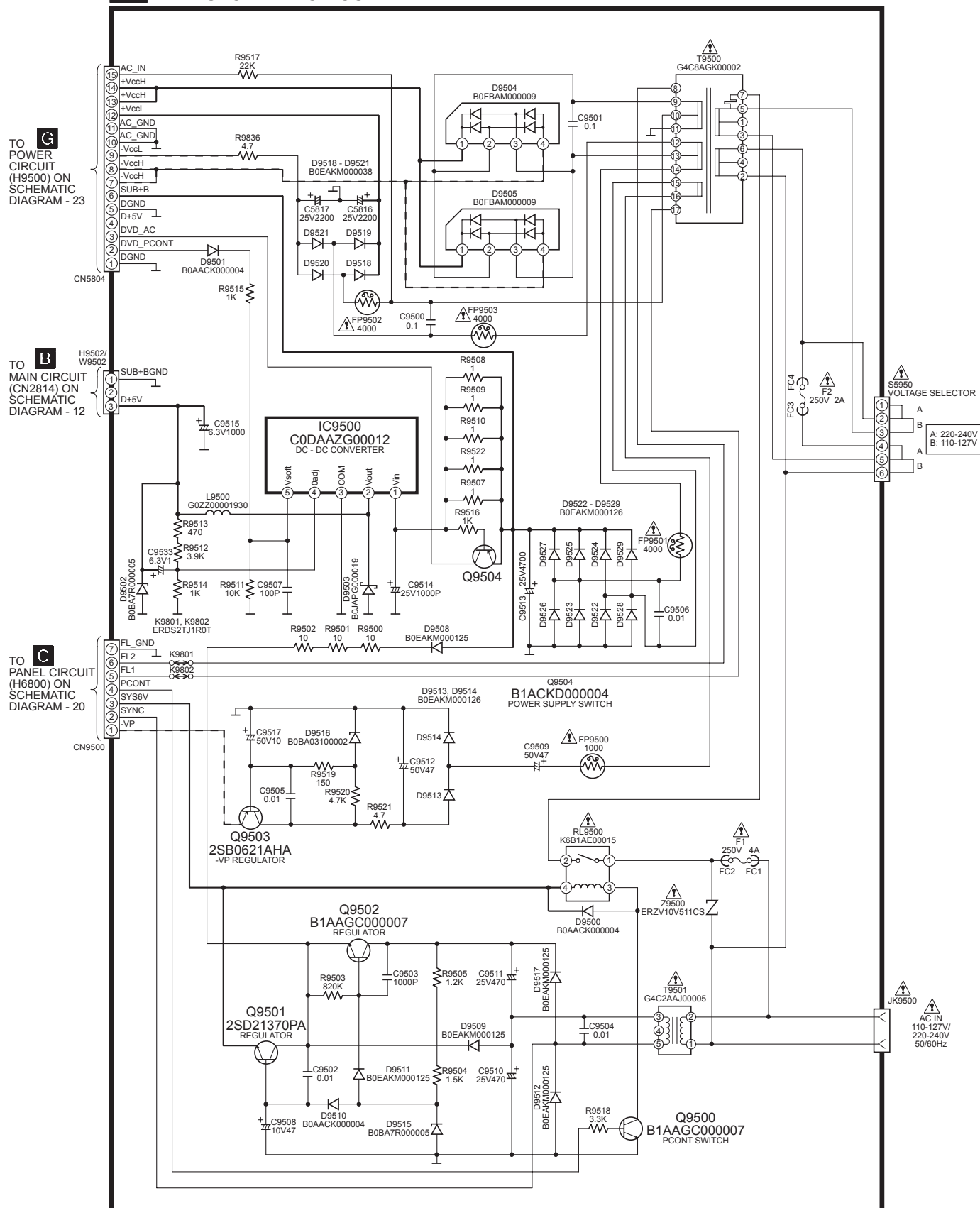
SCHEMATIC DIAGRAM - 25
