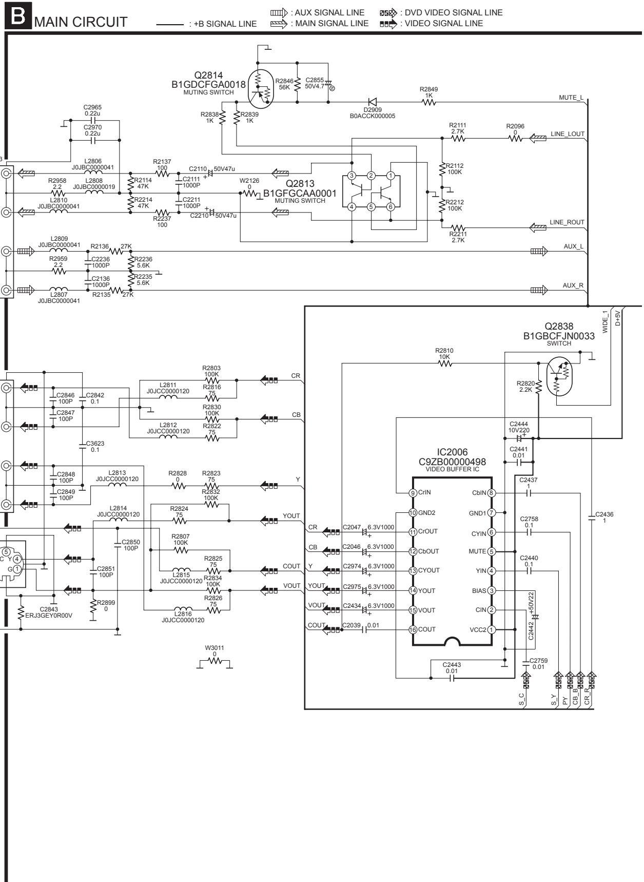
SCHEMATIC DIAGRAM - 10
