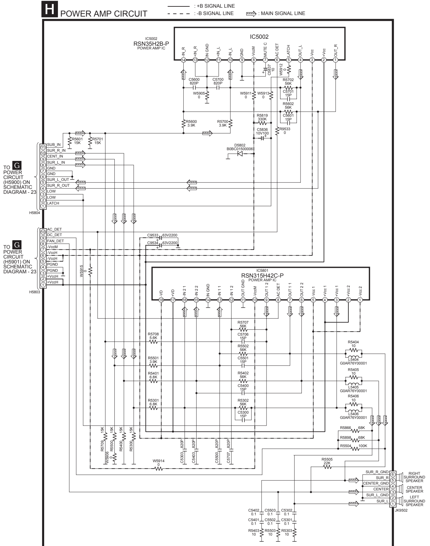
SCHEMATIC DIAGRAM - 24
