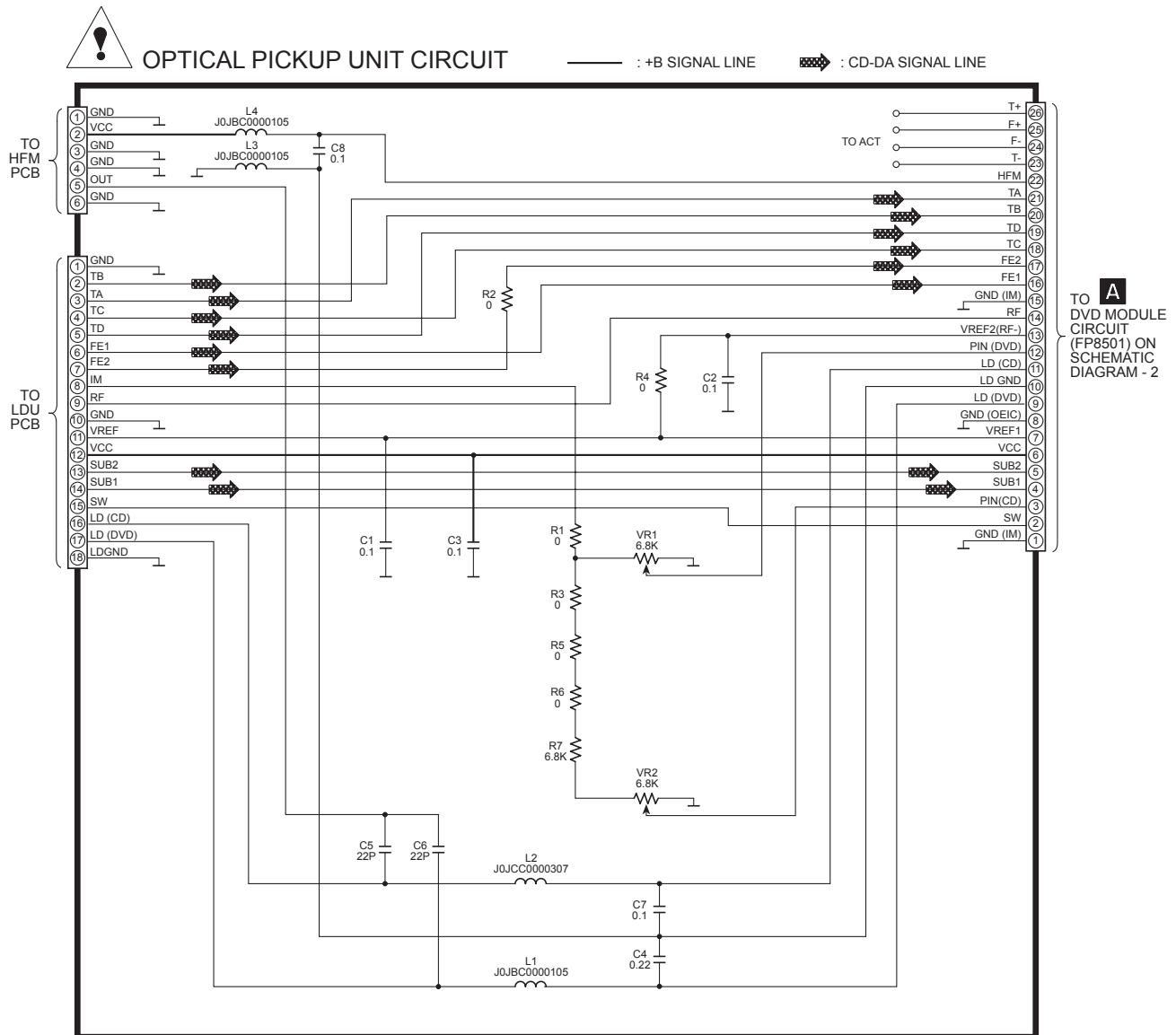
SCHEMATIC DIAGRAM - 1
