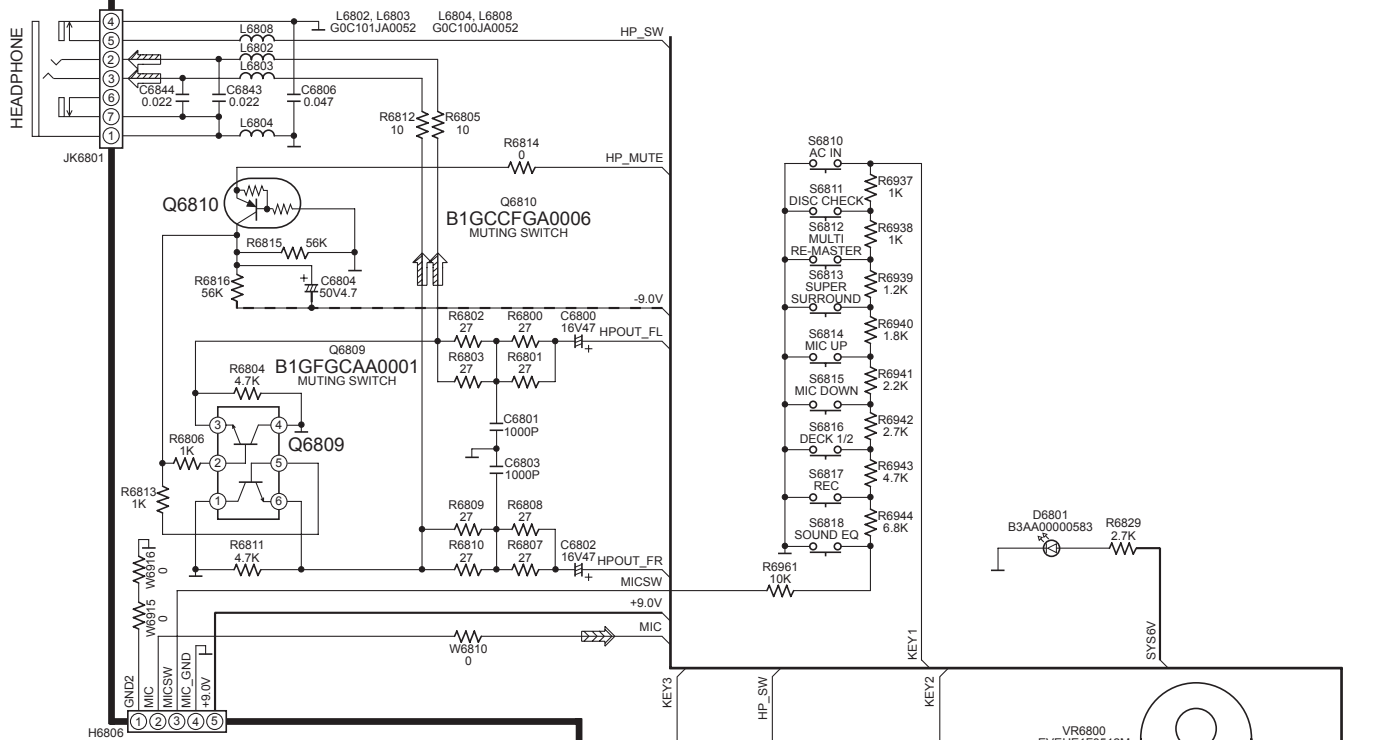
SCHEMATIC DIAGRAM - 19
