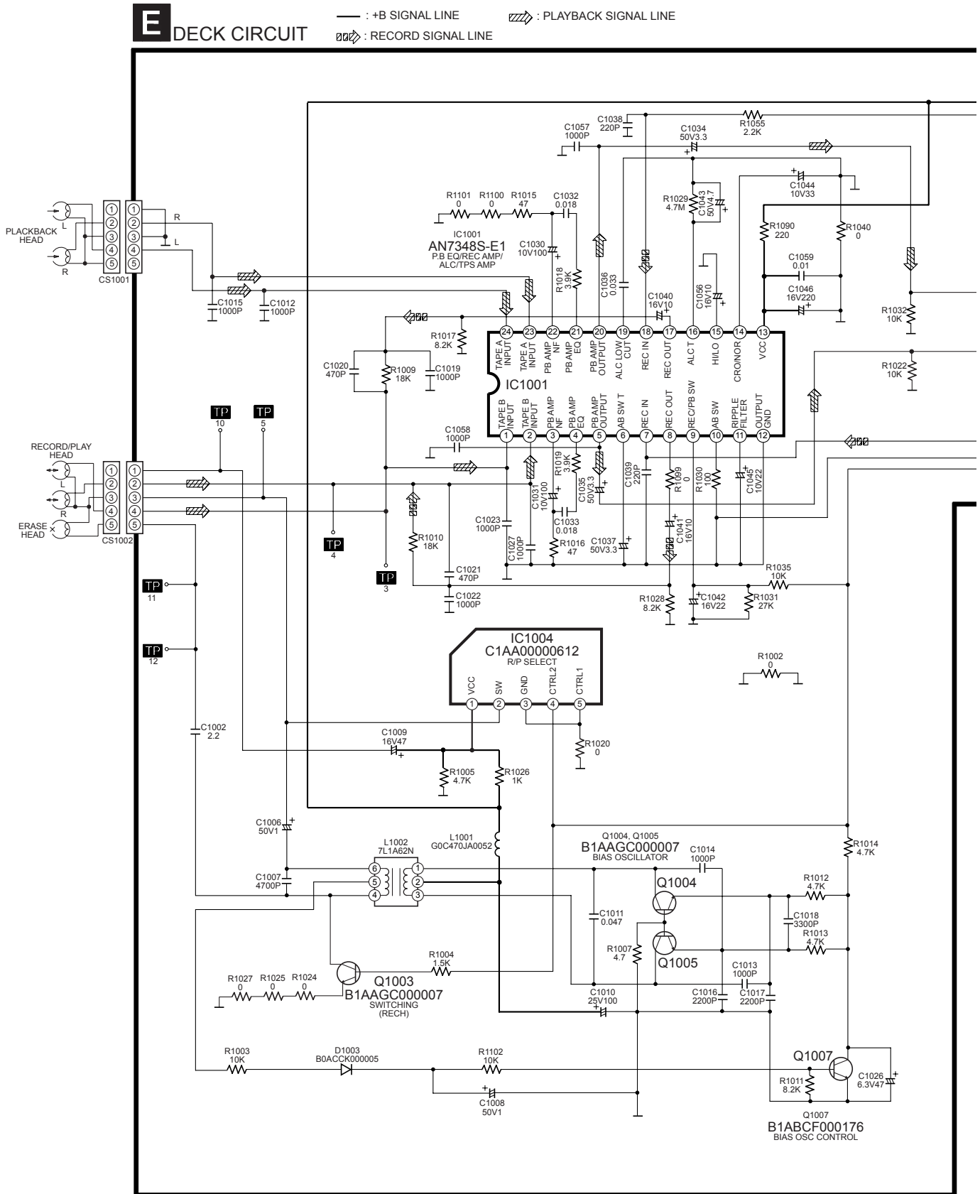
SCHEMATIC DIAGRAM - 21
