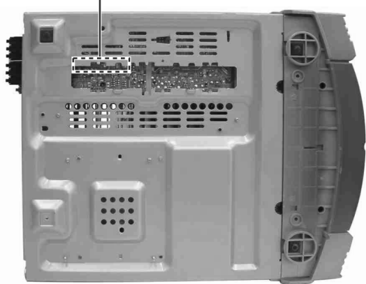
Solder terminal
