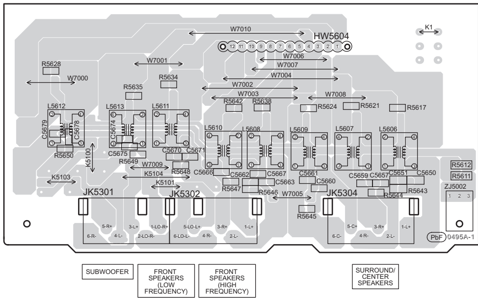
L SPEAKER P.C.B. (REPV0144A)
