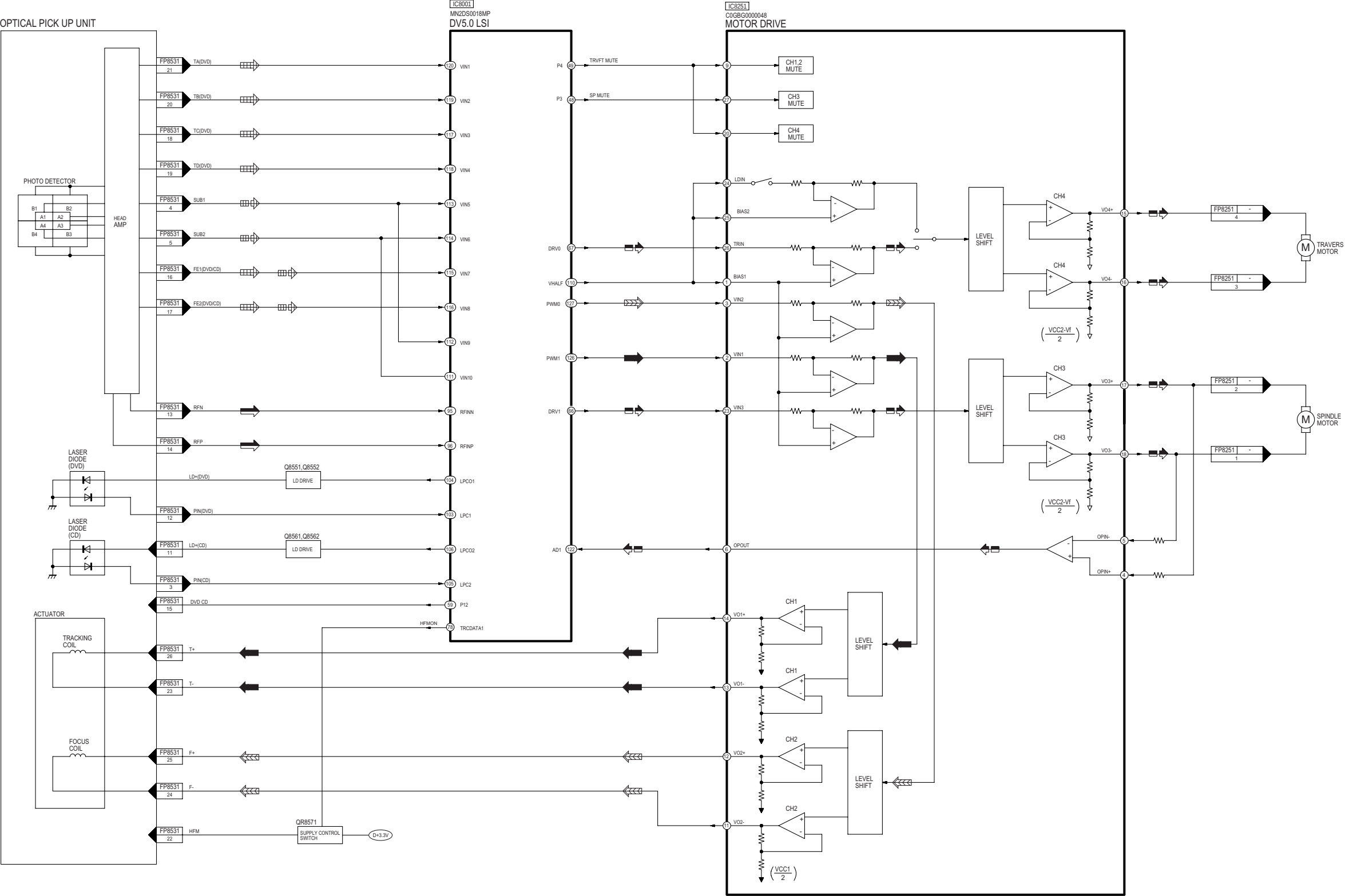
SA-VK960GC/GCS/GCT/GS DVD (SERVO) BLOCK DIAGRAM
