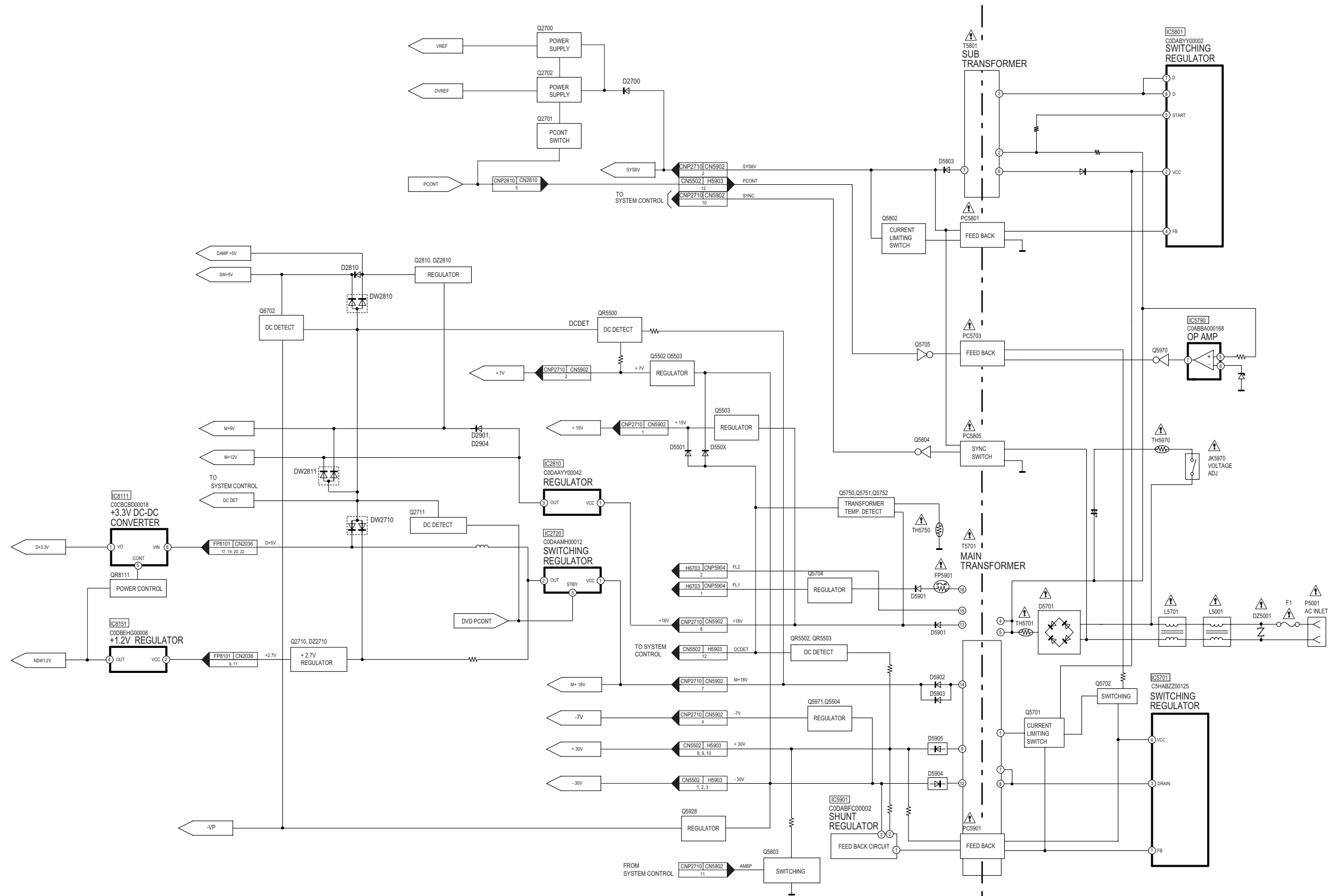
SA-VK960GC/GCS/GCT/GS POWER BLOCK DIAGRAM
