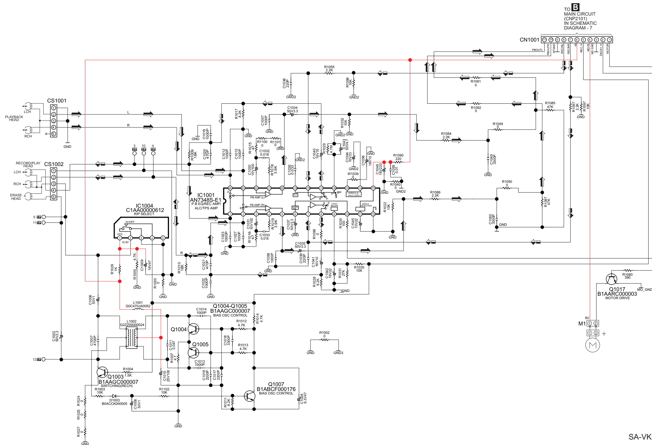
SCHEMATIC DIAGRAM - 11
