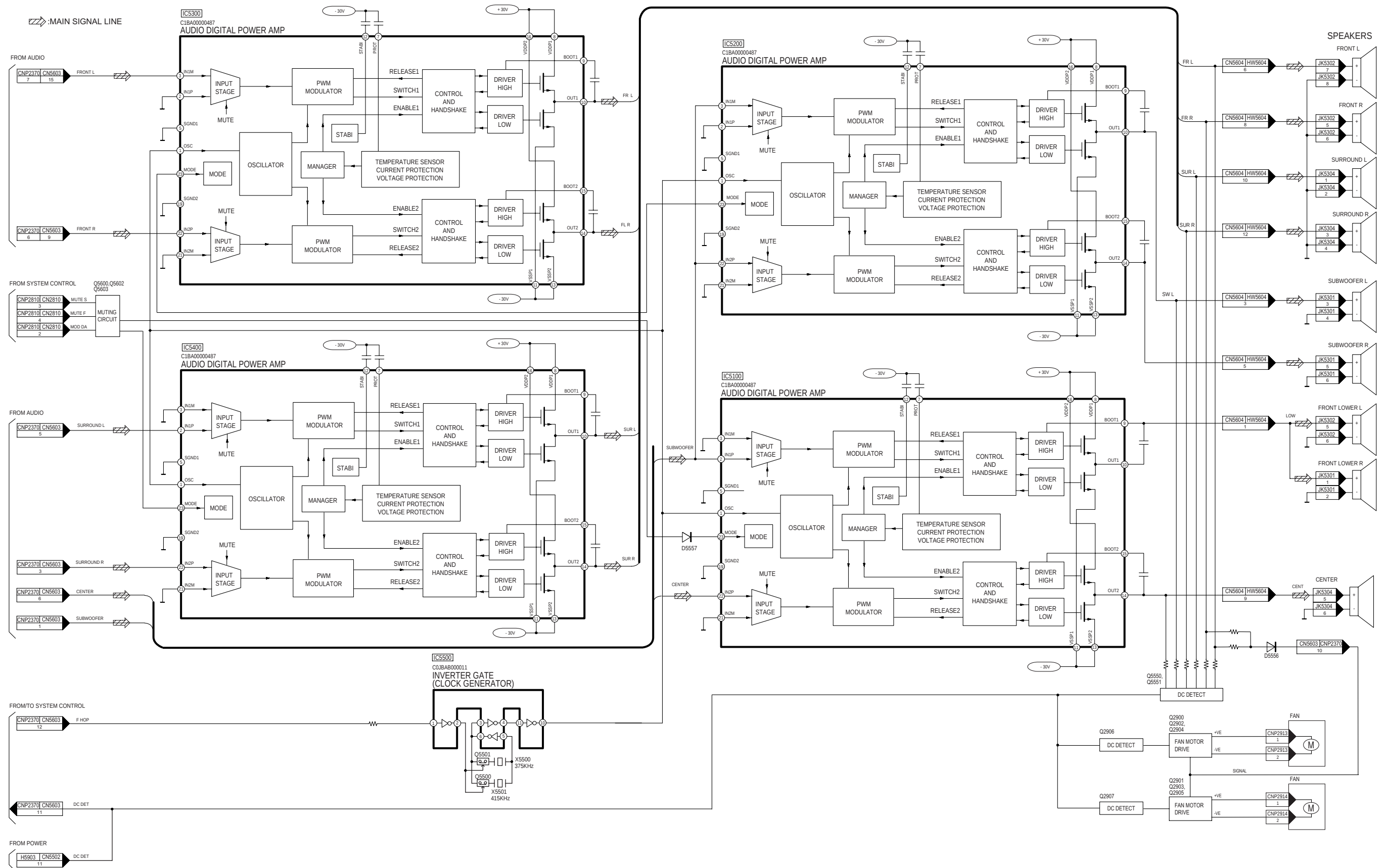
SA-VK960GC/GCS/GCT/GS AUDIO DIGITAL AMP BLOCK DIAGRAM
