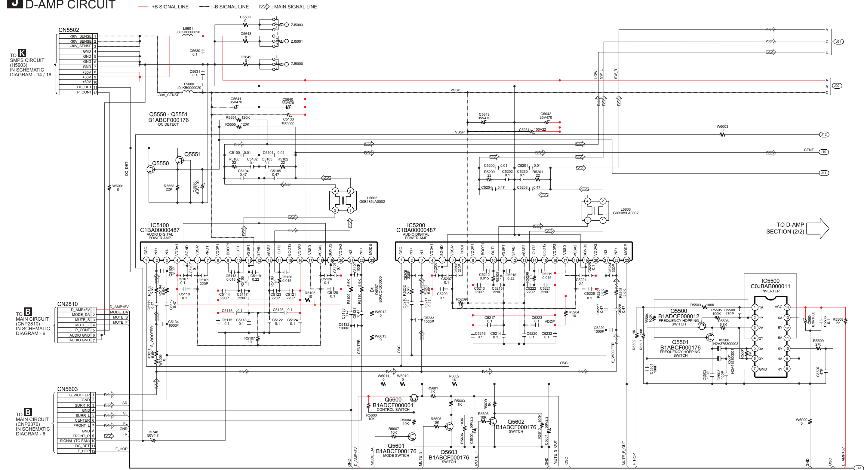
SCHEMATIC DIAGRAM - 12
