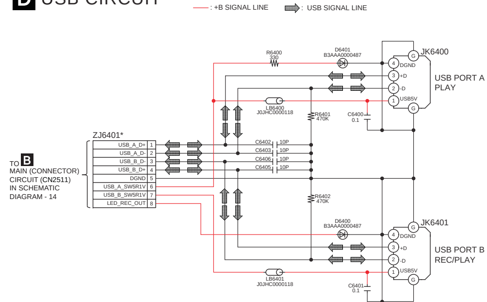
SCHEMATIC DIAGRAM - 17
