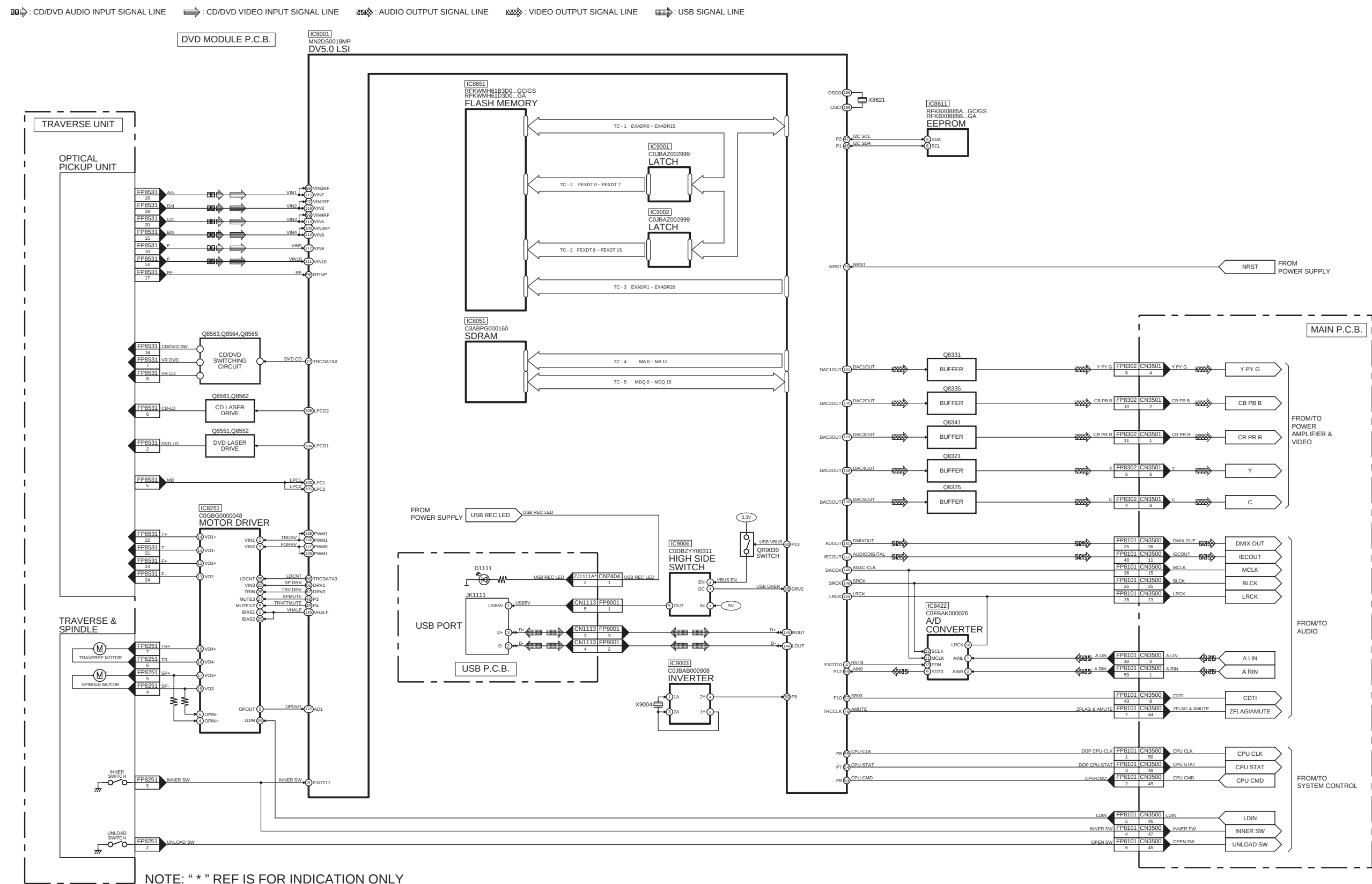
SA-VKX60GA/GC/GS DVD MODULE BLOCK DIAGRAM
