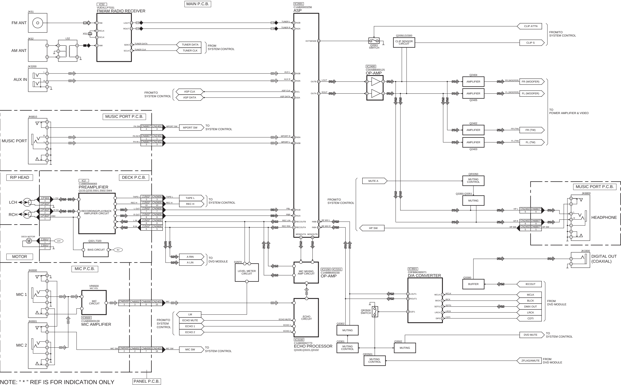
SA-VKX60GA/GC/GS AUDIO BLOCK DIAGRAM
