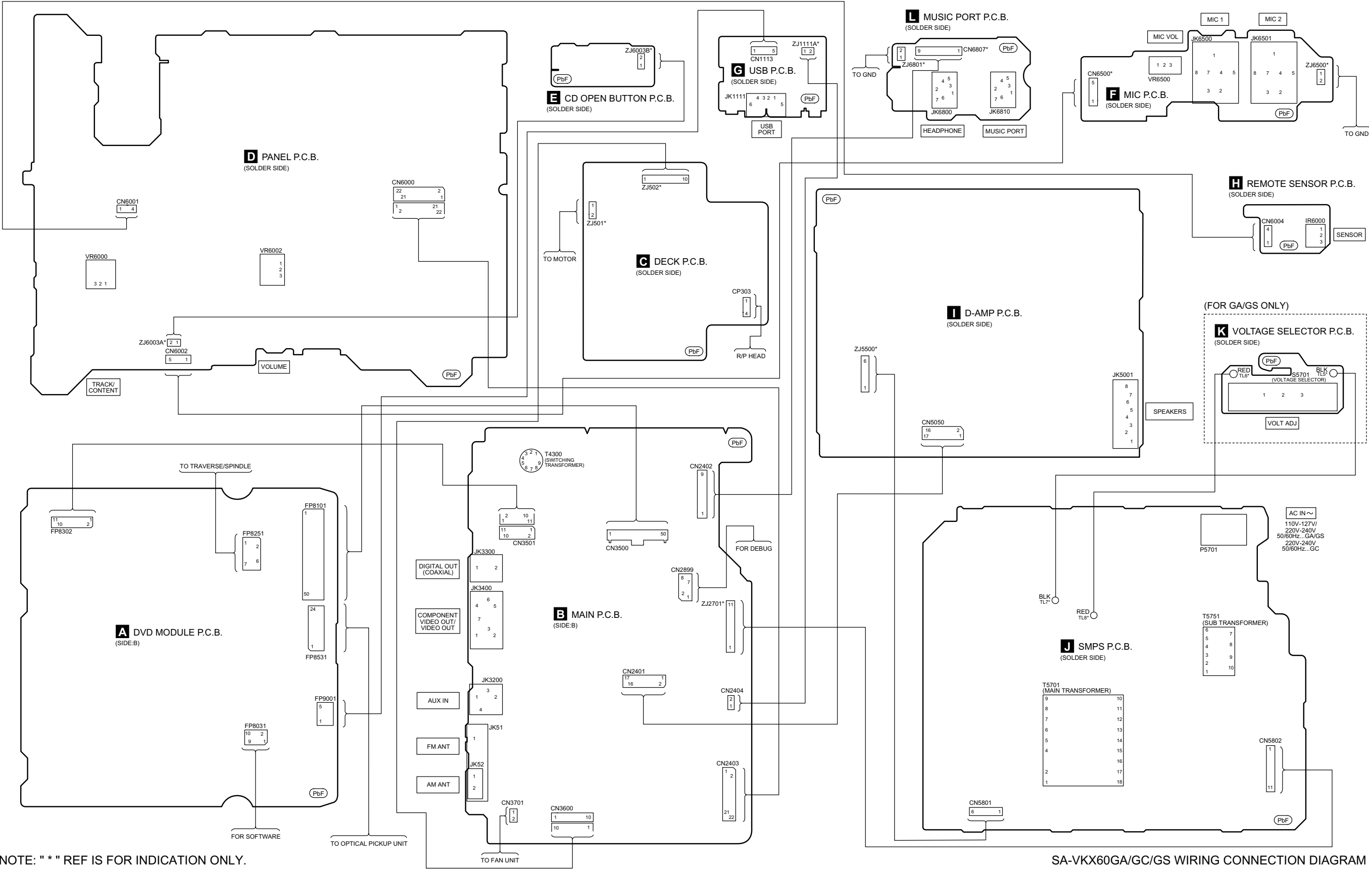
SA-VKX60GA/GC/GS WIRING CONNECTION DIAGRAM
