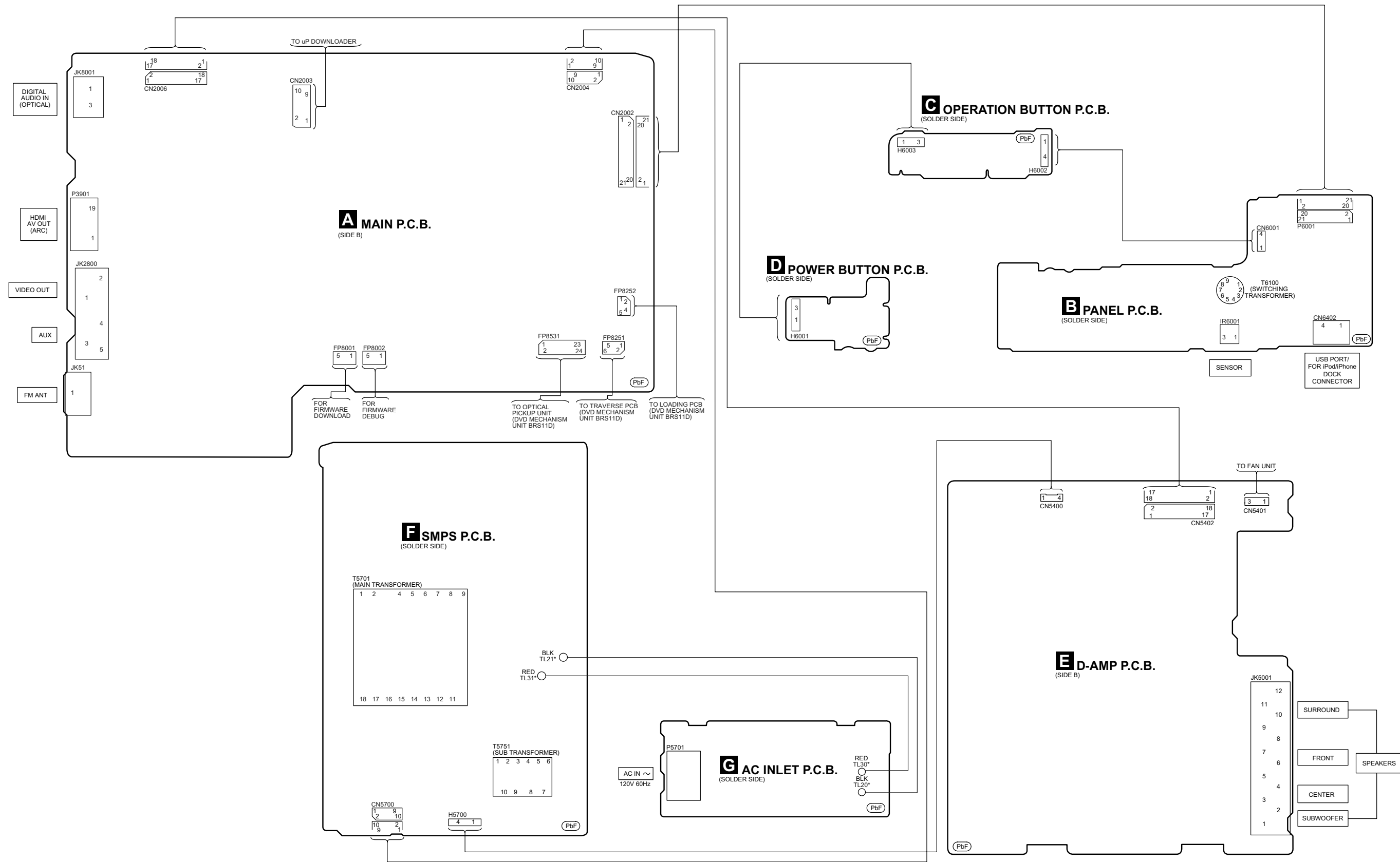
SA-XH170P WIRING CONNECTION DIAGRAM
