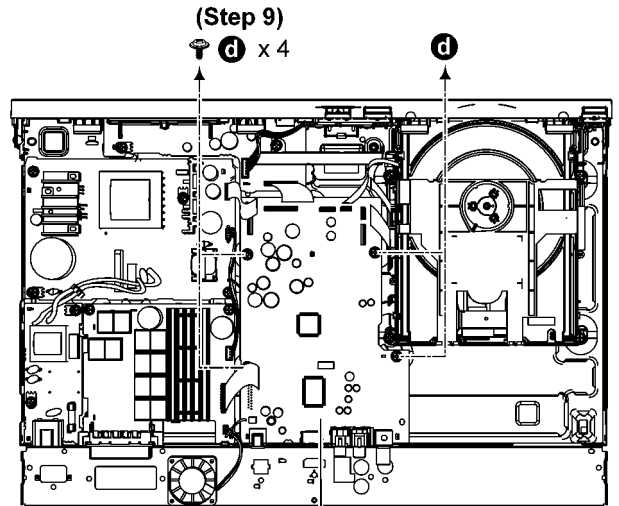
Main P.C.B. (Step 10)
