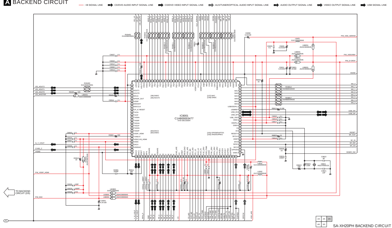
SCHEMATIC DIAGRAM - 3
