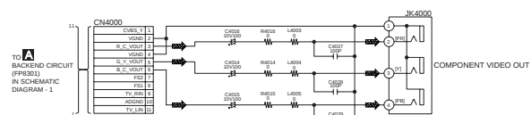
SCHEMATIC DIAGRAM - 17
