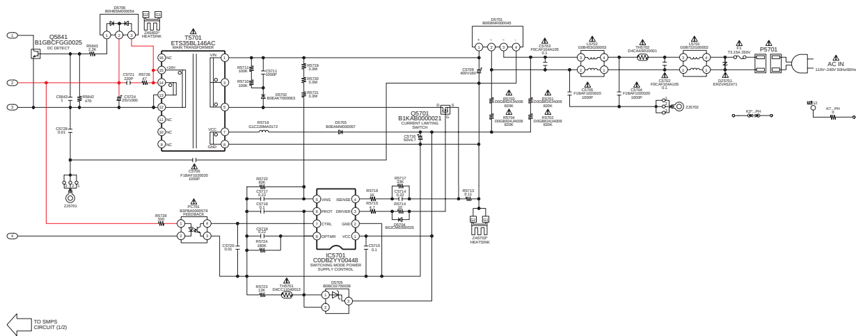
SCHEMATIC DIAGRAM - 16
