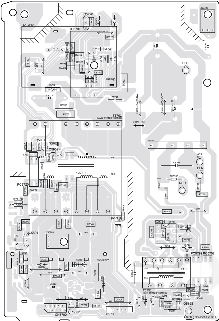
F SMPS P.C.B. (REP4761B...GS/GW) (REP4761C...PH) (REP4761F...GA)
