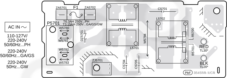
G AC INLET P.C.B. (REP4761B...GS/GW) (REP4761C...PH) (REP4761F...GA)
