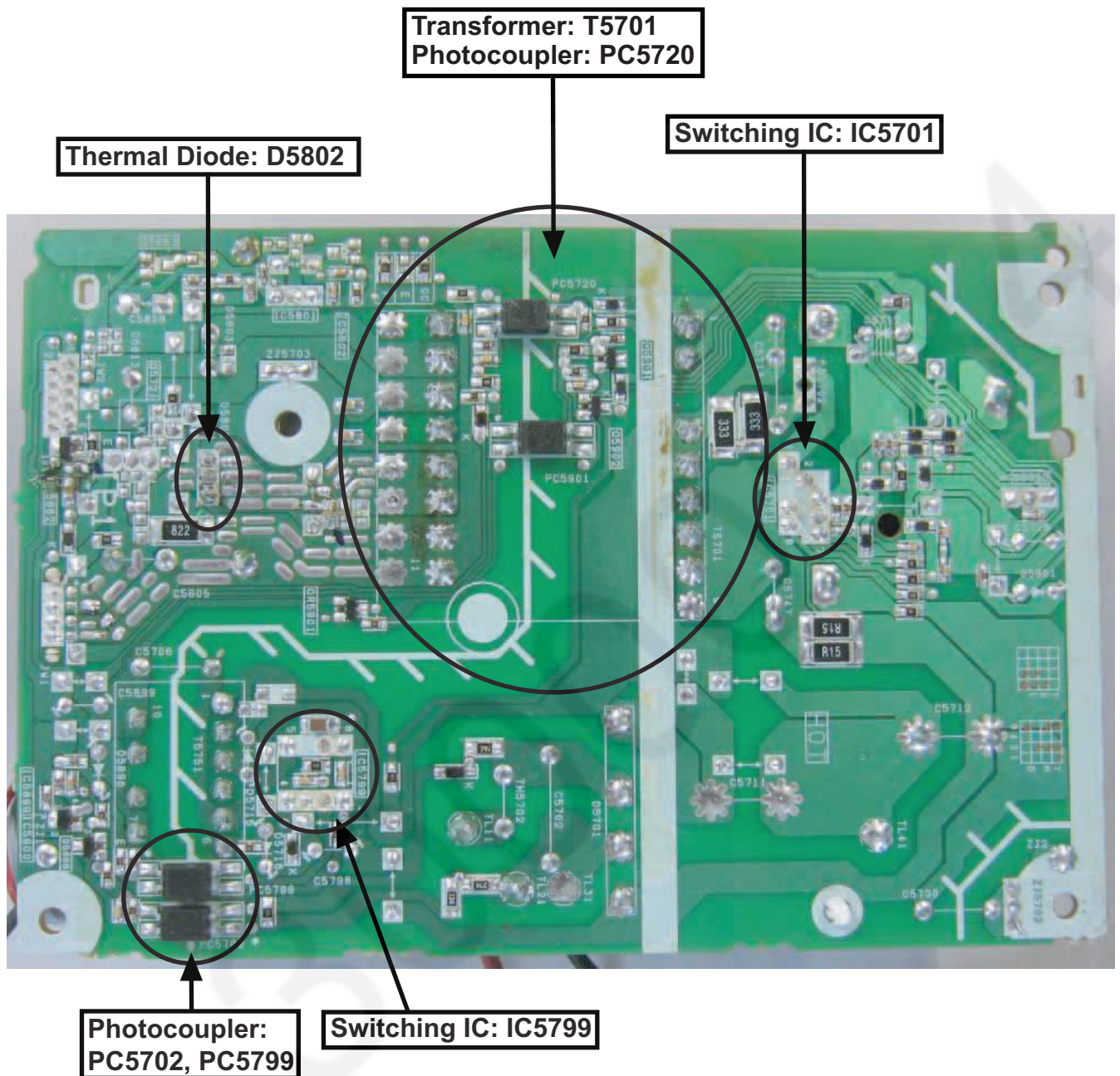
Figure 10-1 SMPS P.C.B.
