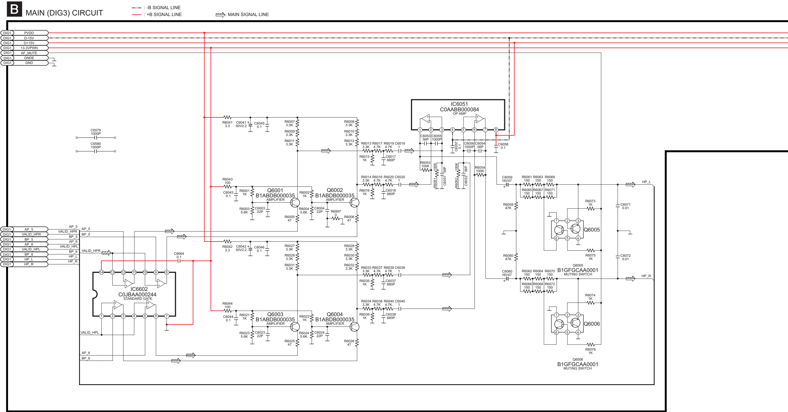
SA-XR57E/EB/EG MAIN (DIG3) CIRCUIT
