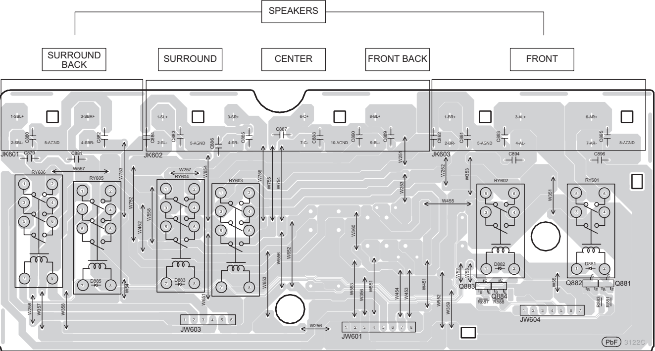
F SPEAKER P.C.B (REP4029C-P)
