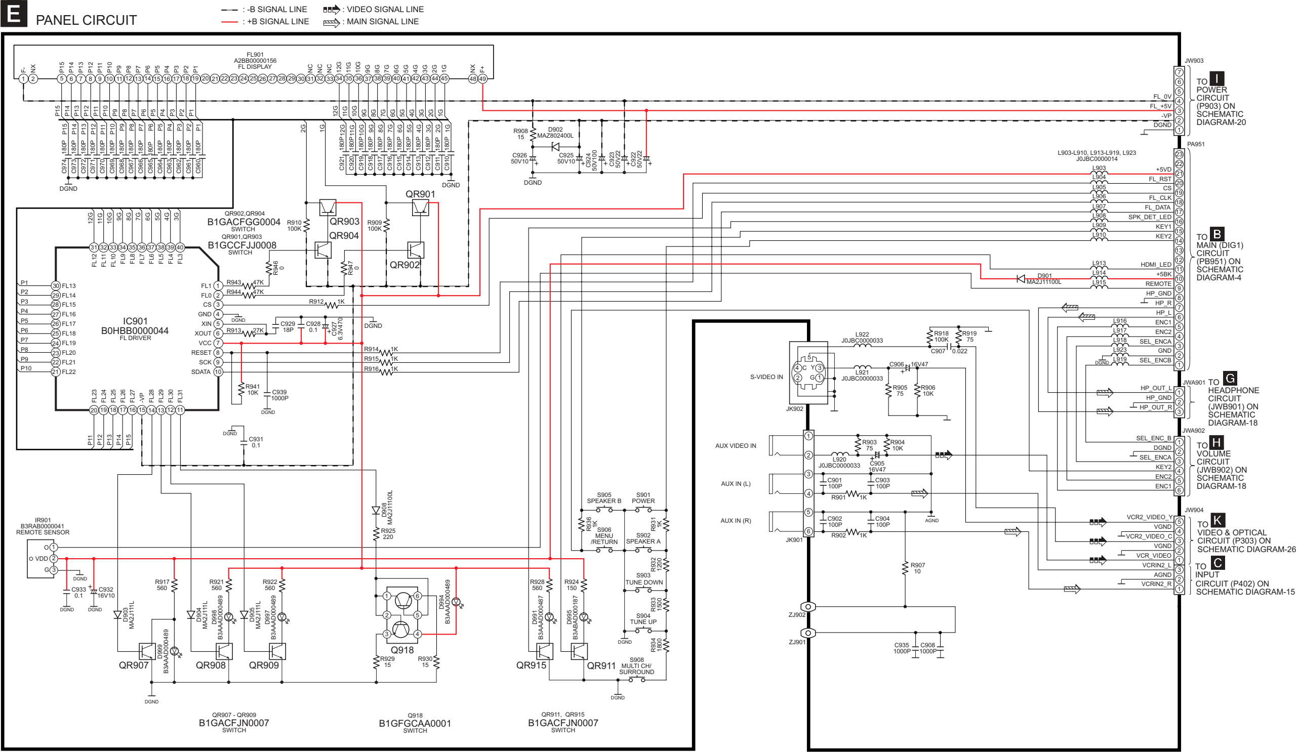
SA-XR57E/EB/EG PANEL CIRCUIT
