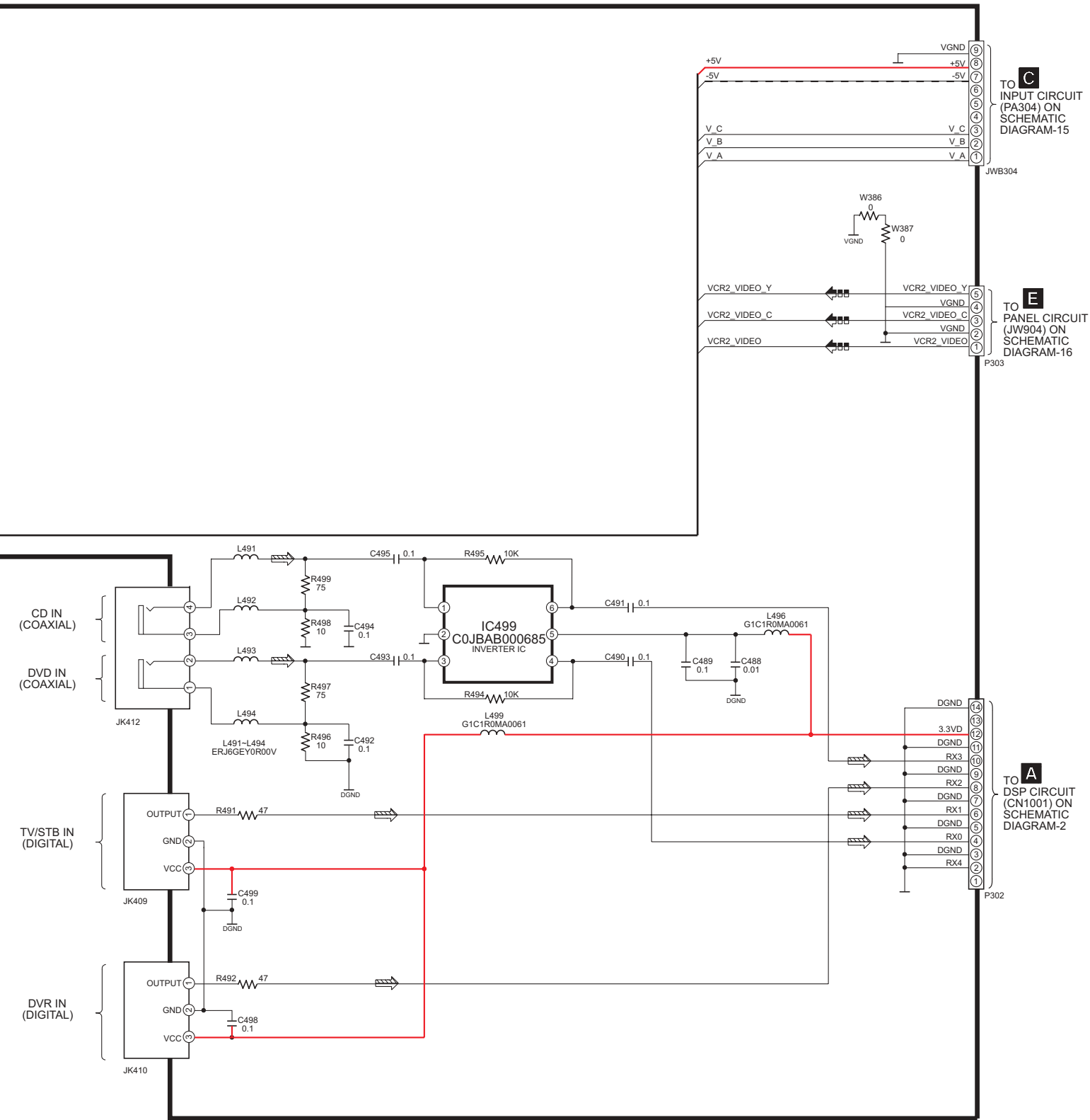
SA-XR57E/EB/EG VIDEO & OPTICAL CIRCUIT
