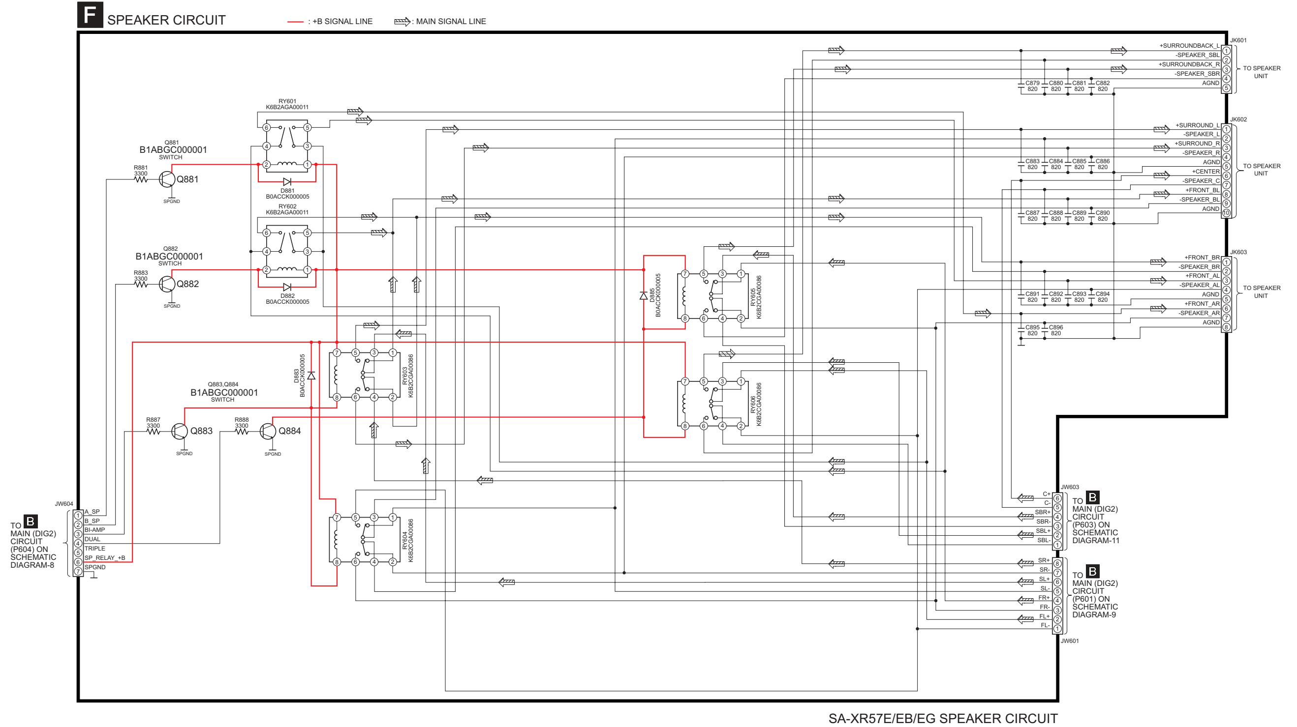
SCHEMATIC DIAGRAM - 17
