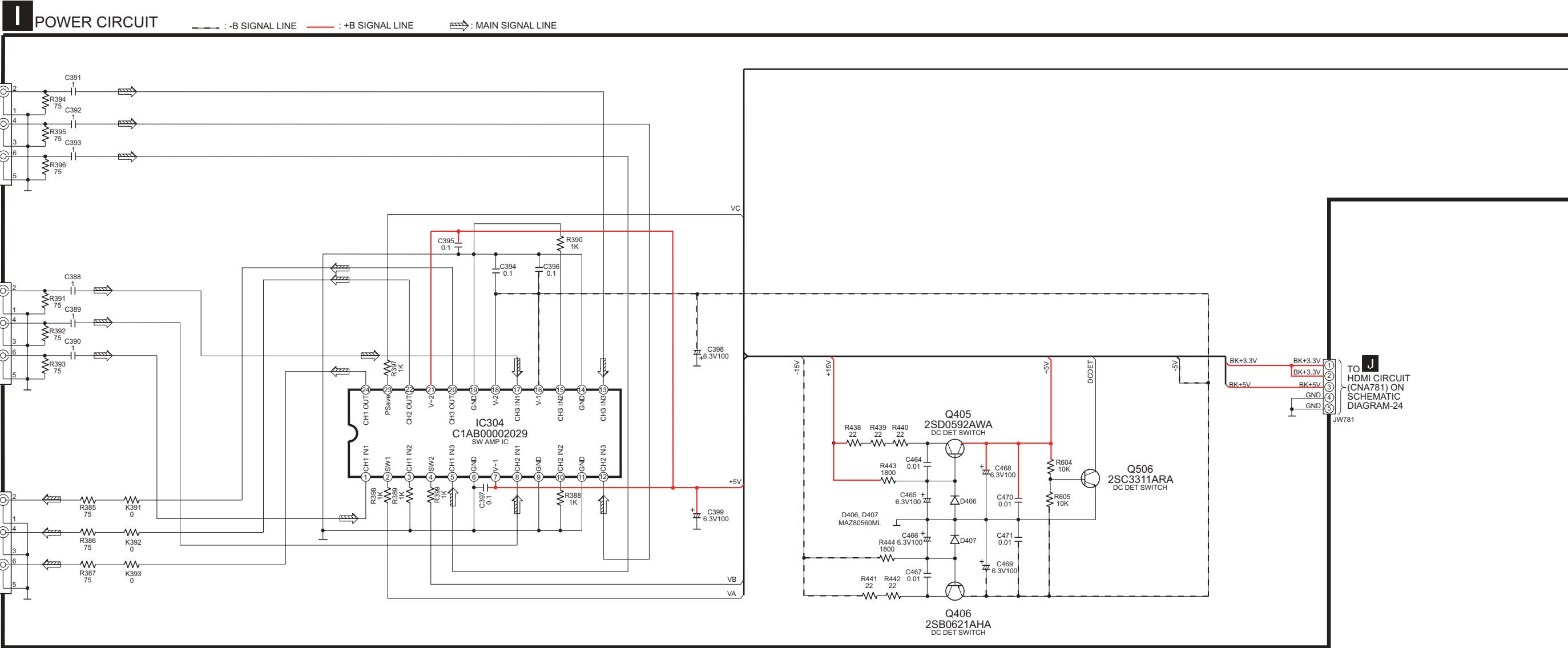
SA-XR57E/EB/EG HEADPHONE / VOLUME / POWER CIRCUIT
