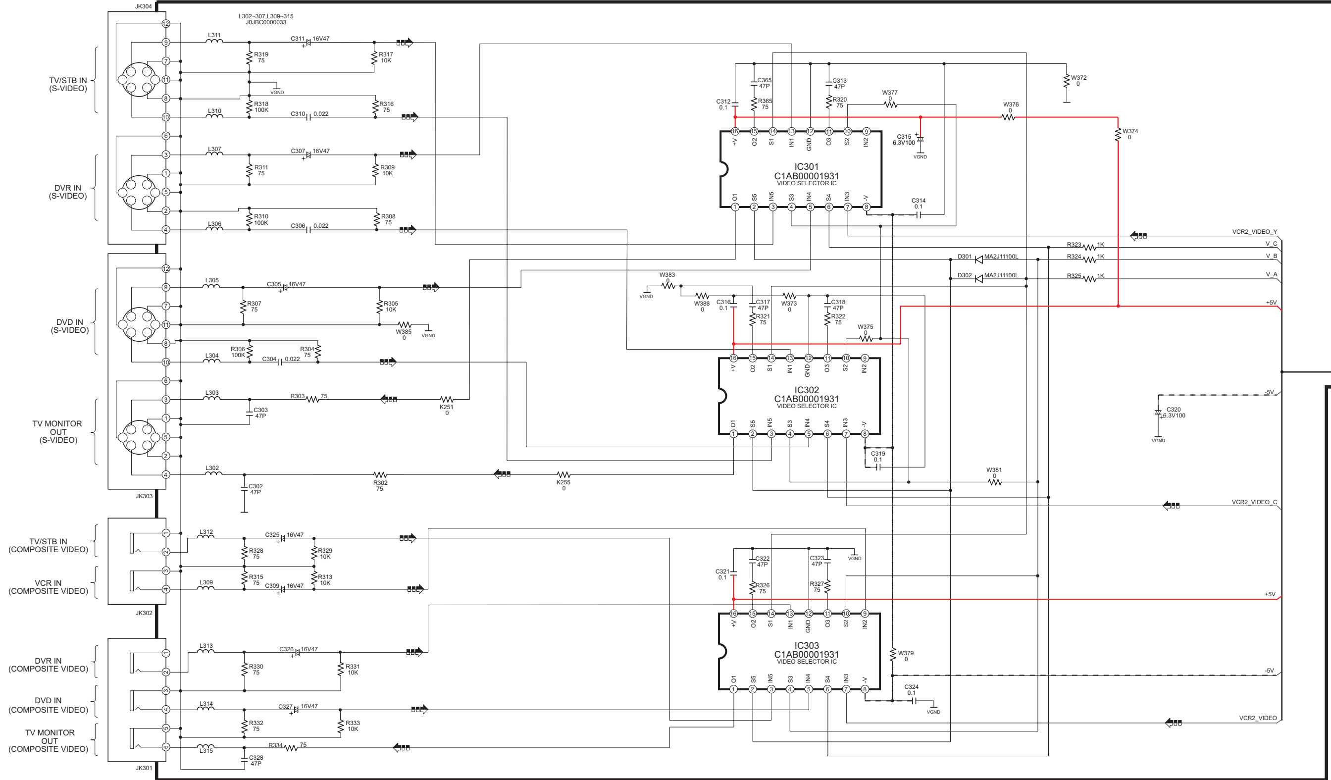
SCHEMATIC DIAGRAM - 25
