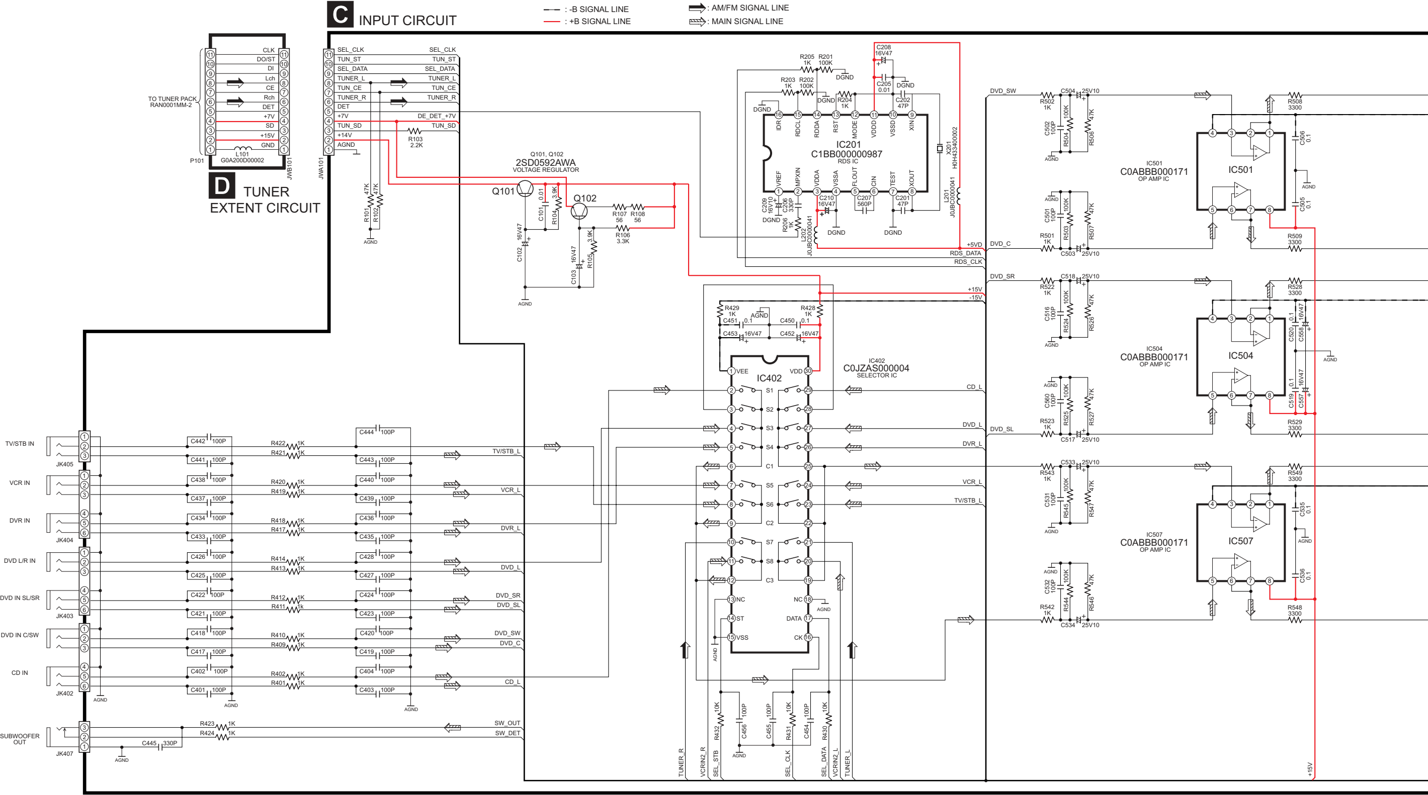
SCHEMATIC DIAGRAM - 14
