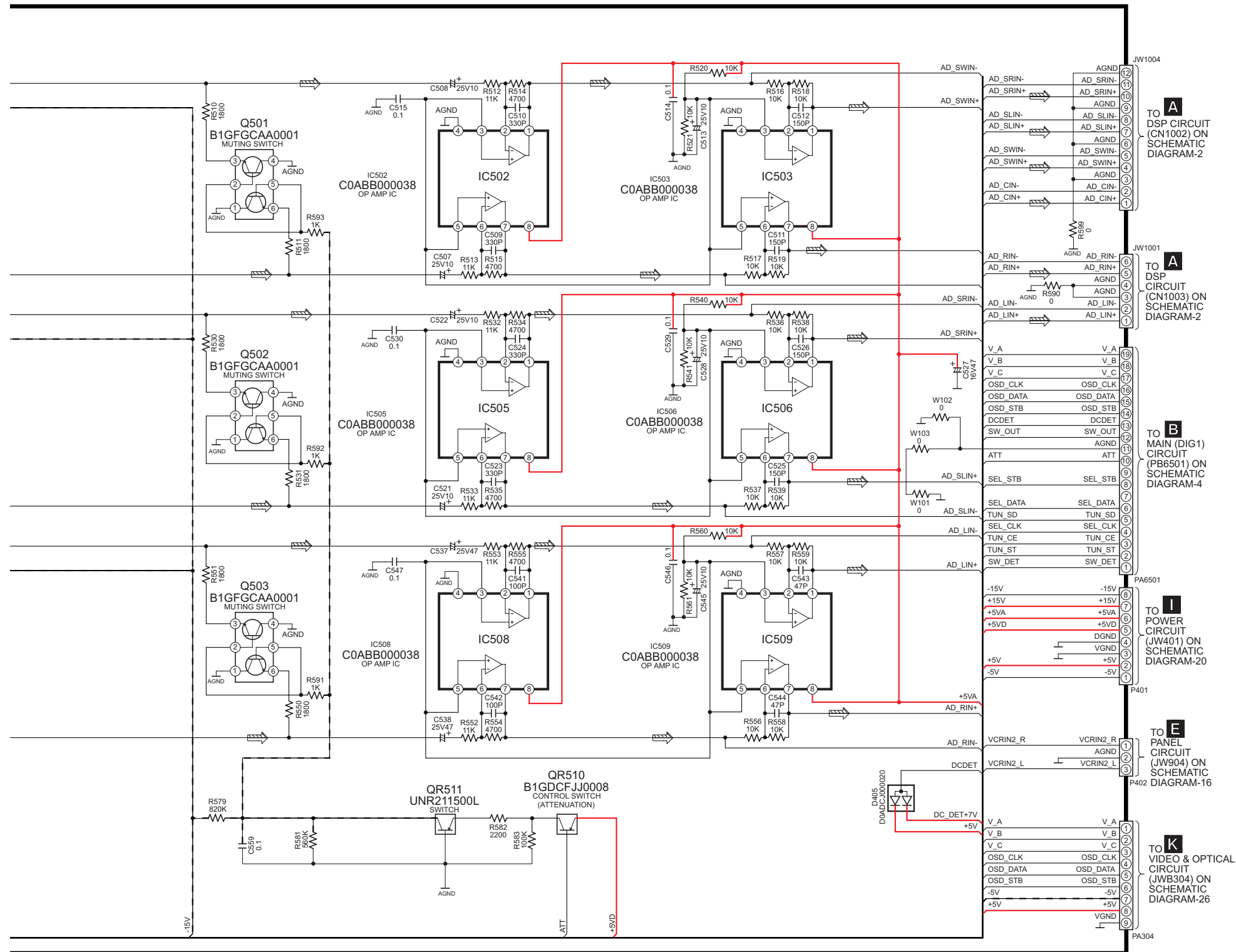
SCHEMATIC DIAGRAM - 15
