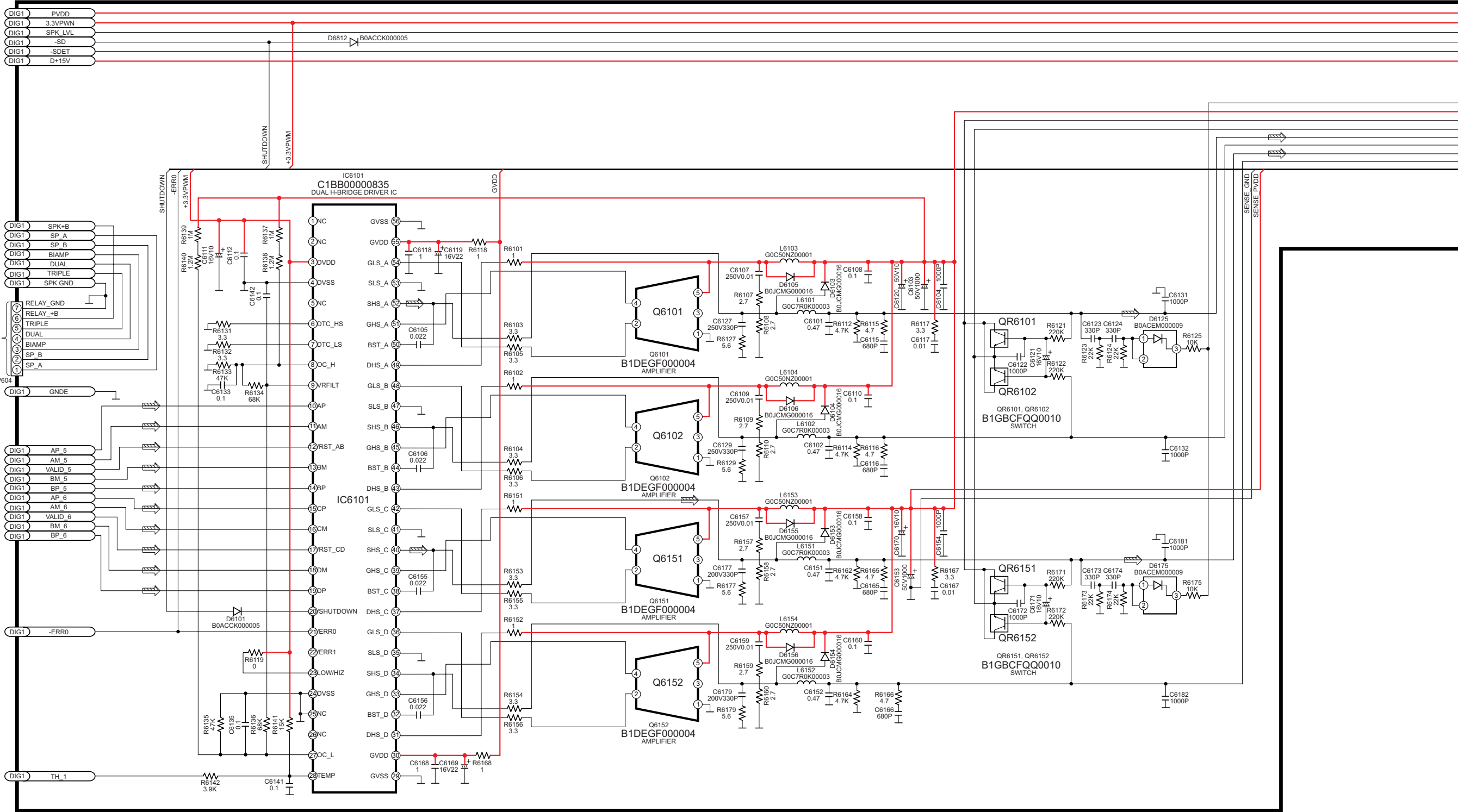
SA-XR57E/EB/EG MAIN (DIG 2) CIRCUIT
