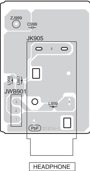
G HEADPHONE P.C.B (REP4027D-S)
