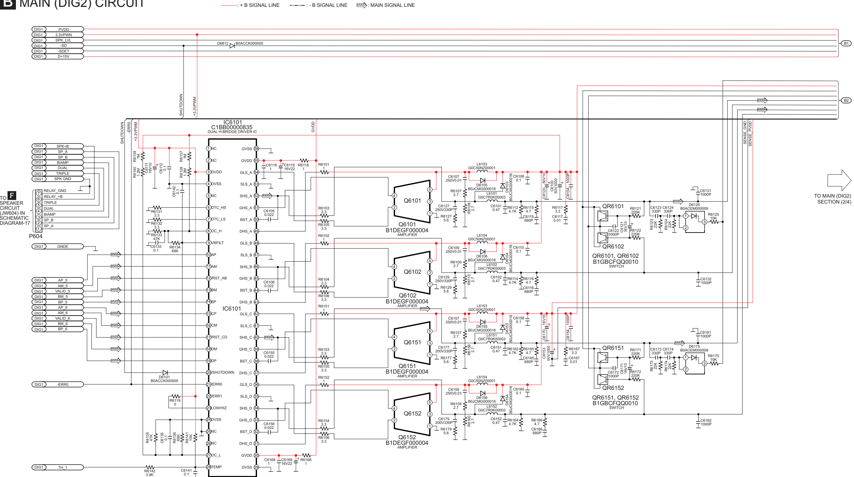
SCHEMATIC DIAGRAM - 8
