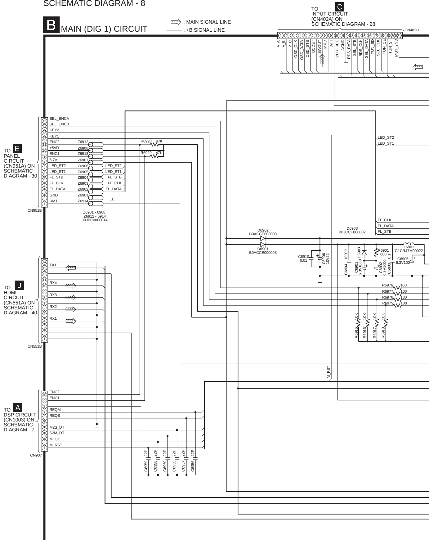
SCHEMATIC DIAGRAM - 8
