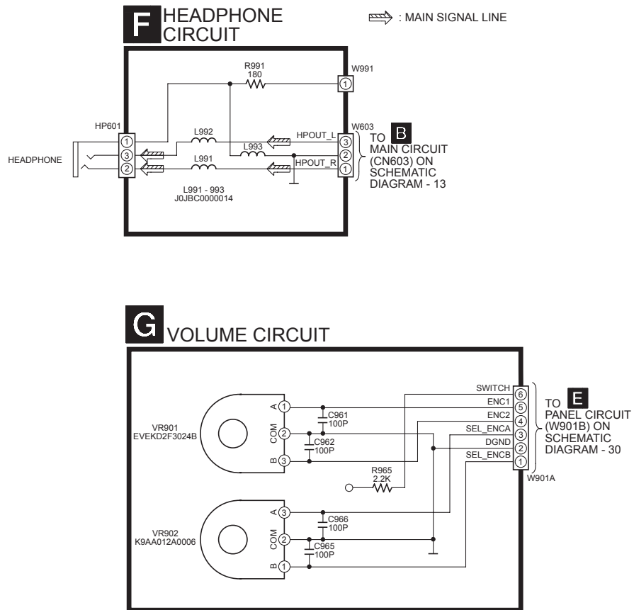
SCHEMATIC DIAGRAM - 31
