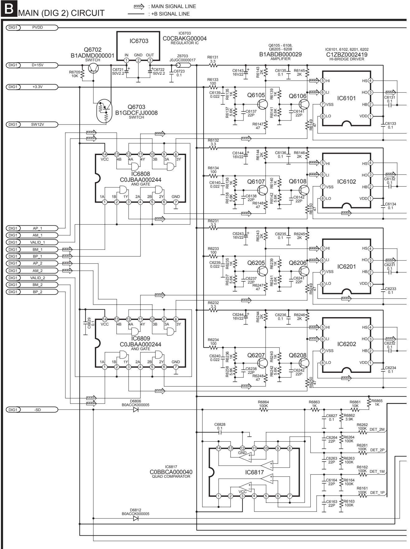
SCHEMATIC DIAGRAM - 15
