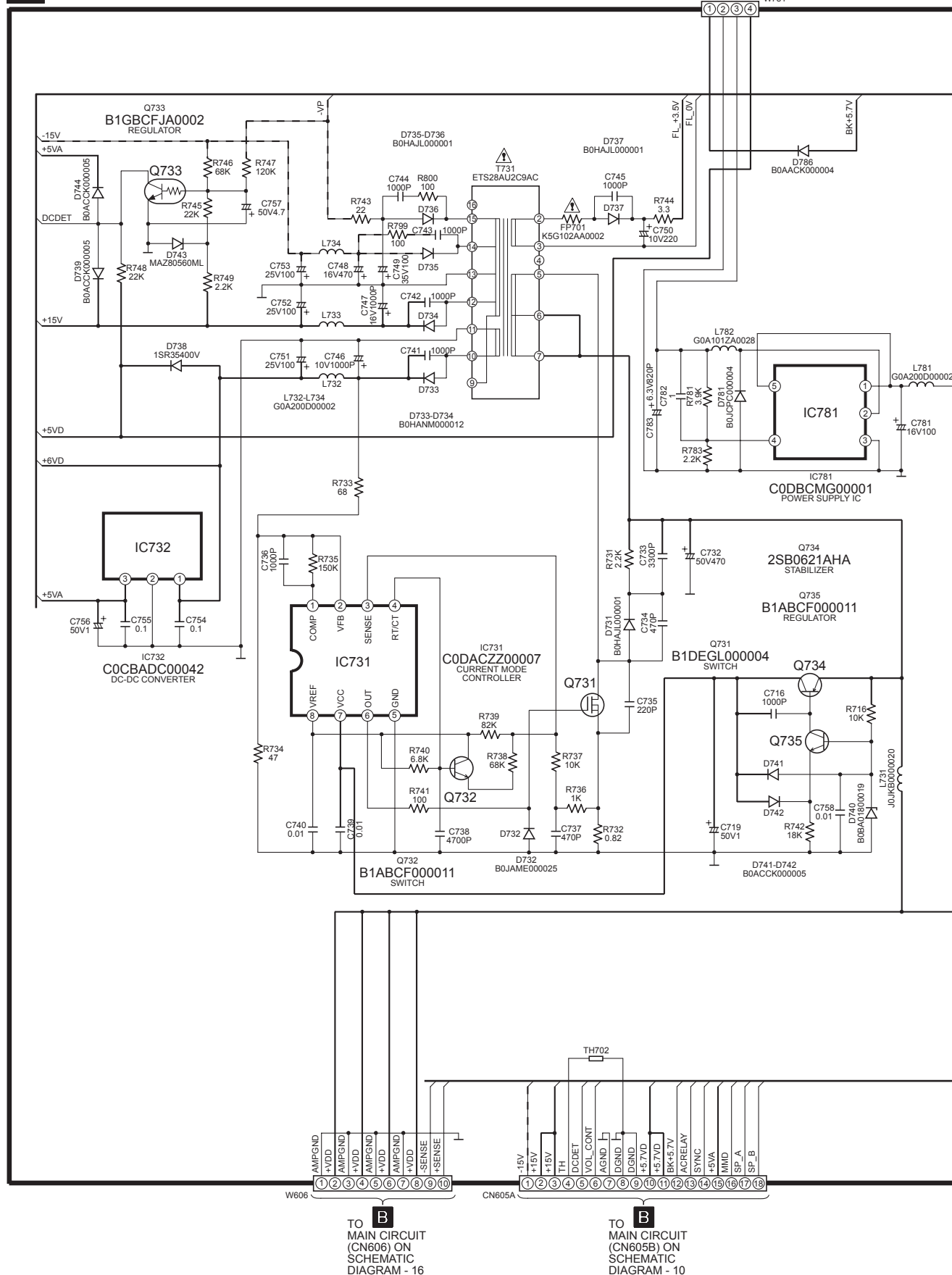
SCHEMATIC DIAGRAM - 32
