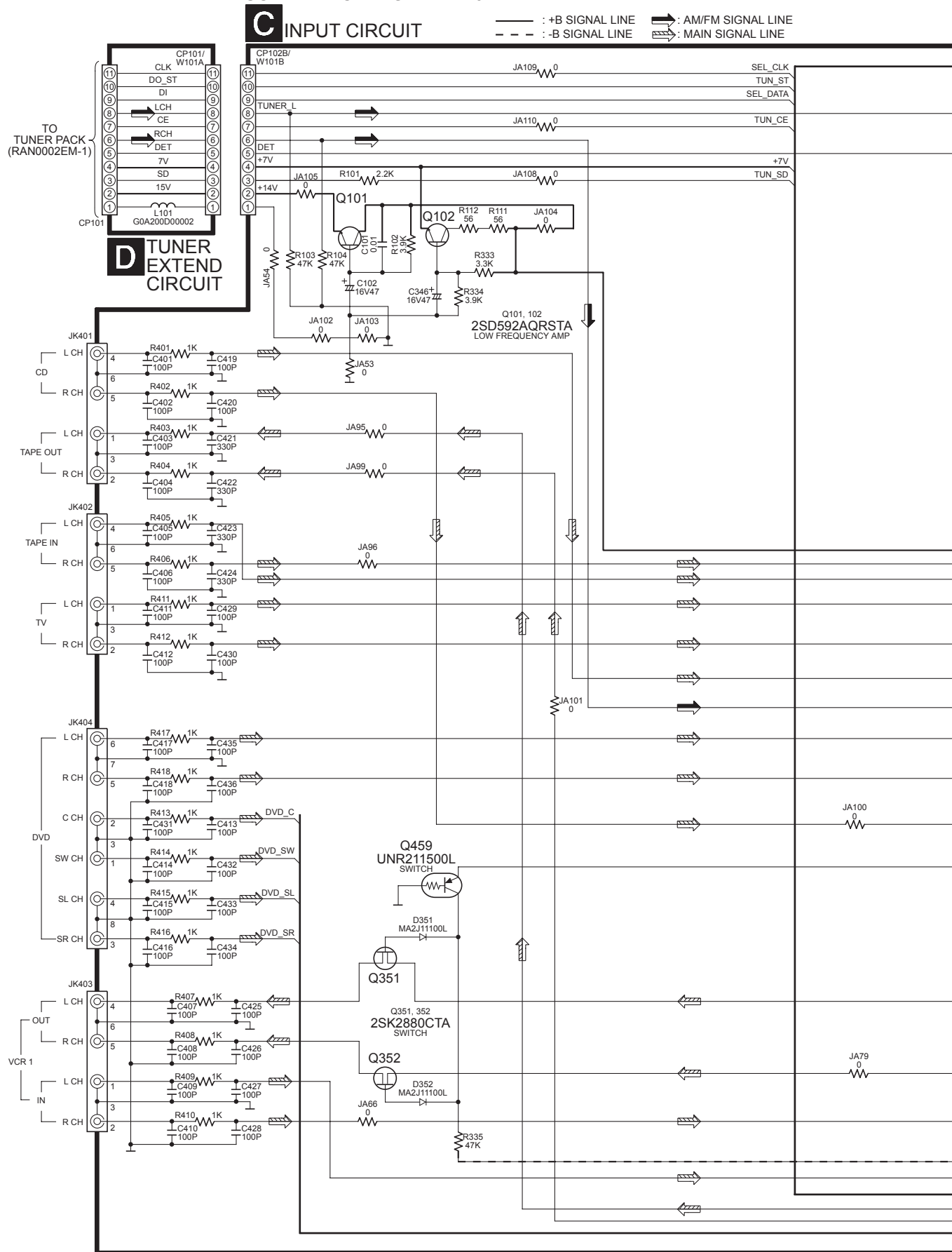
SCHEMATIC DIAGRAM - 20
