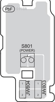
G POWER SWITCH P.C.B (REPV0116B)
