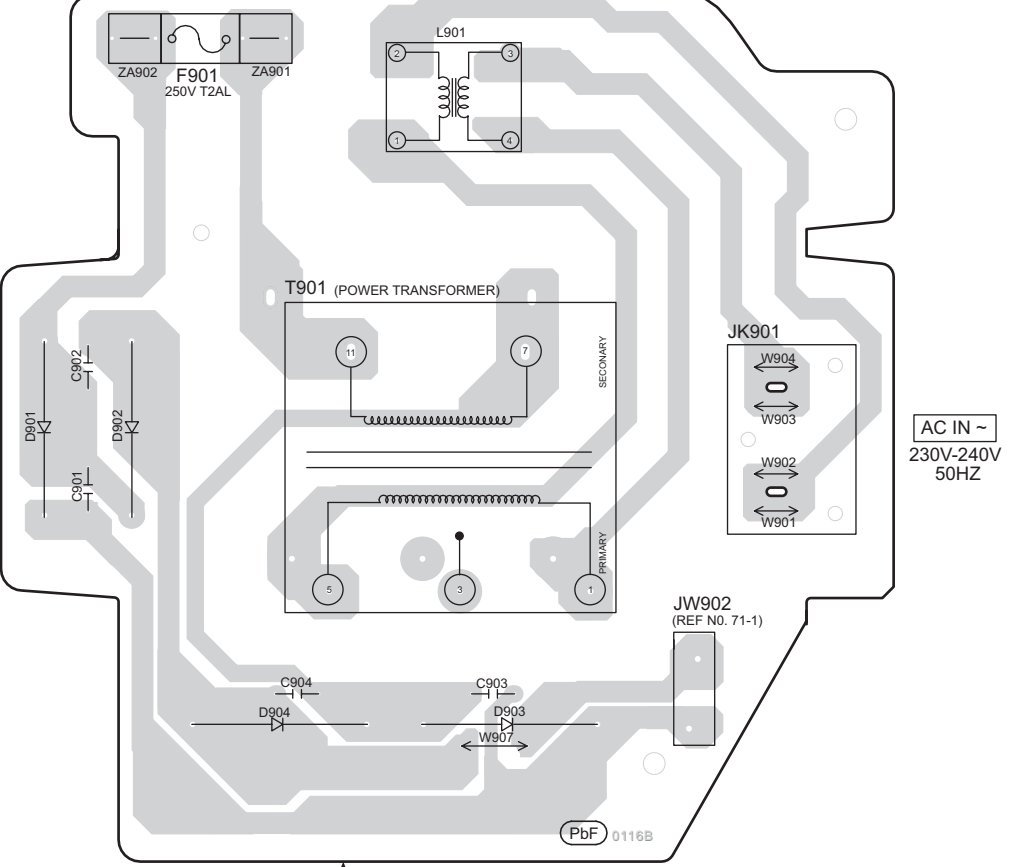
L TRANSFORMER P.C.B (REPV0116B)
