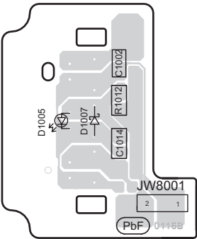
F LED P.C.B (REPV0116B)
