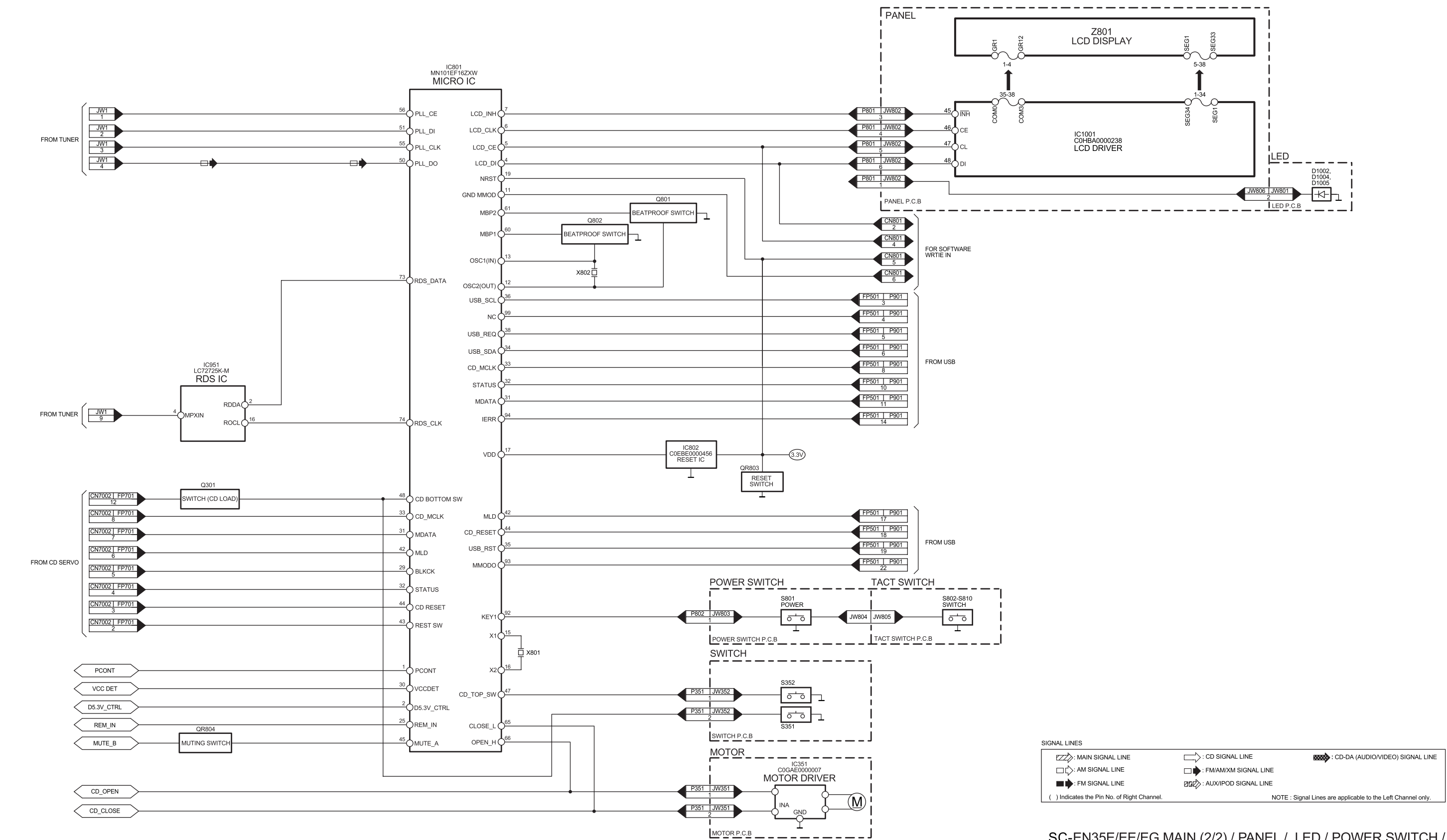
SC-EN35E/EE/EG MAIN (2/2) / PANEL / LED / POWER SWITCH / TACT SWITCH / SWITCH / MOTOR BLOCK DIAGRAM
