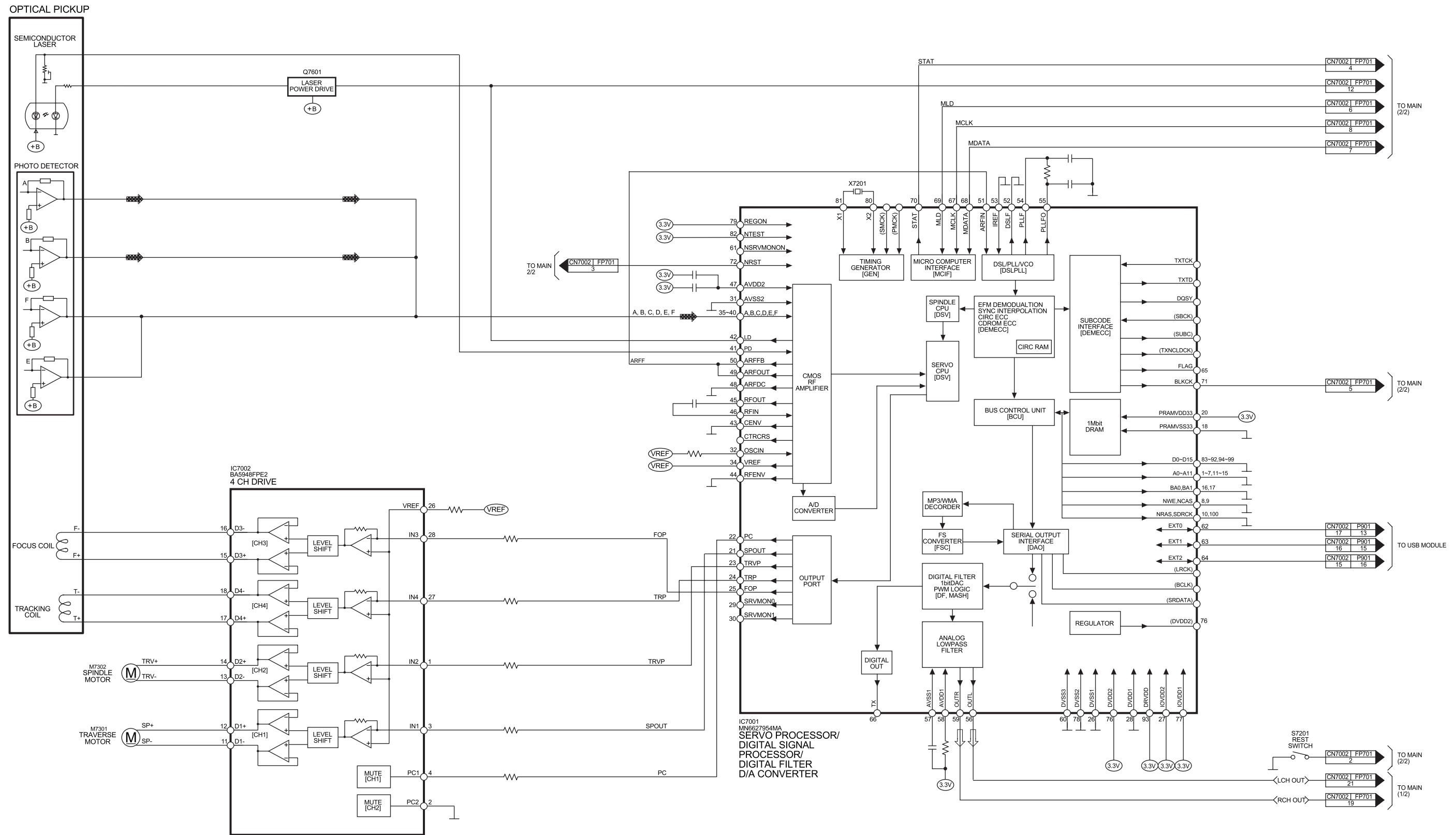
SC-EN35E/EE/EG CD SERVO BLOCK DIAGRAM
