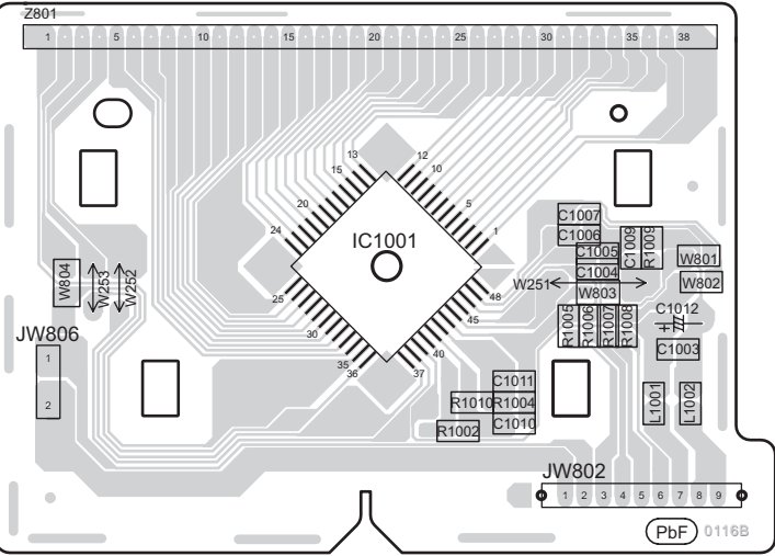
E PANEL P.C.B (REPV0116B)
