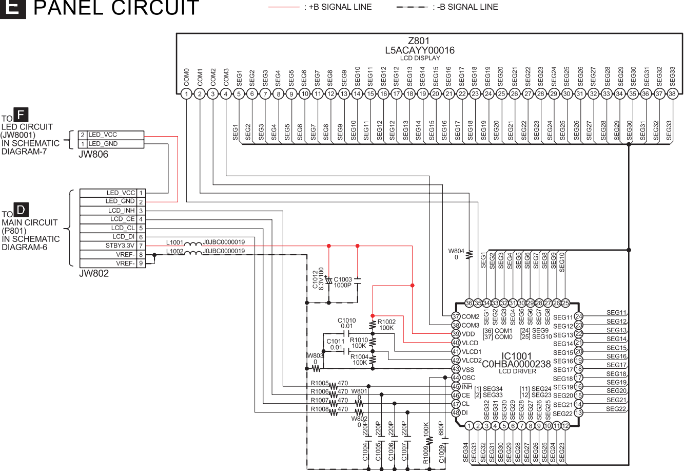
SCHEMATIC DIAGRAM - 7
