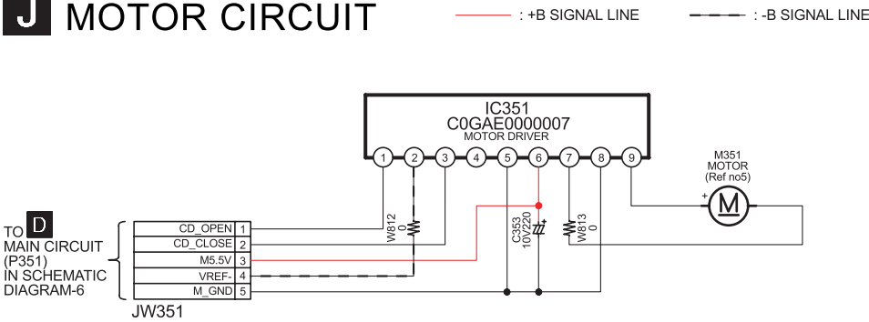
SCHEMATIC DIAGRAM - 8
