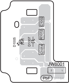
F LED P.C.B (REPV0116A)
