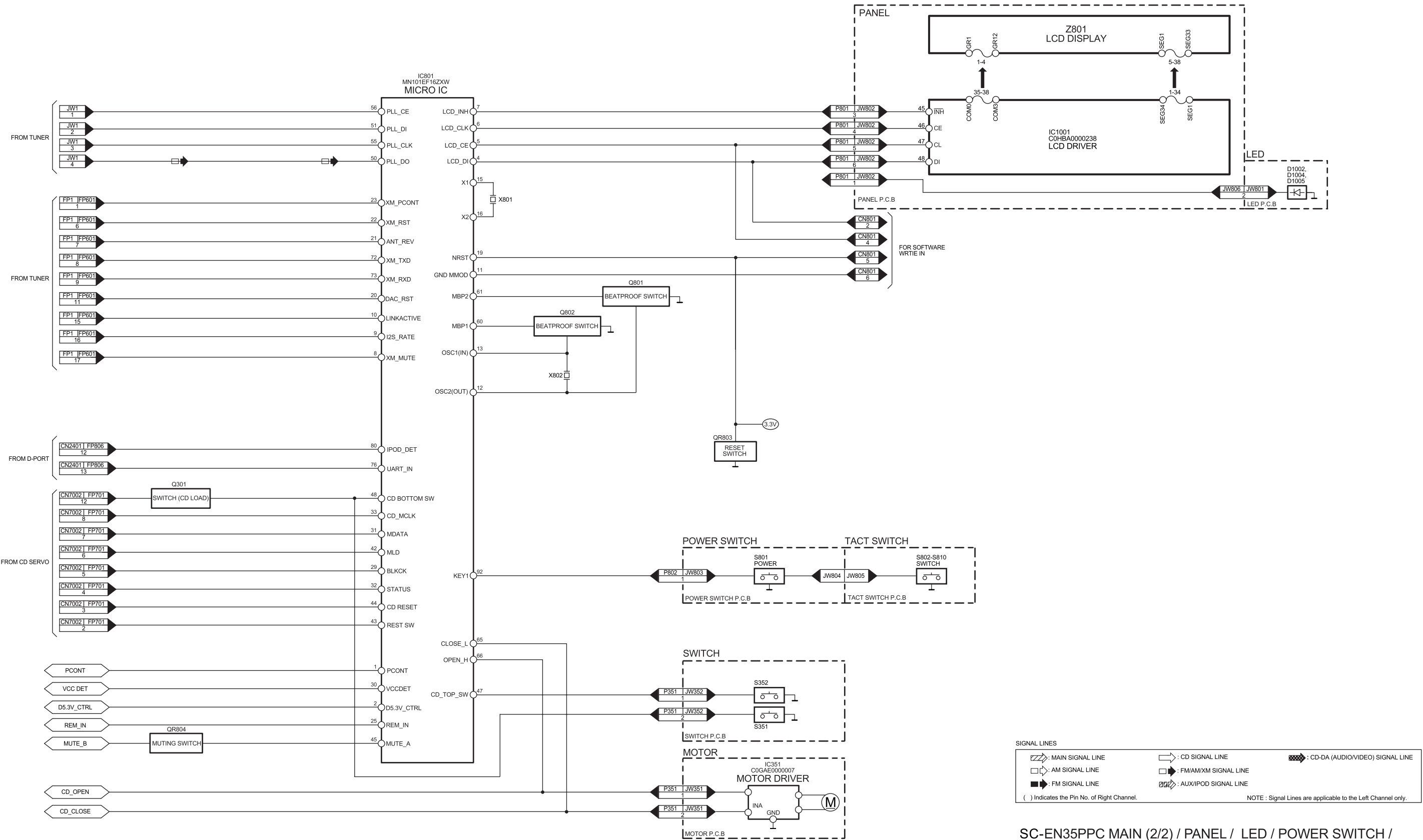
SC-EN35PPC MAIN (2/2) / PANEL / LED / POWER SWITCH / TACT SWITCH / SWITCH / MOTOR BLOCK DIAGRAM
