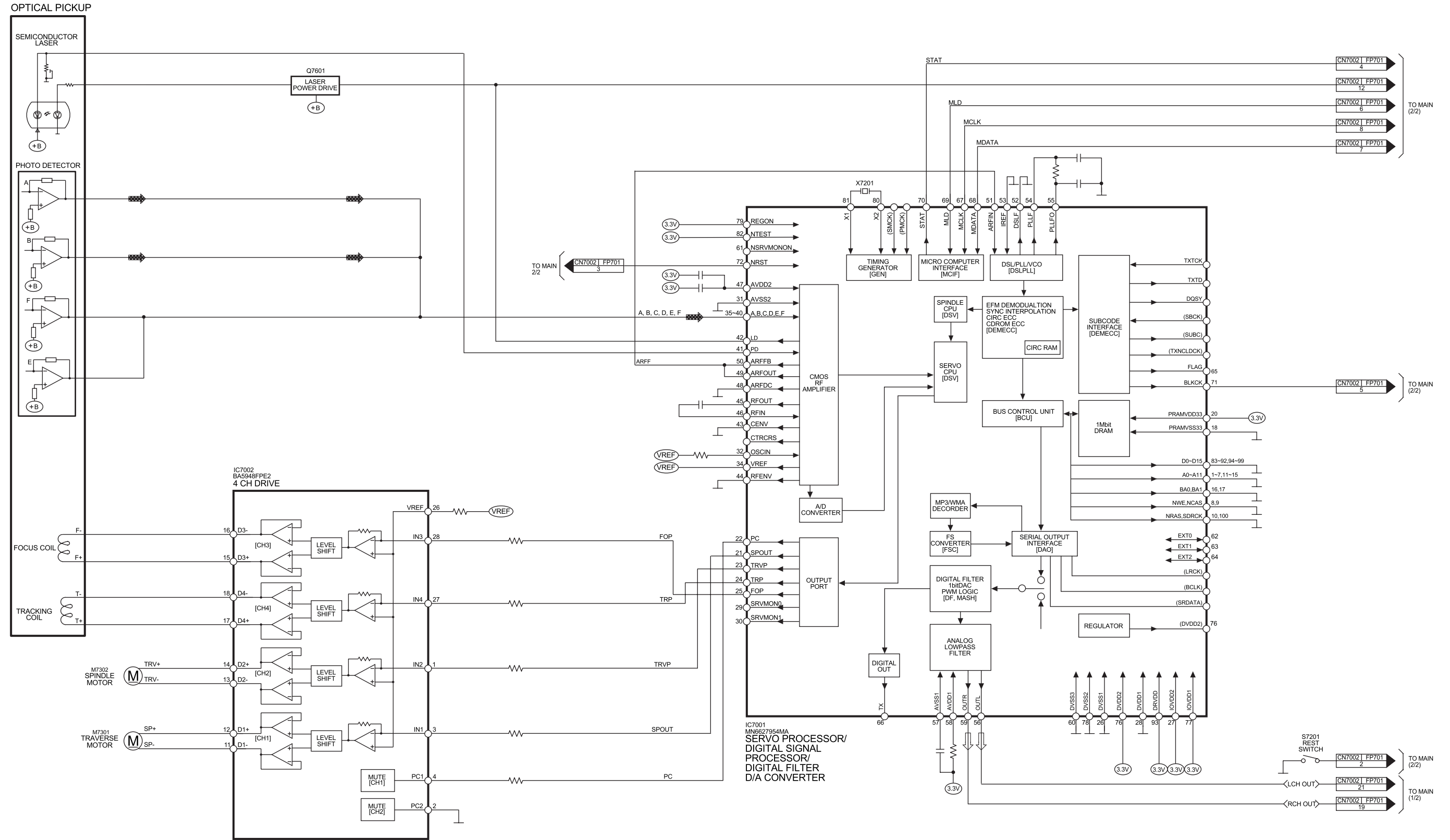
SC-EN35PPC CD SERVO BLOCK DIAGRAM
