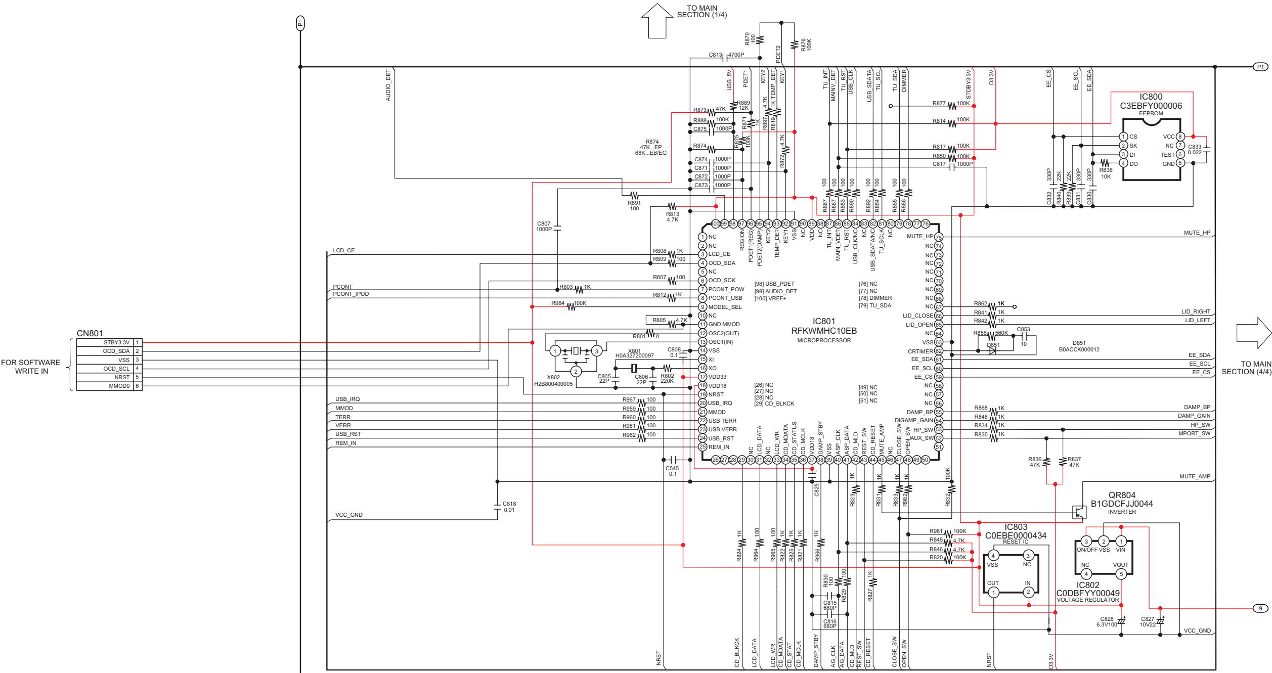
SCHEMATIC DIAGRAM - 4 B MAIN(MICON) CIRCUIT
