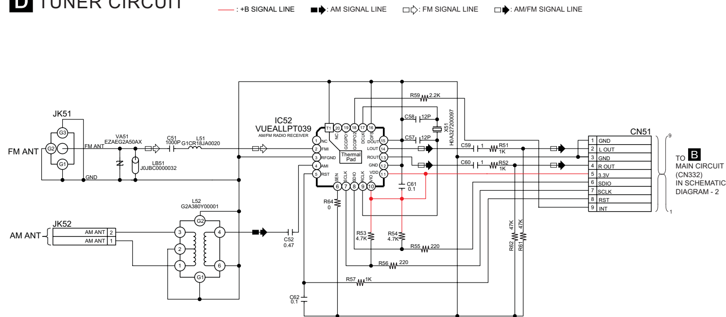
SCHEMATIC DIAGRAM - 8
