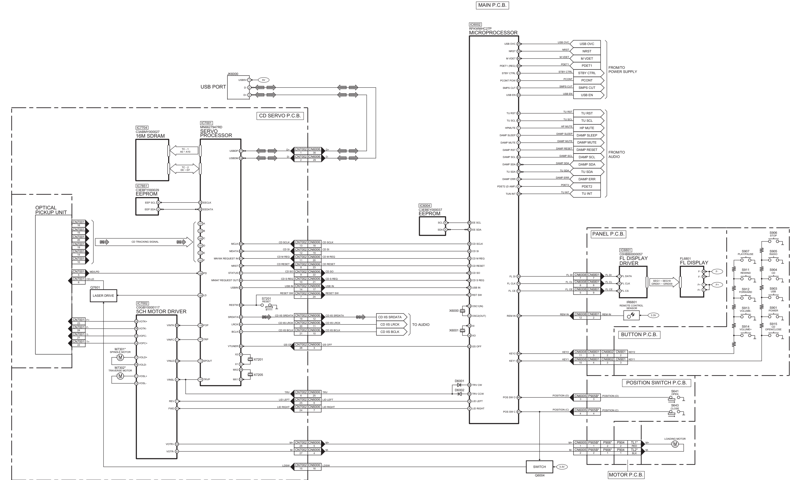
SC-HC17EB/EC/EE/EG SERVO & SYSTEM CONTROL BLOCK DIAGRAM
