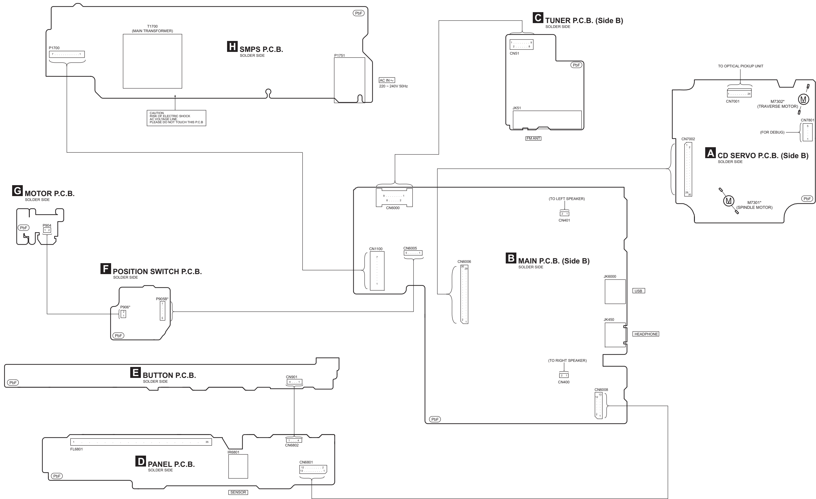
SC-HC17EB/EC/EE/EG WIRING CONNECTION DIAGRAM
