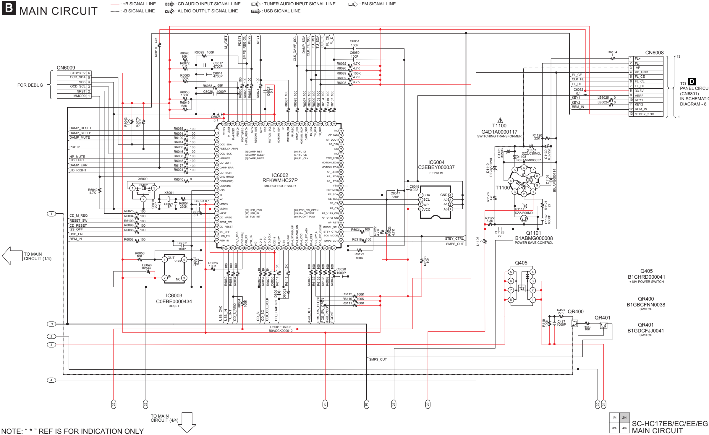
SCHEMATIC DIAGRAM - 4
