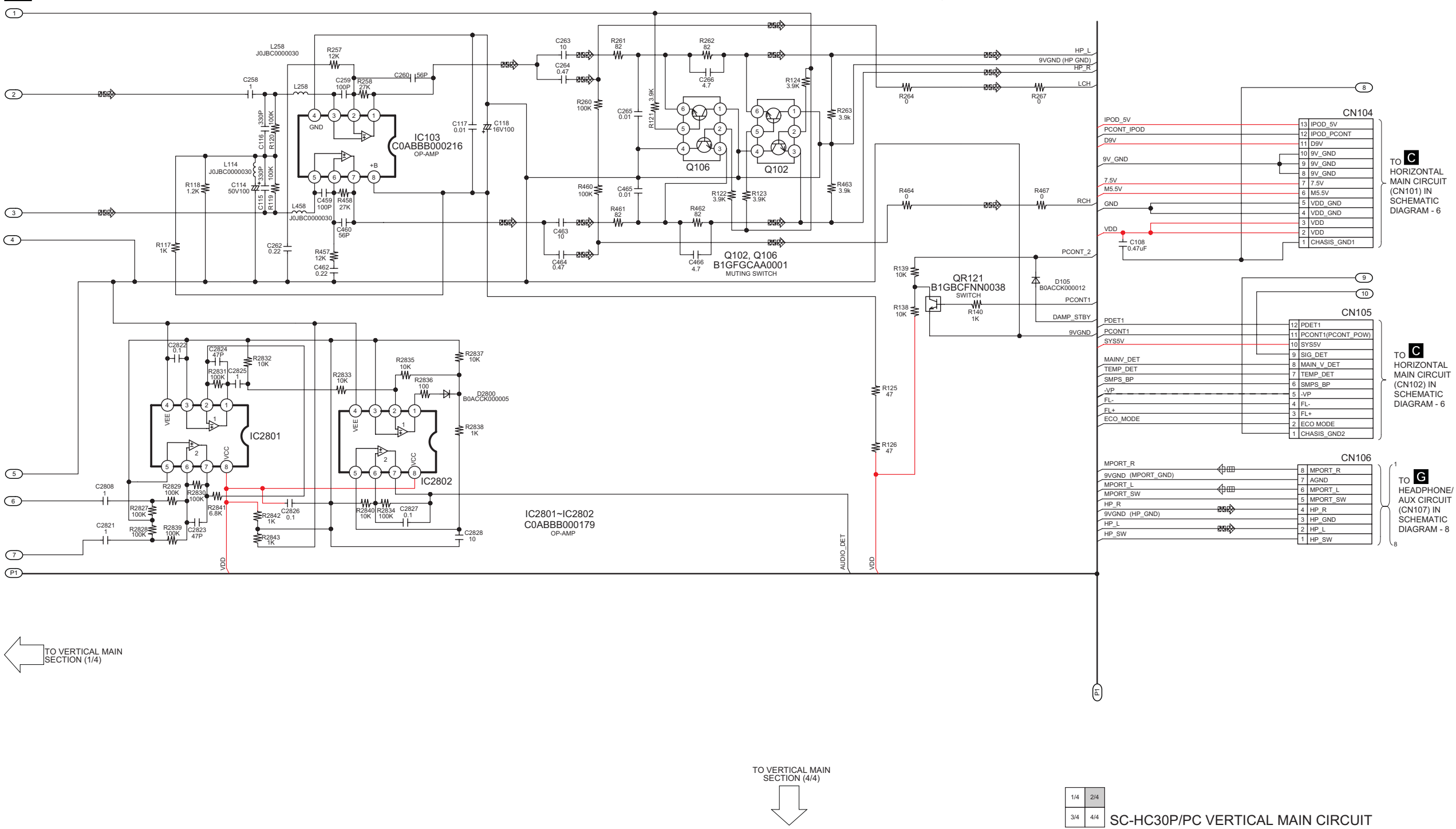
SCHEMATIC DIAGRAM - 3
