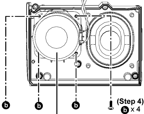
Front Speaker (SP1) (Step 5)
