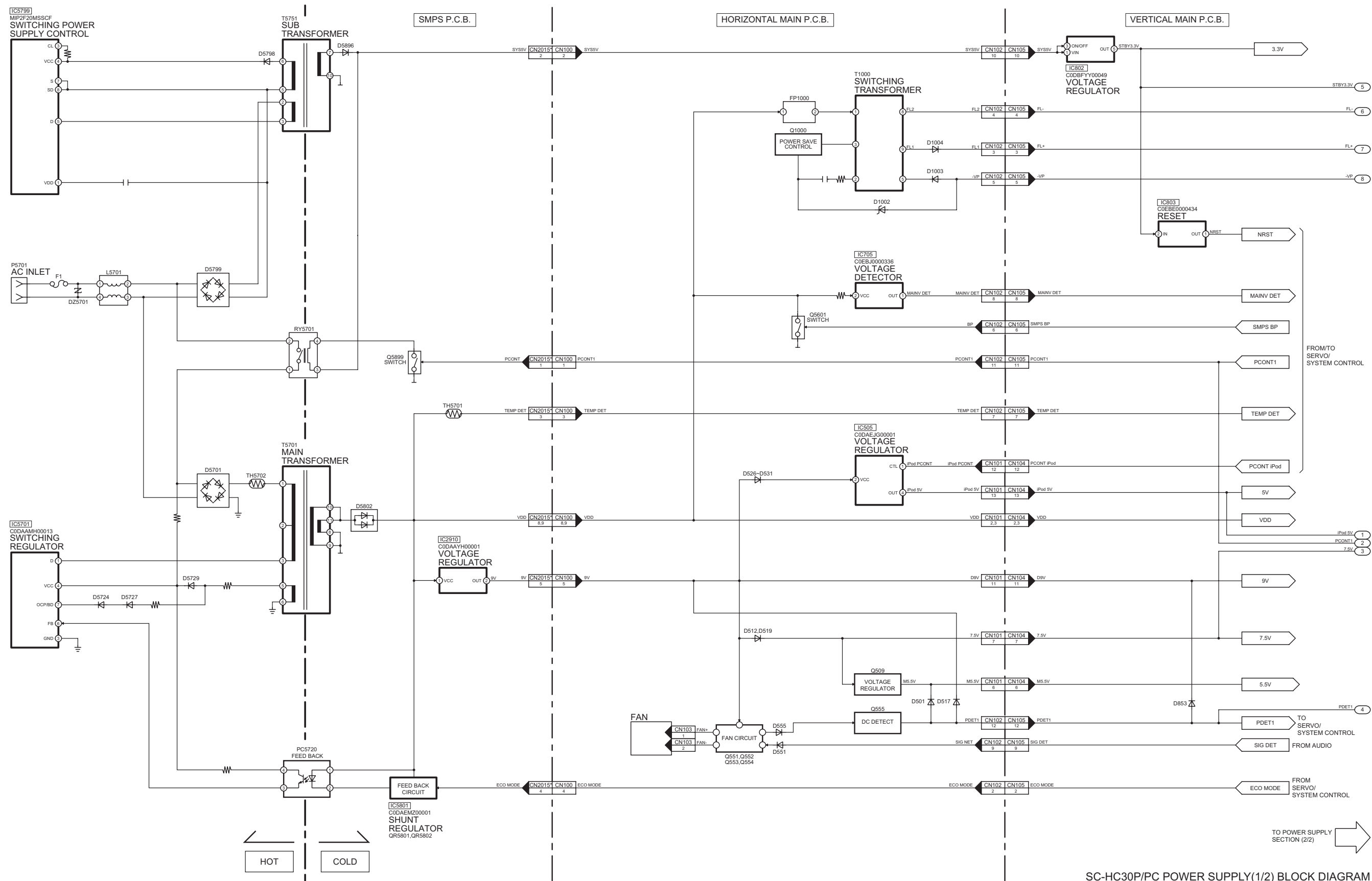
SC-HC30P/PC POWER SUPPLY(1/2) BLOCK DIAGRAM
