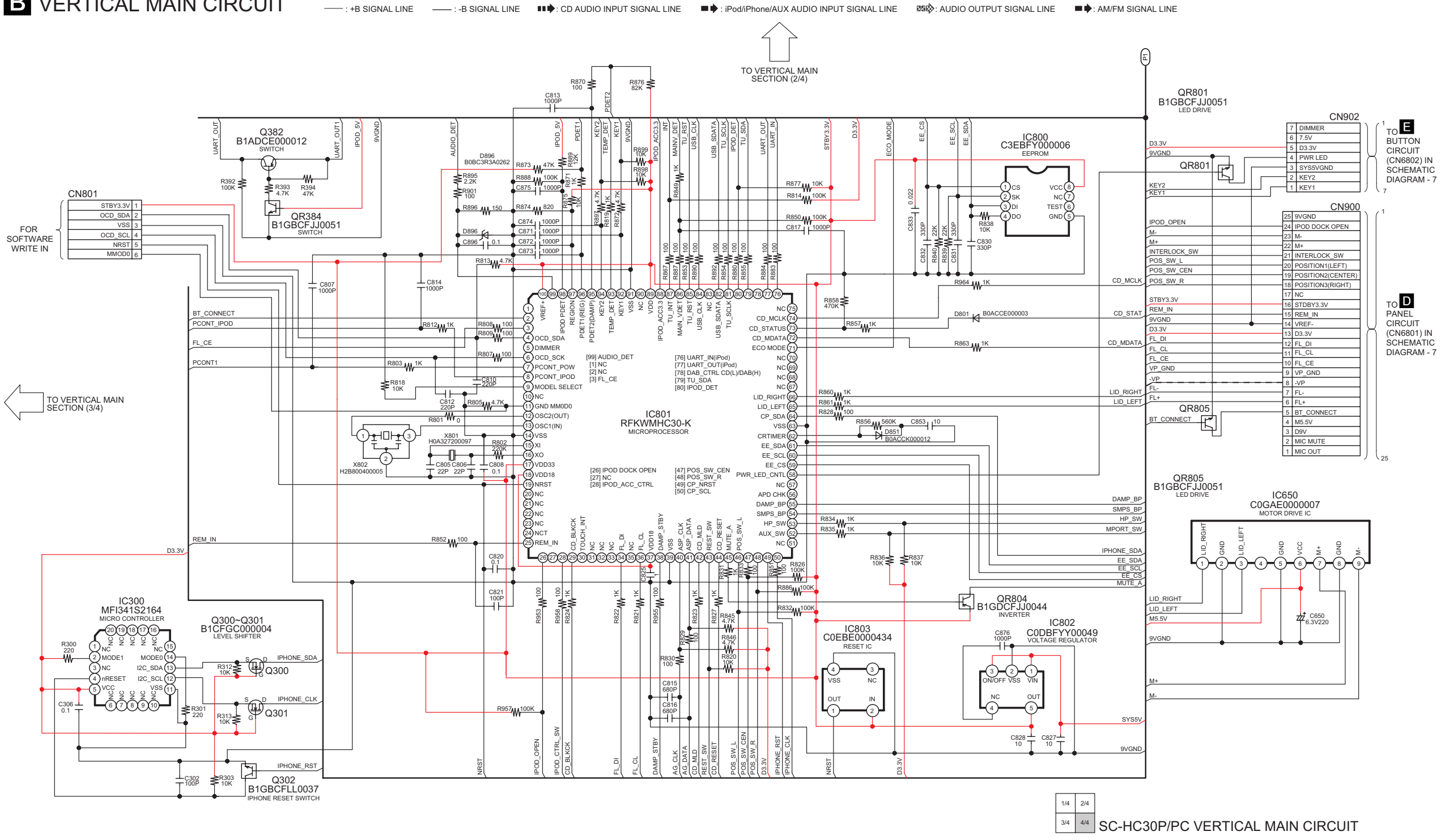
SCHEMATIC DIAGRAM - 5
