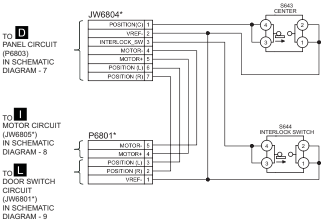
SC-HC30P/PC iPod/iPhone / iPod/iPhone SWITCH / DOOR SWITCH / INTERLOCK SWITCH CIRCUIT
