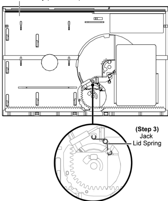
Door Assembly (Back View)
