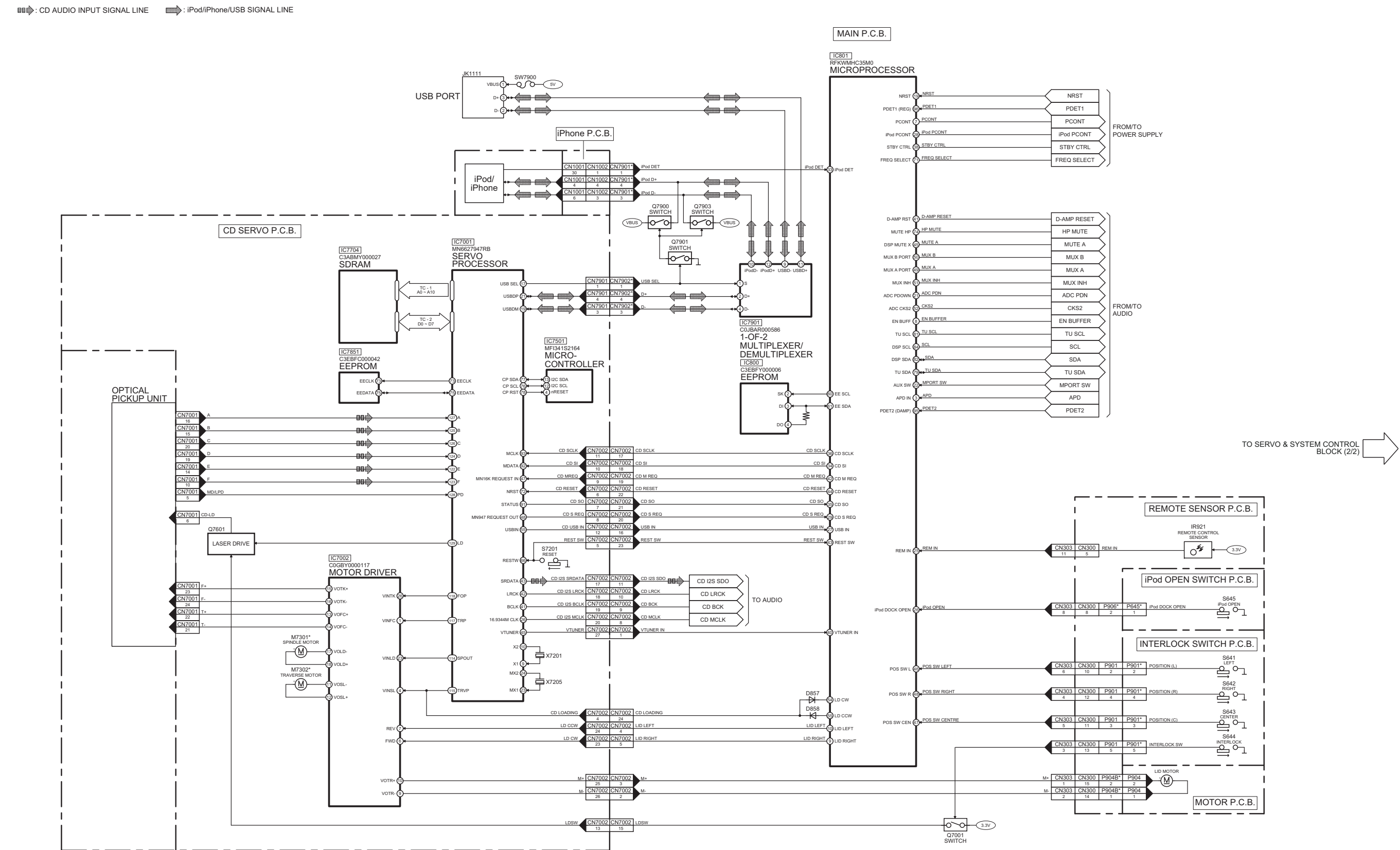
SC-HC35EF/EG/EP SERVO & SYSTEM CONTROL (1/2) BLOCK DIAGRAM
