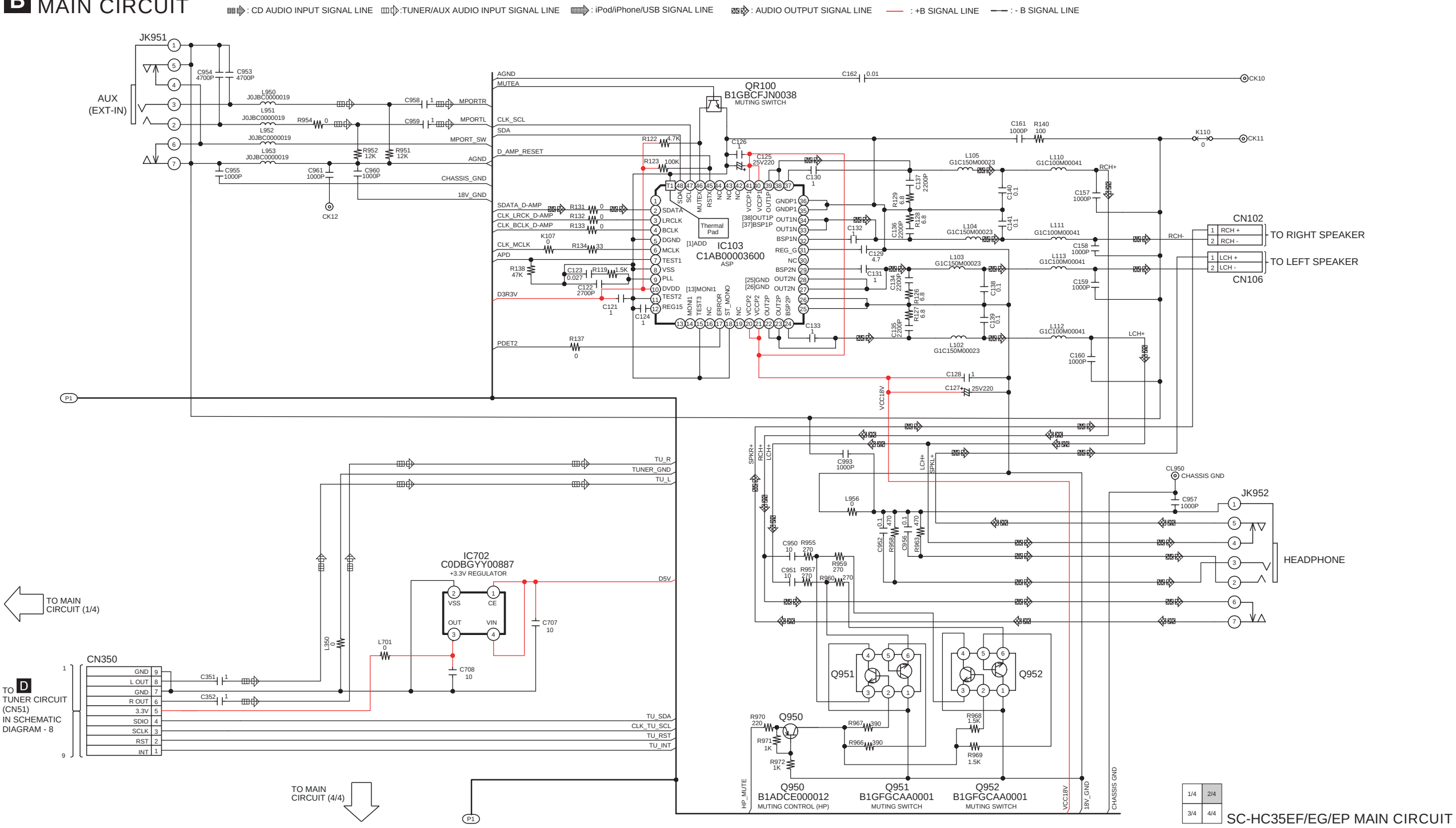
SCHEMATIC DIAGRAM - 4
