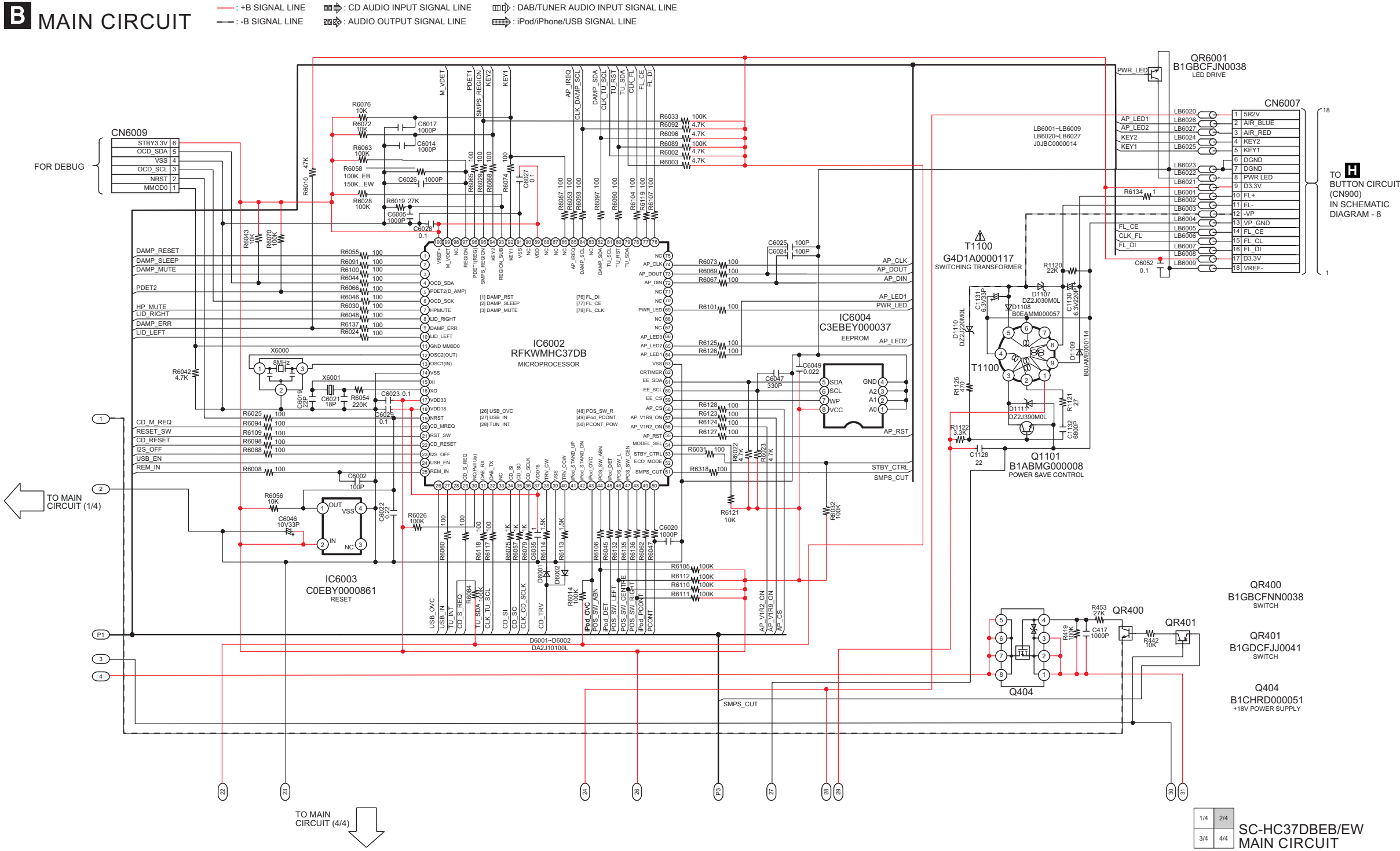
SCHEMATIC DIAGRAM - 4
