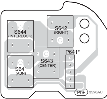
F INTERLOCK SWITCH P.C.B. (REP4776AC)
