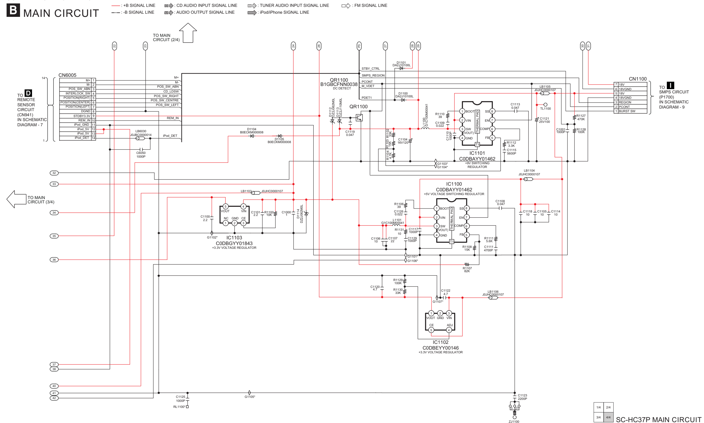
SCHEMATIC DIAGRAM - 6
