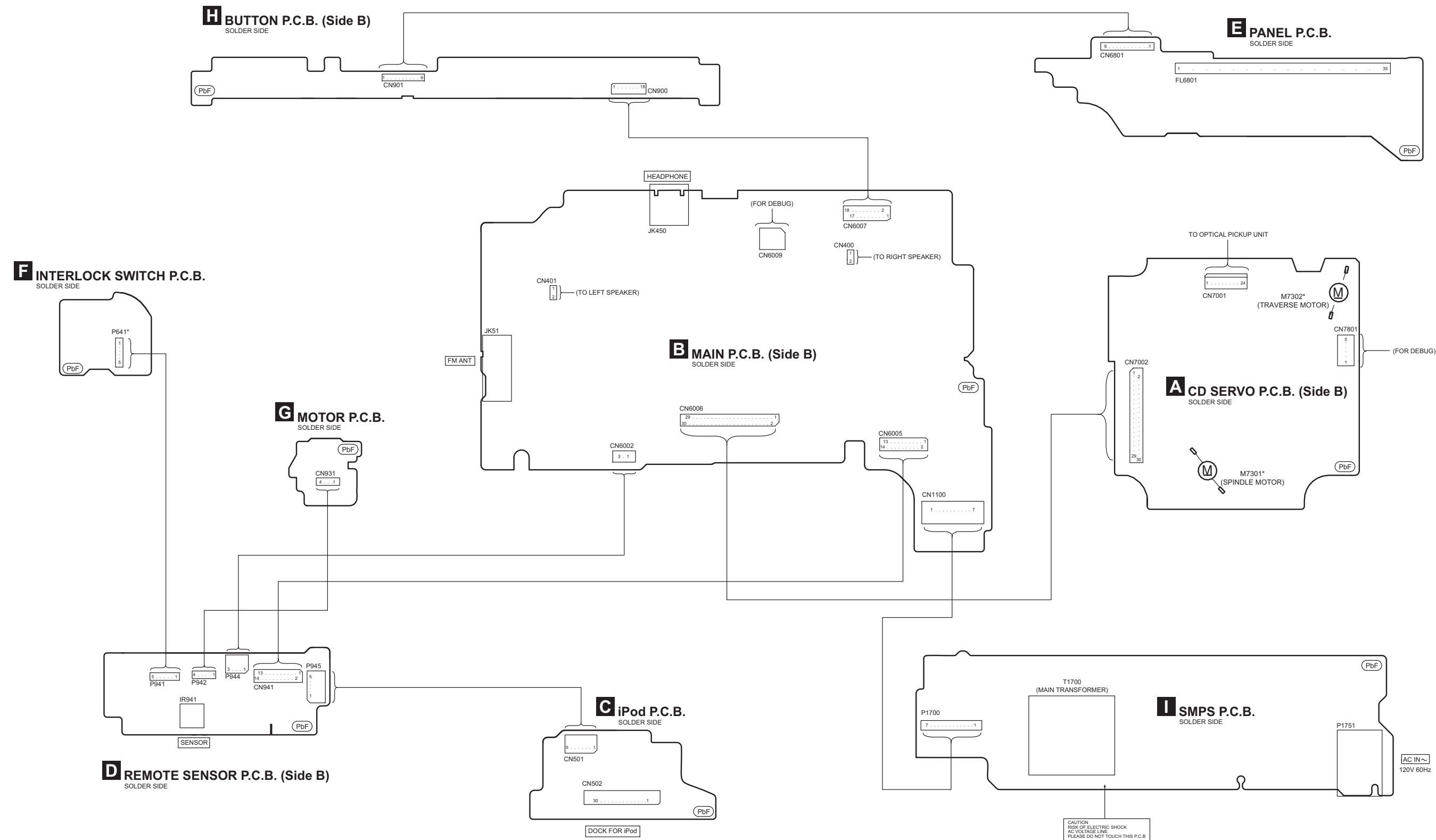
SC-HC37P WIRING CONNECTION DIAGRAM
