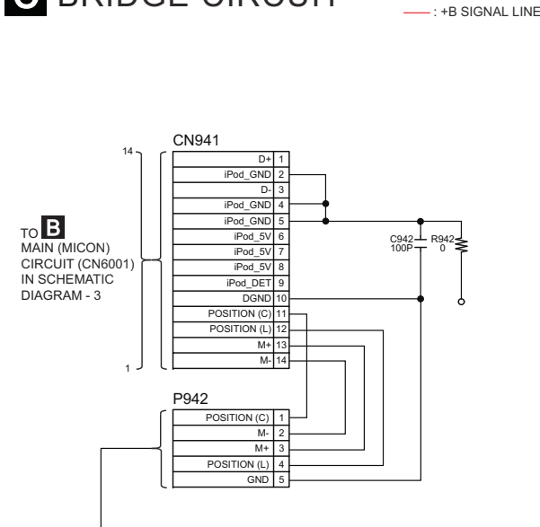
SCHEMATIC DIAGRAM - 9
