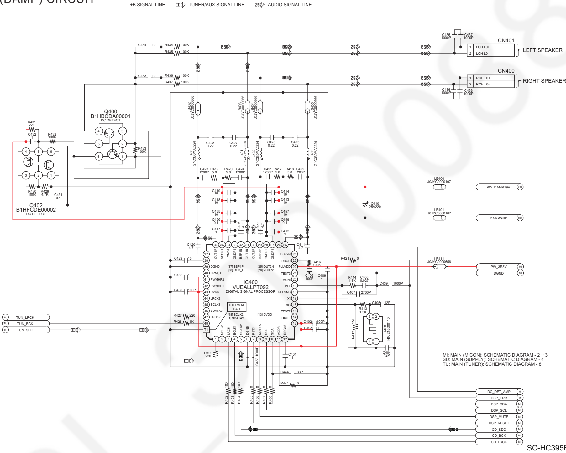
SCHEMATIC DIAGRAM - 7
