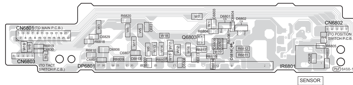
E PANEL P.C.B. (TNPA6408AB)
