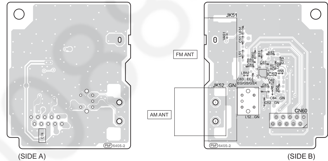
G TUNER P.C.B. (TNPA6405AD...HC400EE/EG, TNPA6405AJ...HC400GN, TNPA6405AK...HC400GS/GSX)
