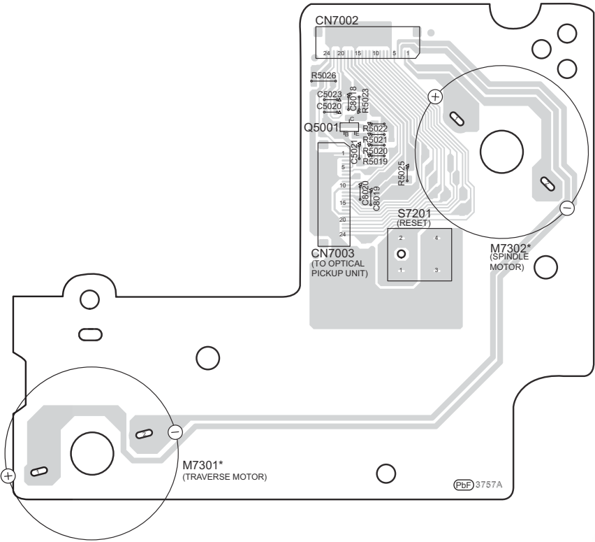
D MOTOR P.C.B. (TNPA6401AD...HC400EE/EG, TNPA6401AJ...HC400GN, TNPA6401AK...HC400GS/GSX)
