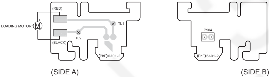
D MOTOR P.C.B. (TNPA6401AD...HC400EE/EG, TNPA6401AJ...HC400GN, TNPA6401AK...HC400GS/GSX)
