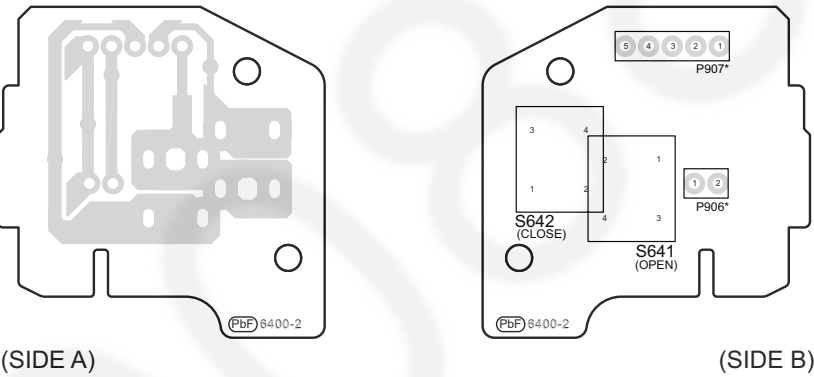
C POSITION SWITCH P.C.B. (TNPA6400AD...HC400EE/EG, TNPA6400AJ...HC400GN, TNPA6400AK...HC400GS/GSX)
