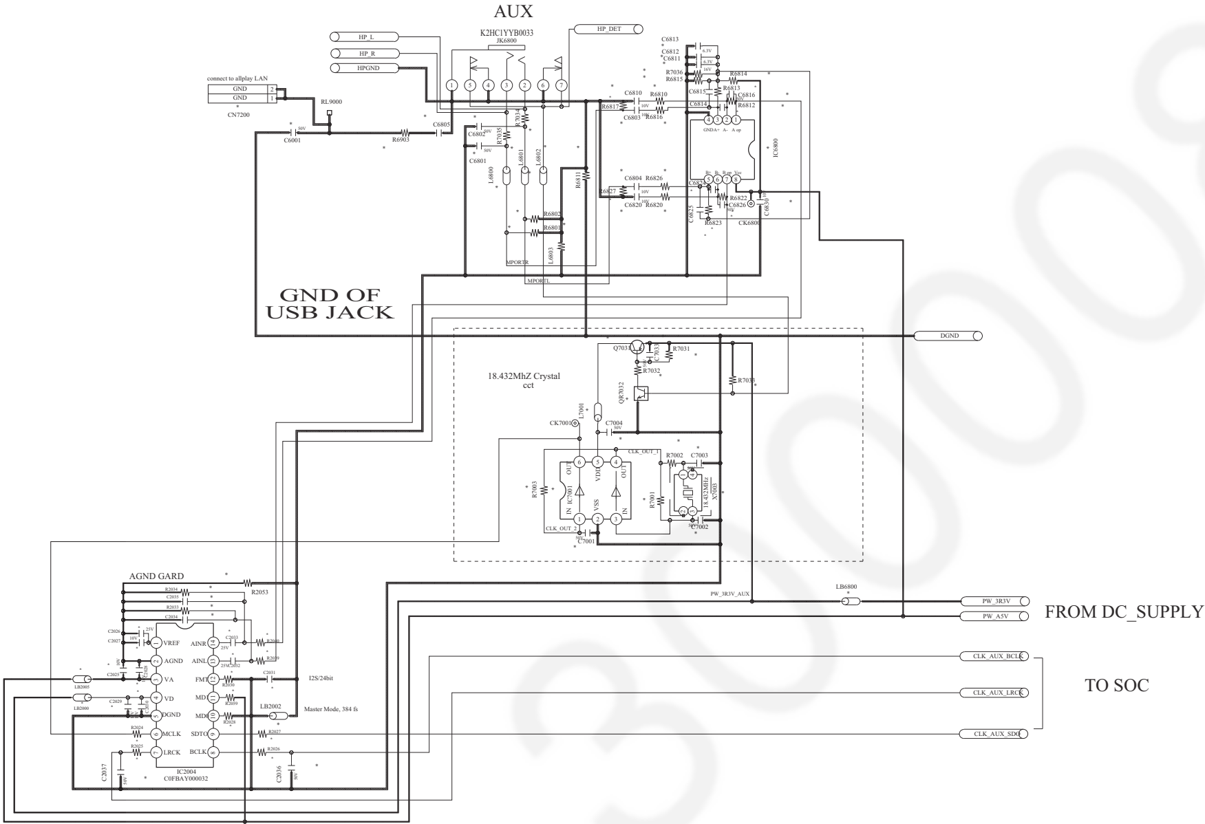
SCHEMATIC DIAGRAM - 6 B MAIN (AUX) CIRCUIT
