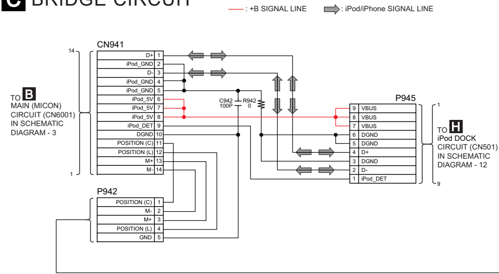
SCHEMATIC DIAGRAM - 9
