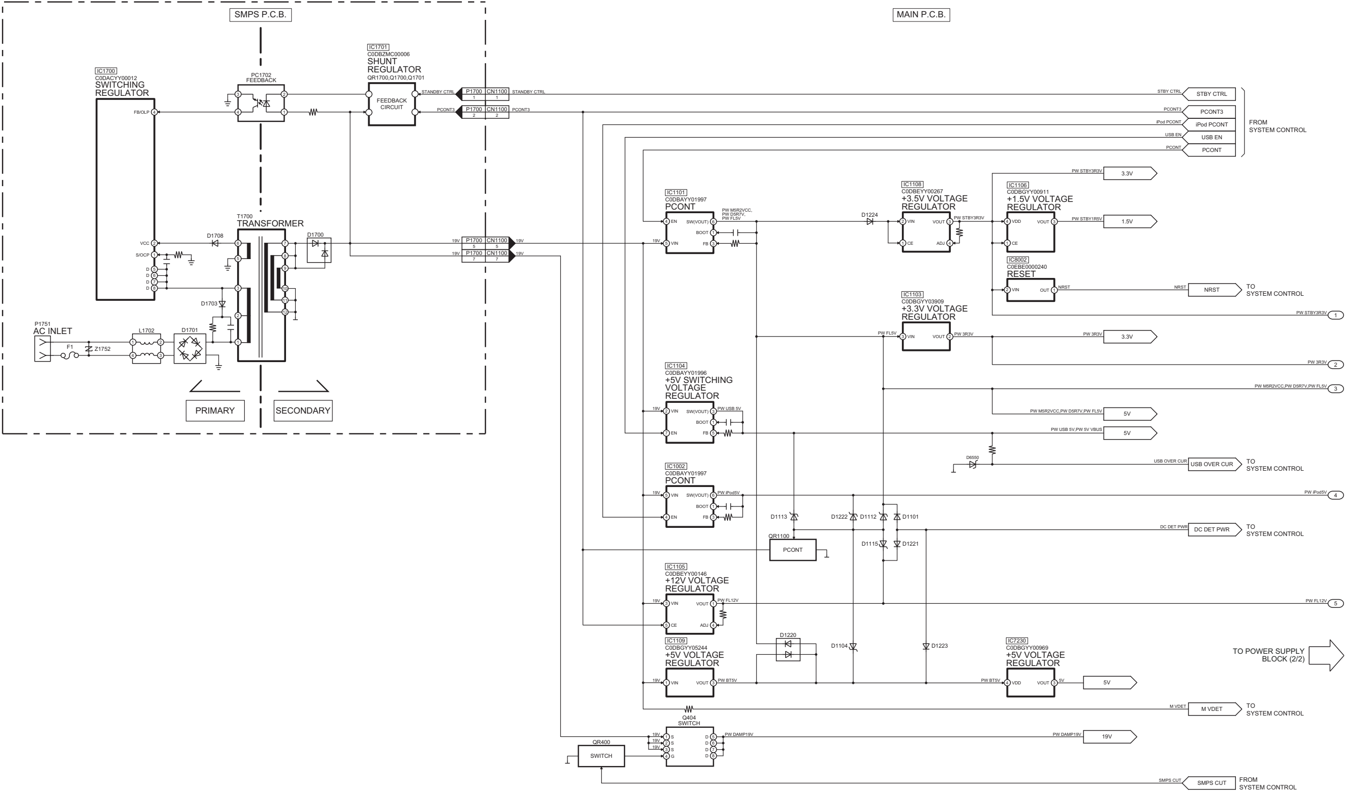
SC-HC49EG POWER SUPPLY (1/2) BLOCK DIAGRAM
