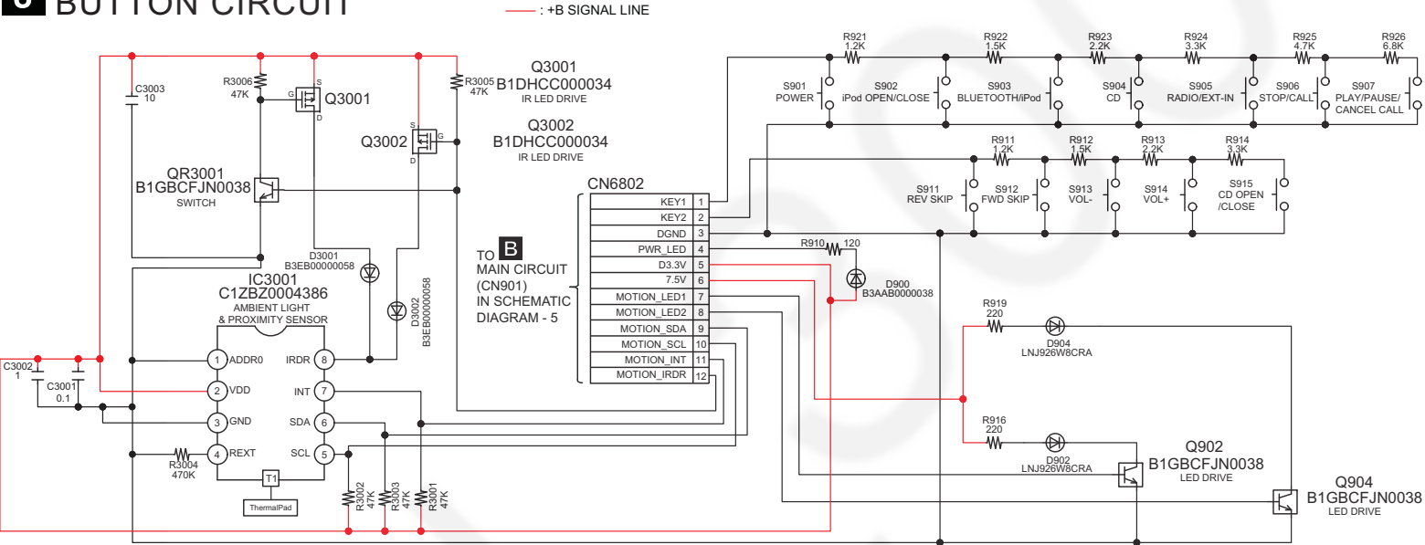
J BUTTON CIRCUIT
