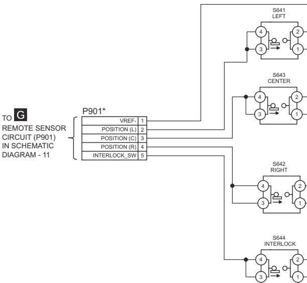
I INTERLOCK SWITCH CIRCUIT
