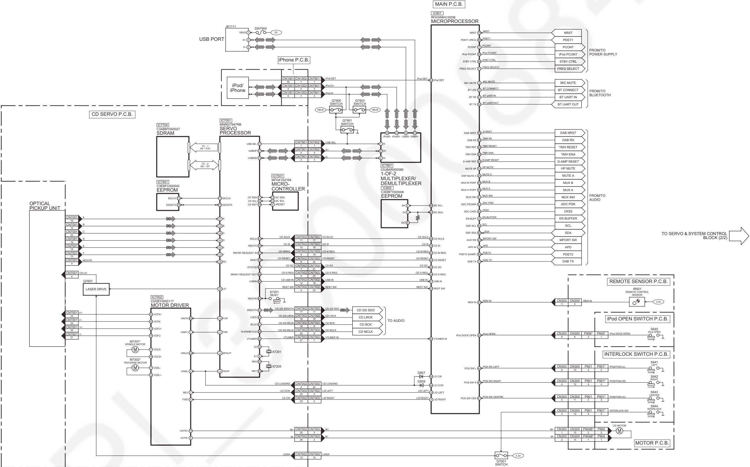
SC-HC55DBEB SERVO & SYSTEM CONTROL (1/2) BLOCK DIAGRAM
