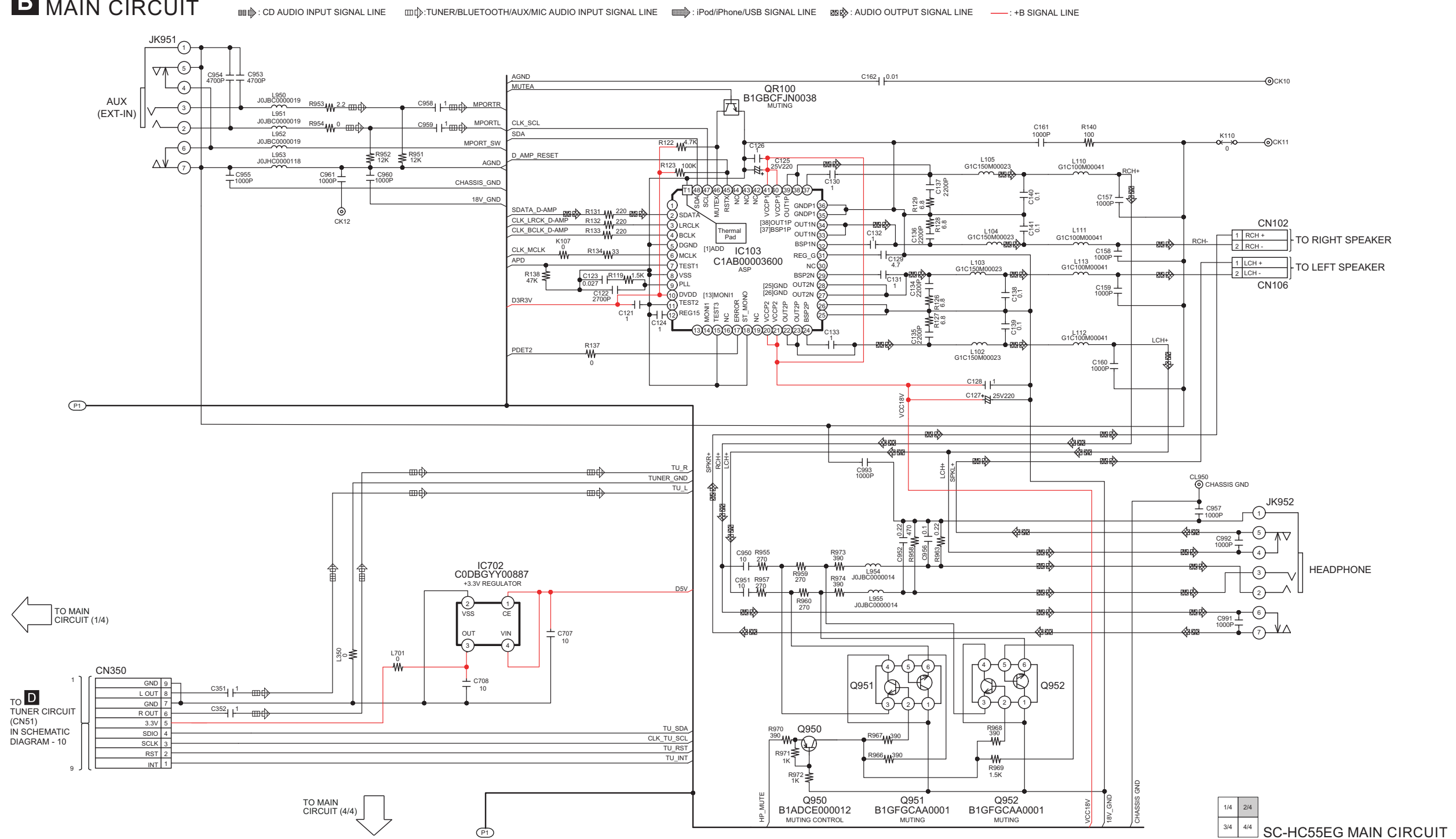
SCHEMATIC DIAGRAM - 4
