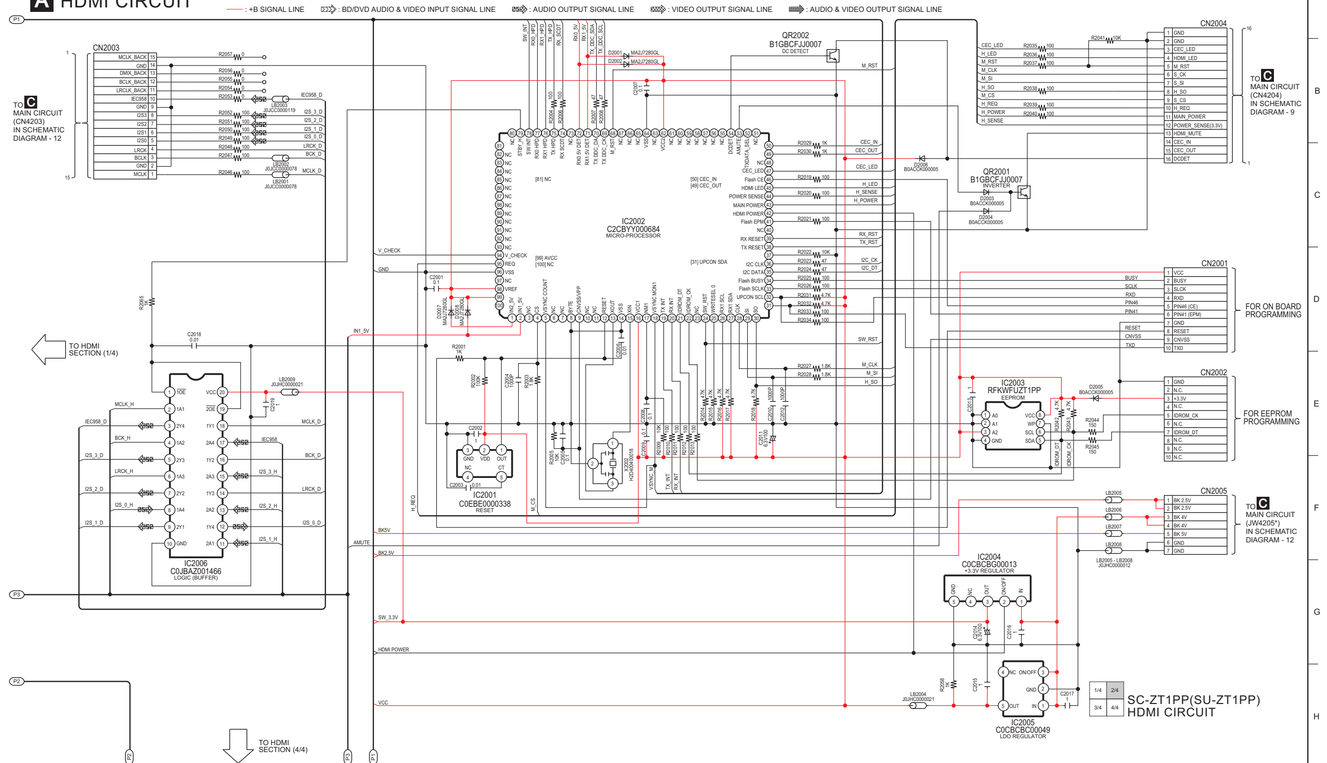
SCHEMATIC DIAGRAM - 2
