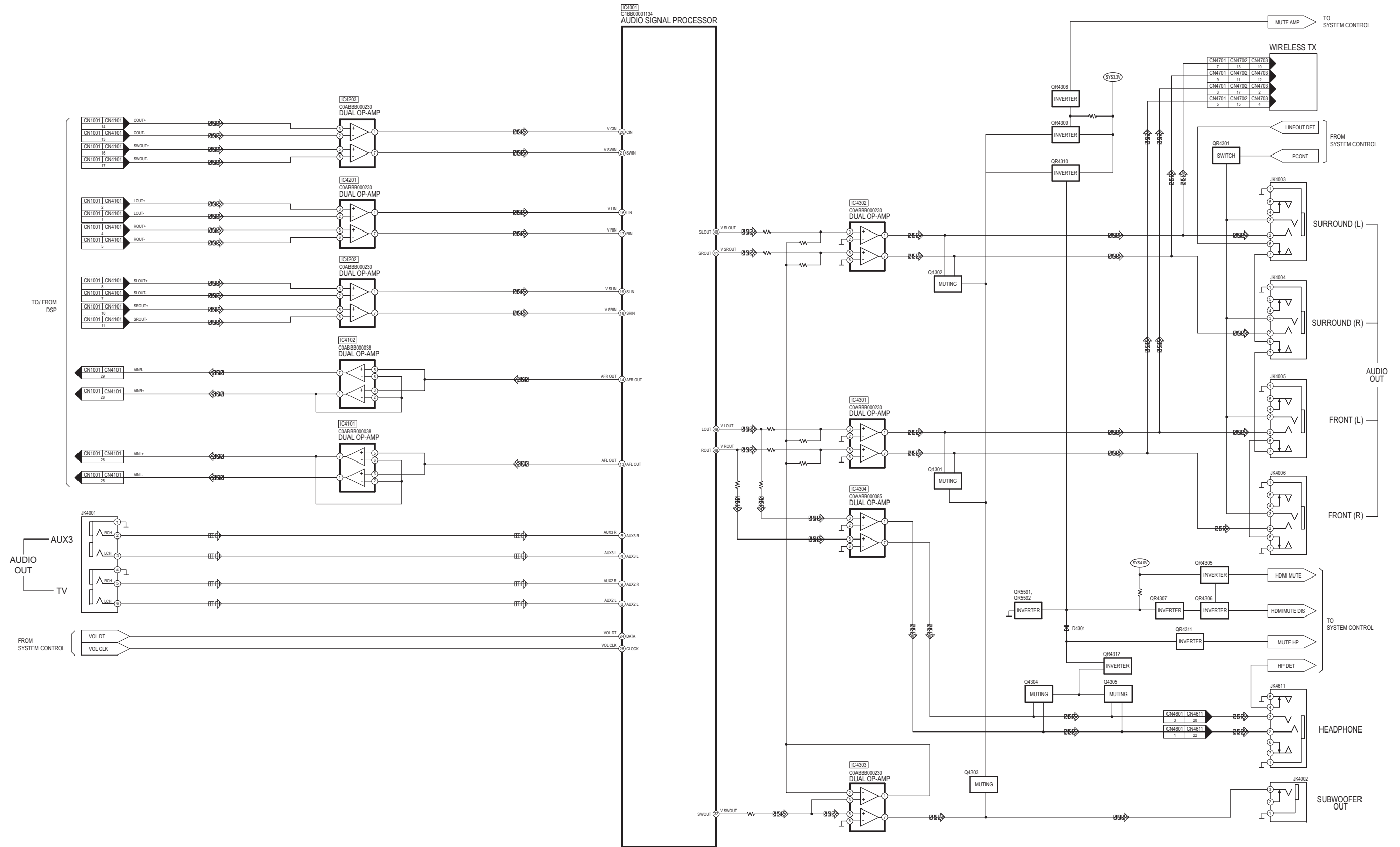
SC-ZT1PP (SU-ZT1PP) AUDIO BLOCK DIAGRAM
