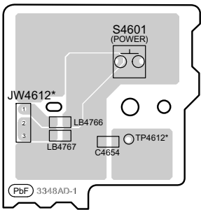
E POWER SW P.C.B. (REP4526B)
