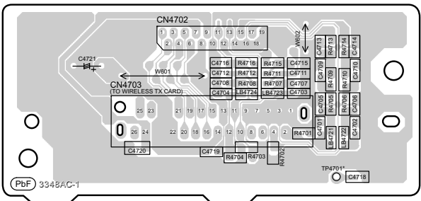
F WIRELESS TX P.C.B. (REP4526B)
