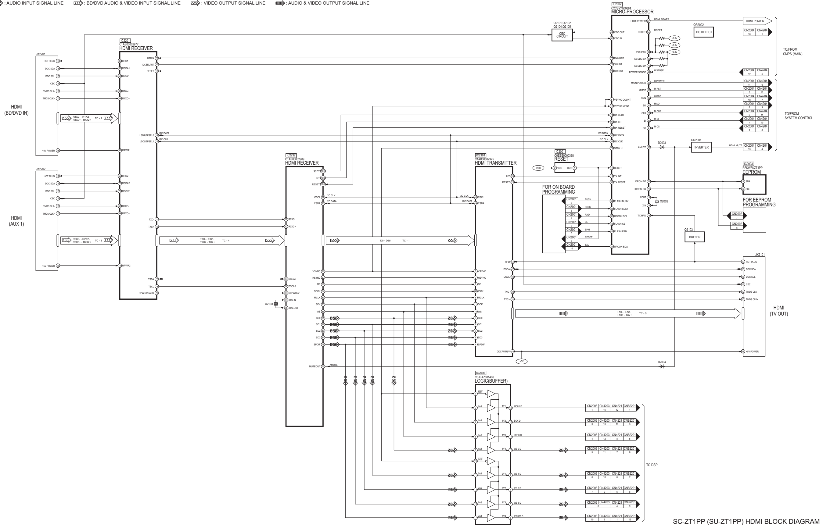
SC-ZT1PP (SU-ZT1PP) HDMI BLOCK DIAGRAM
