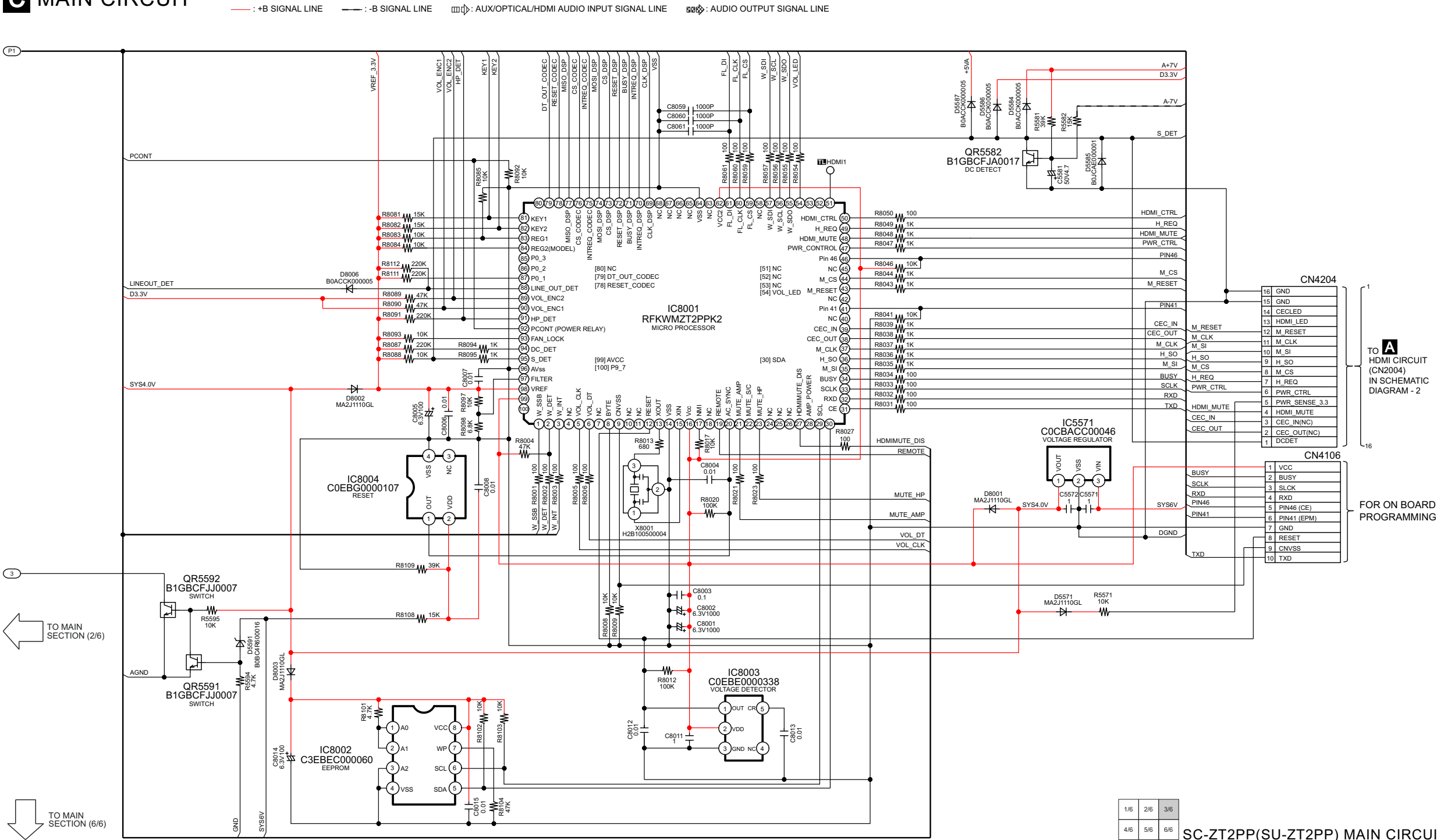
SCHEMATIC DIAGRAM - 9
