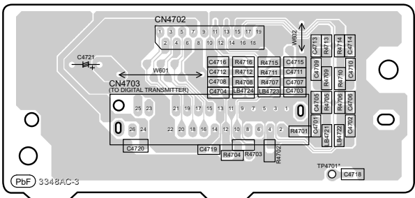
F WIRELESS ADAPTER P.C.B. (REP4526EC)
