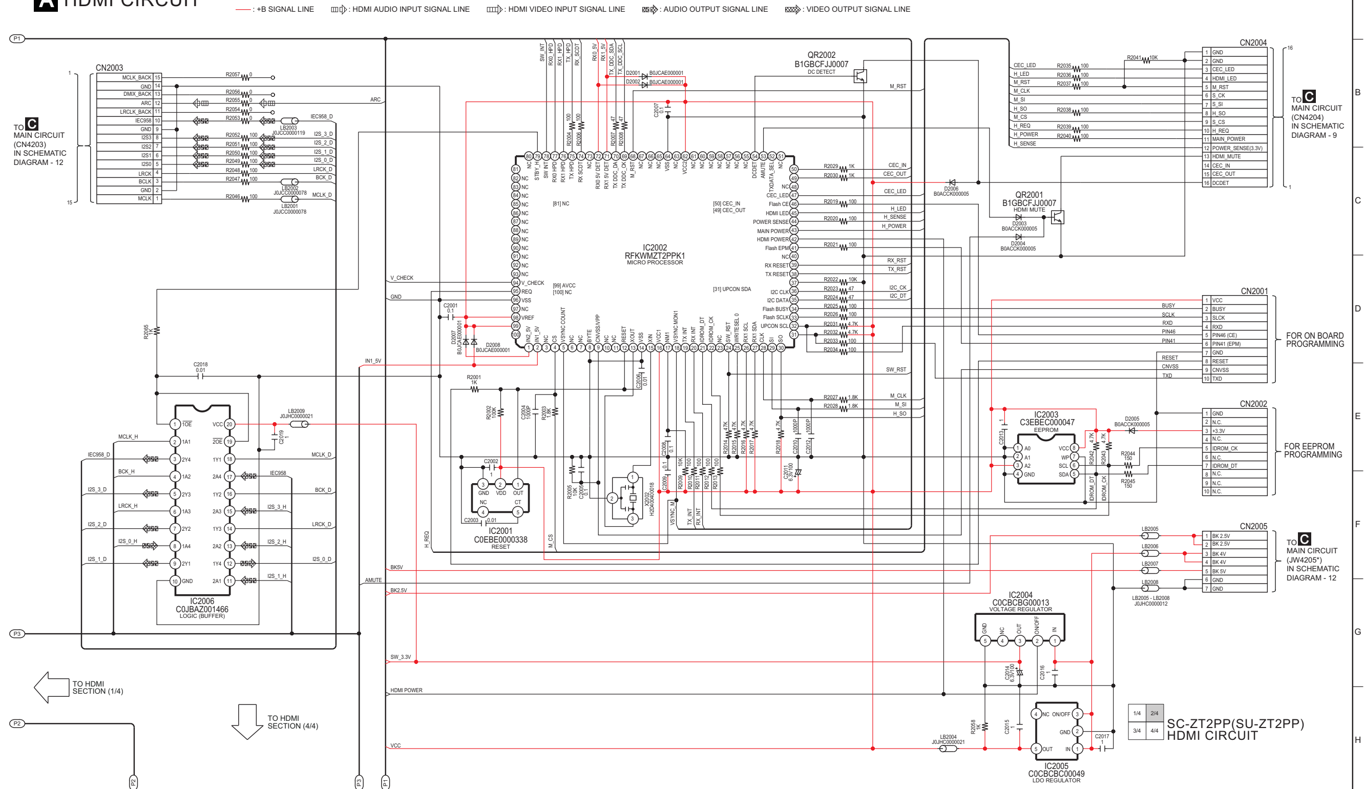
SCHEMATIC DIAGRAM - 2
