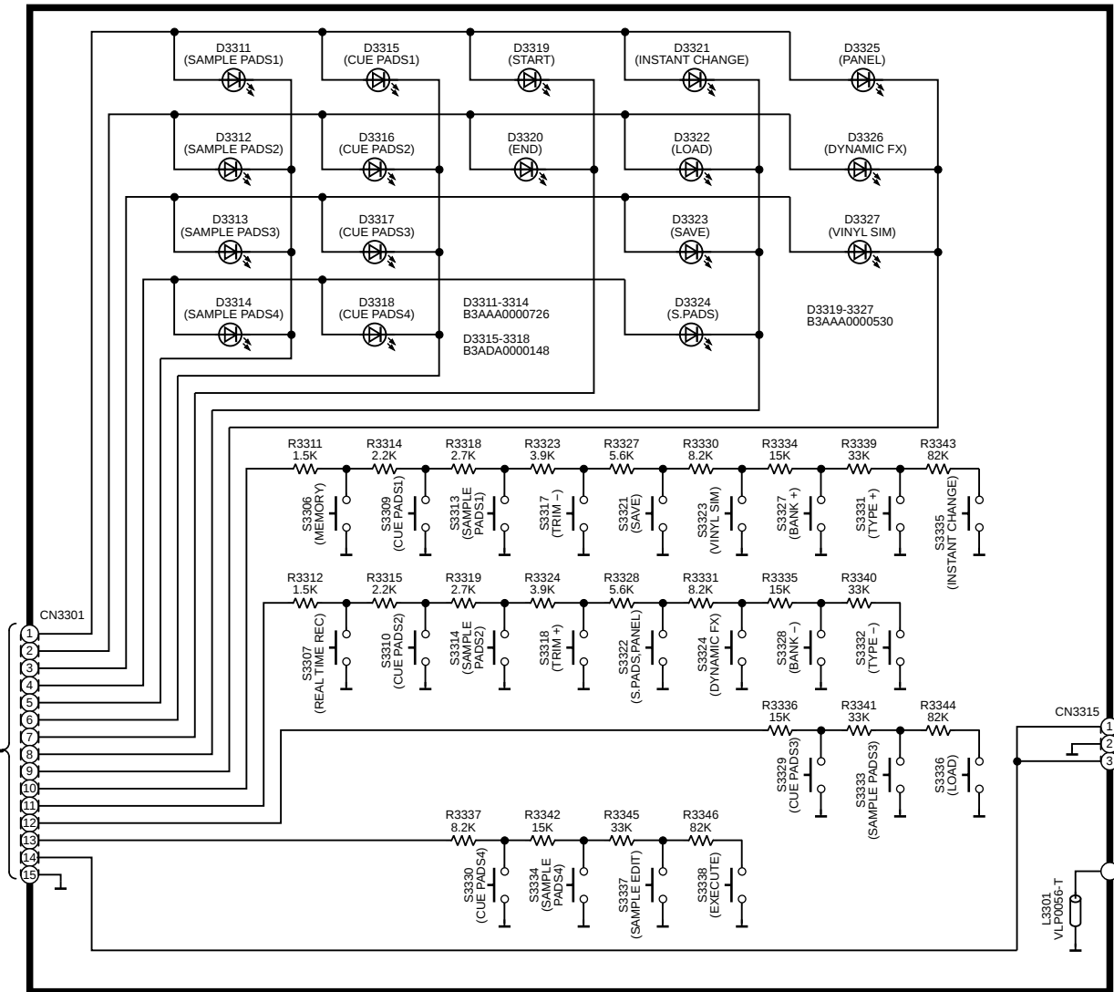
SCHEMATIC DIAGRAM-14 H CONTROL PANEL(1) CIRCUIT → :POSITIVE VOLTAGE LINE → :NEGATIVE VOLTAGE LINE
