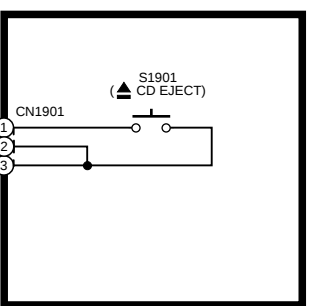
M EJECT SW CIRCUIT
