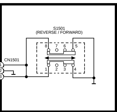
J REVERSE SW CIRCUIT
