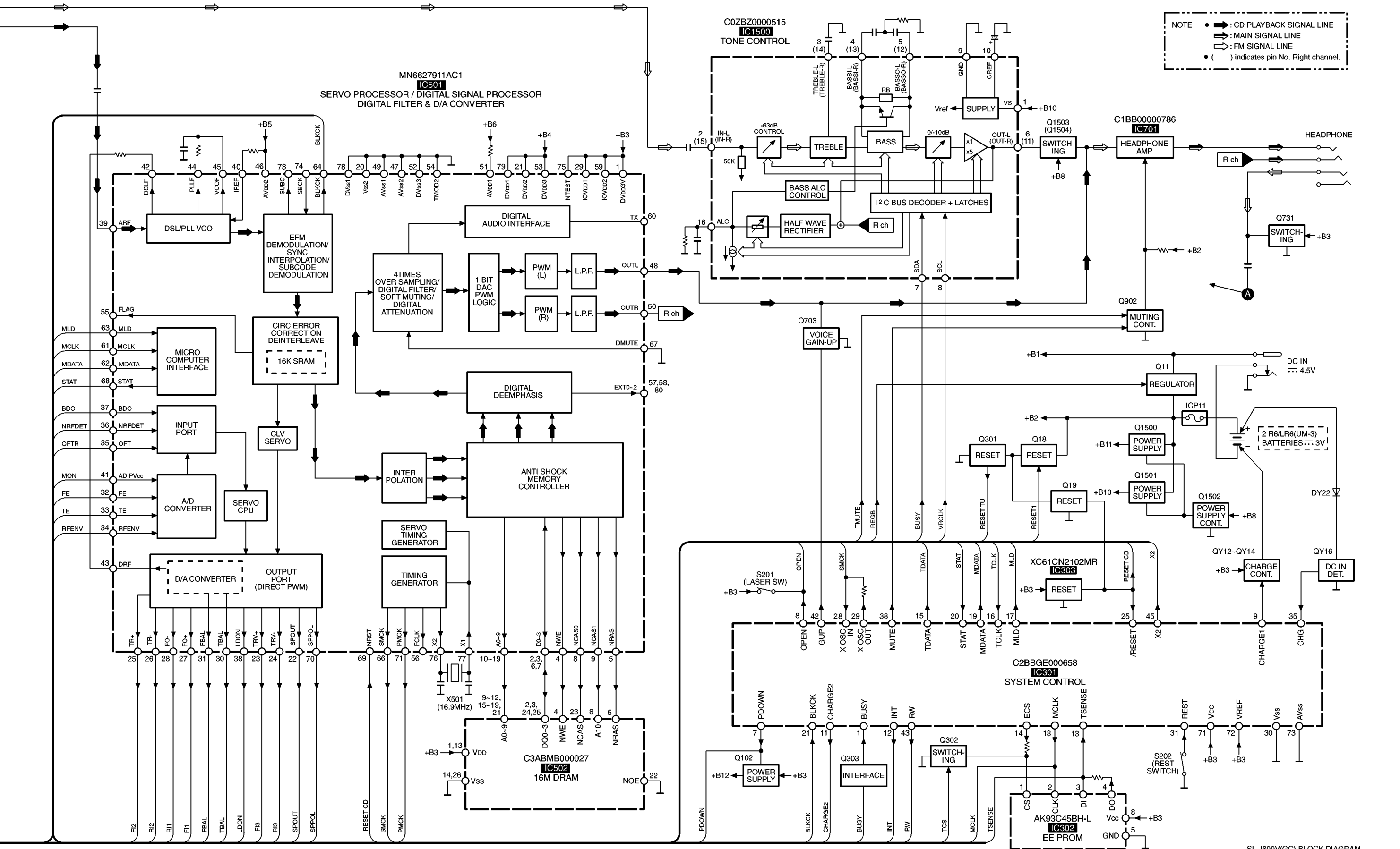
SL-J600V(GC) BLOCK DIAGRAM
