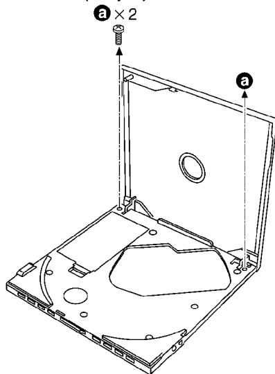
Intermediate cabinet ass'y
