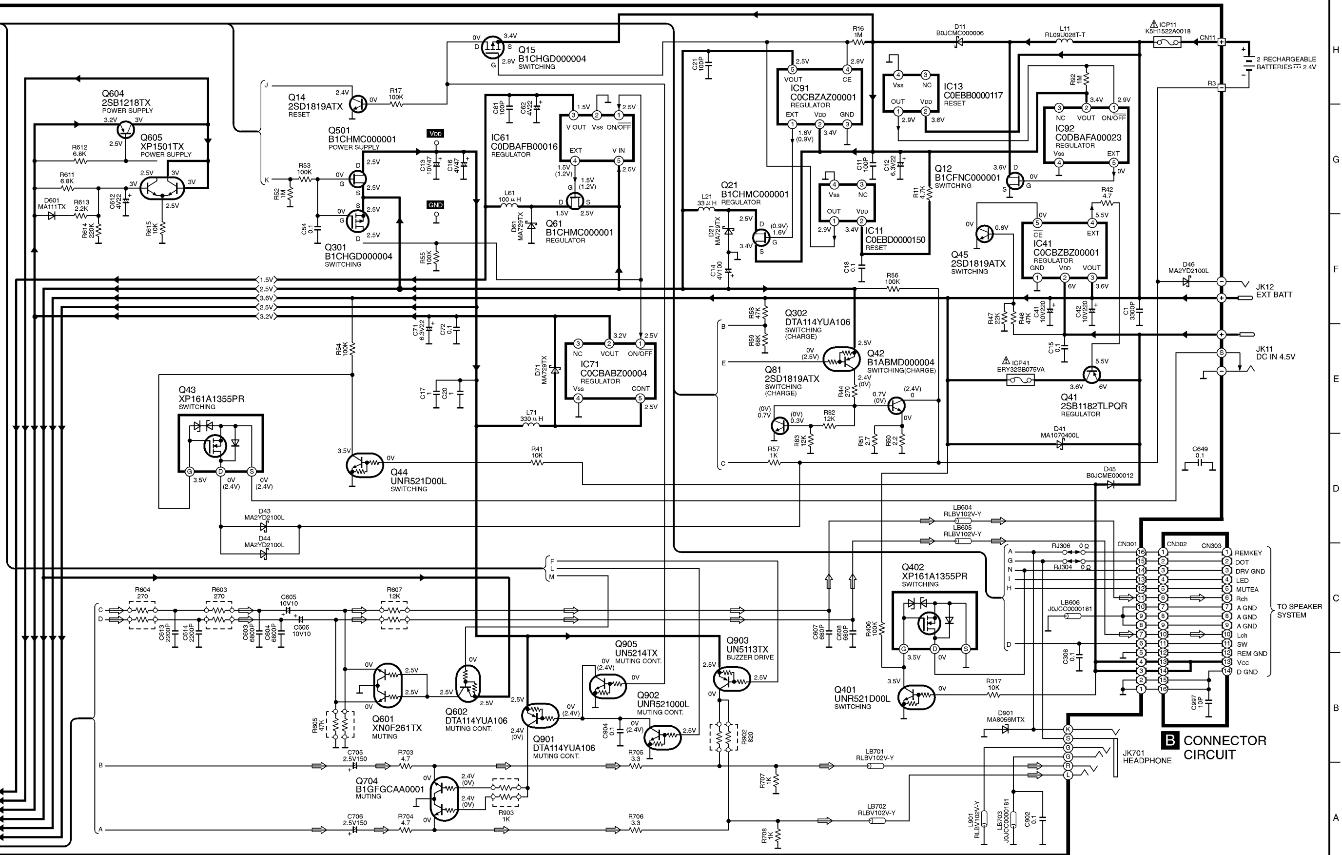
SL-J910(SG, GD) MAIN, CONNECTOR CIRCUIT DIAGRAM
