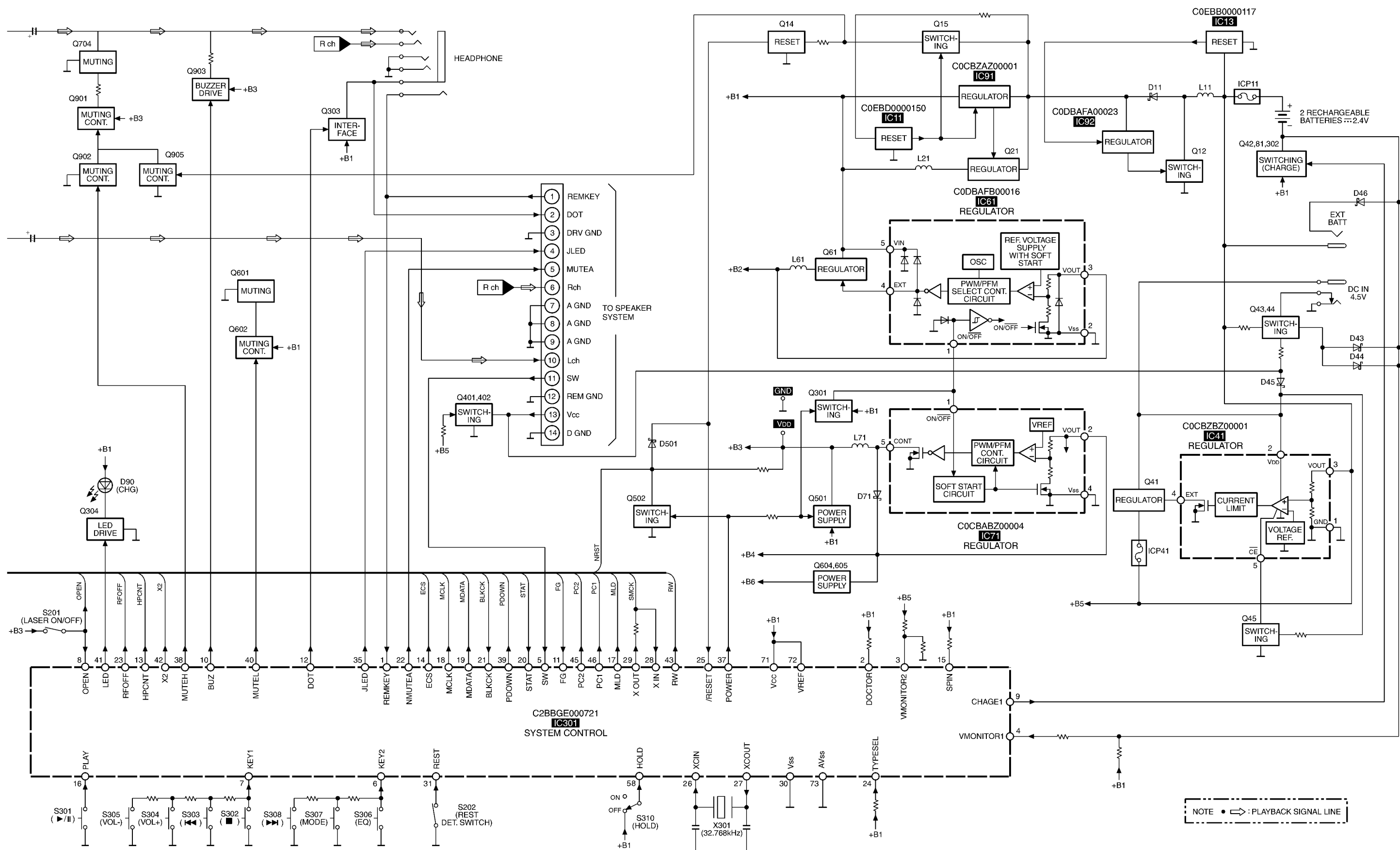
SL-J910(SG,GD) BLOCK DIAGRAM
