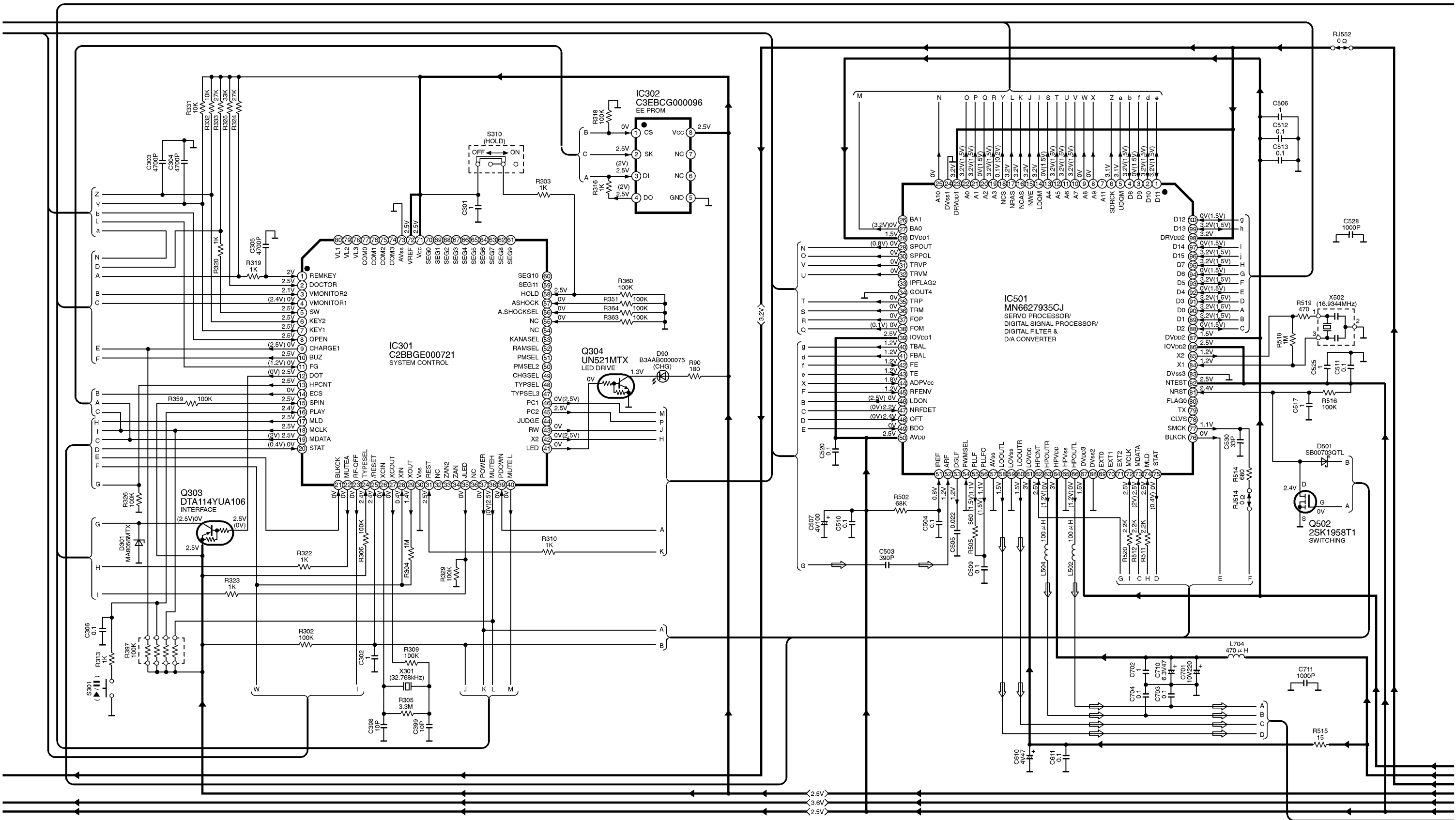
SL-J910(SG,GD) MAIN CIRCUIT DIAGRAM
