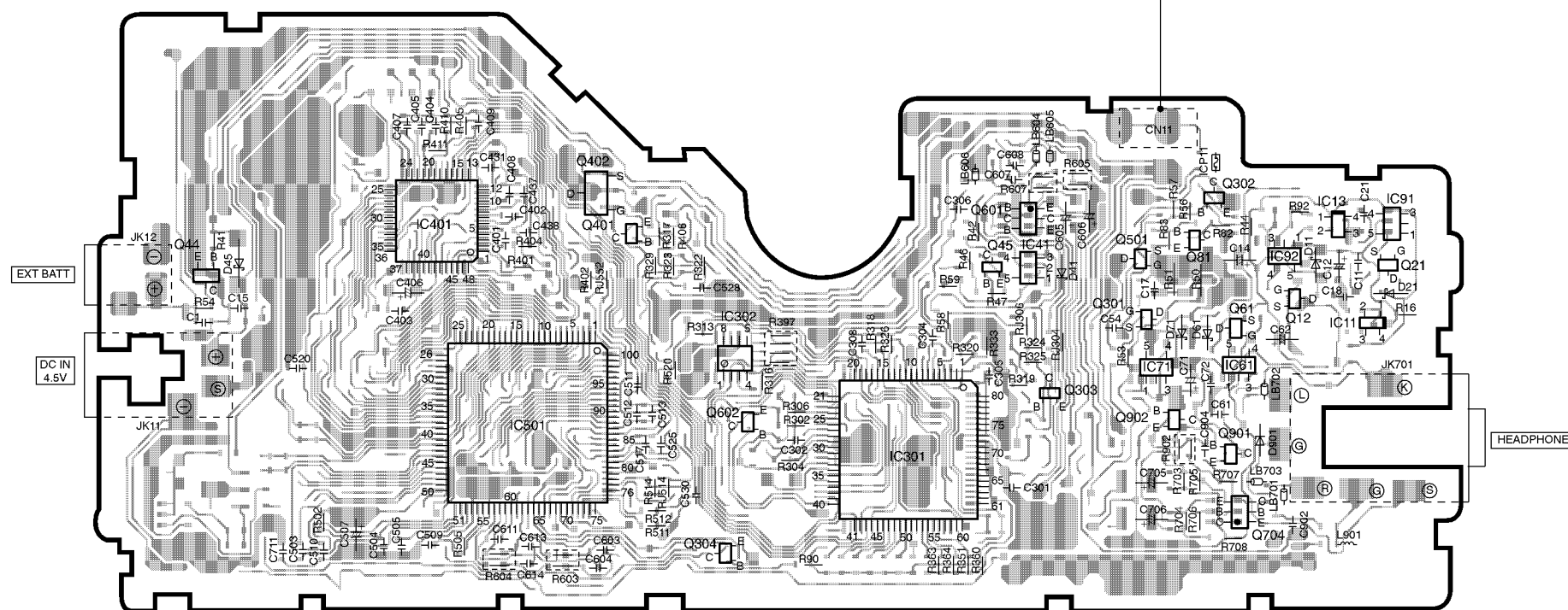
A MAIN P.C.B.(SIDE:B)
