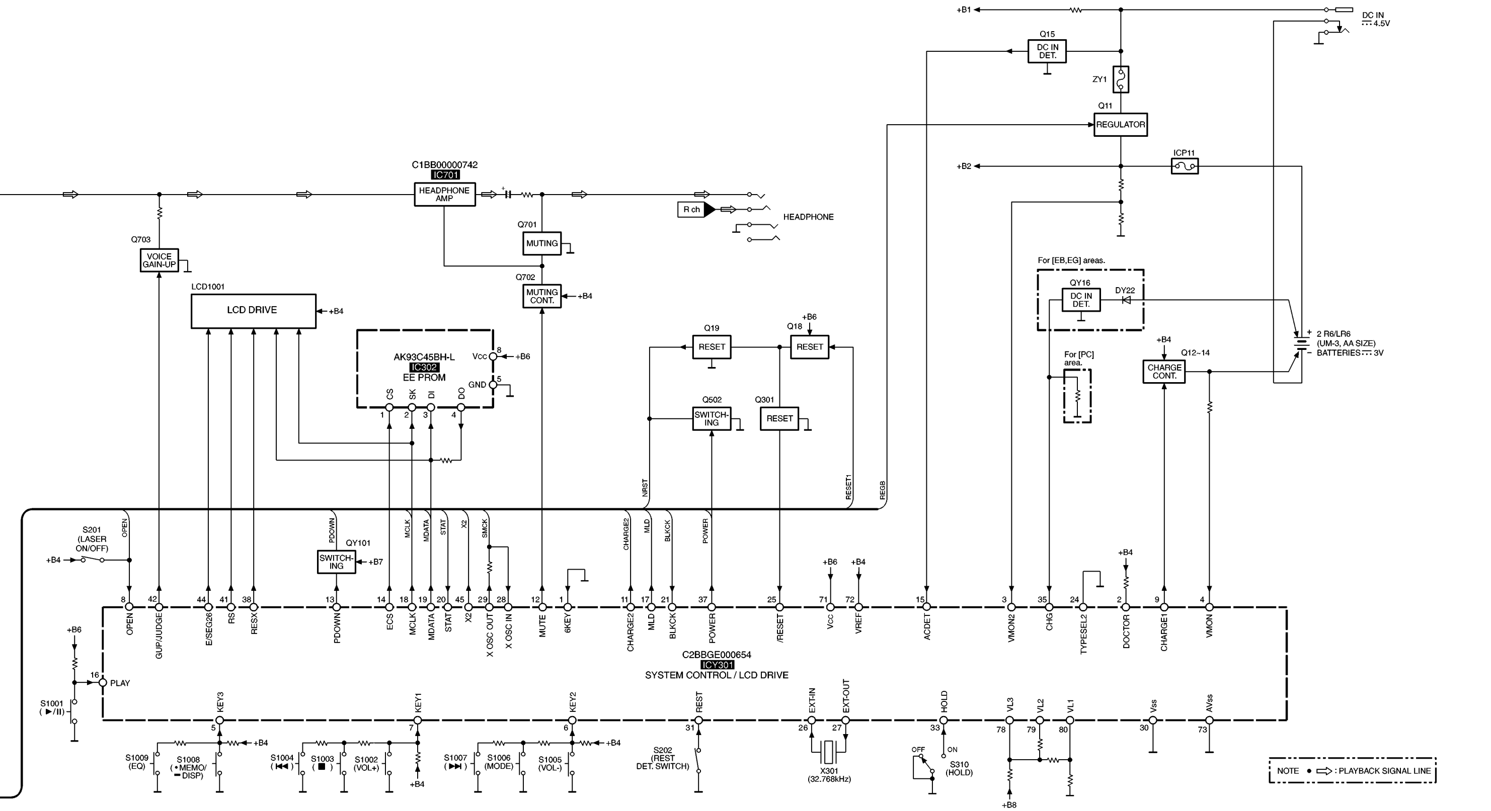
SL-MP70(EB,EG),SL-MP71C(PC,EB,EG) BLOCK DIAGRAM
