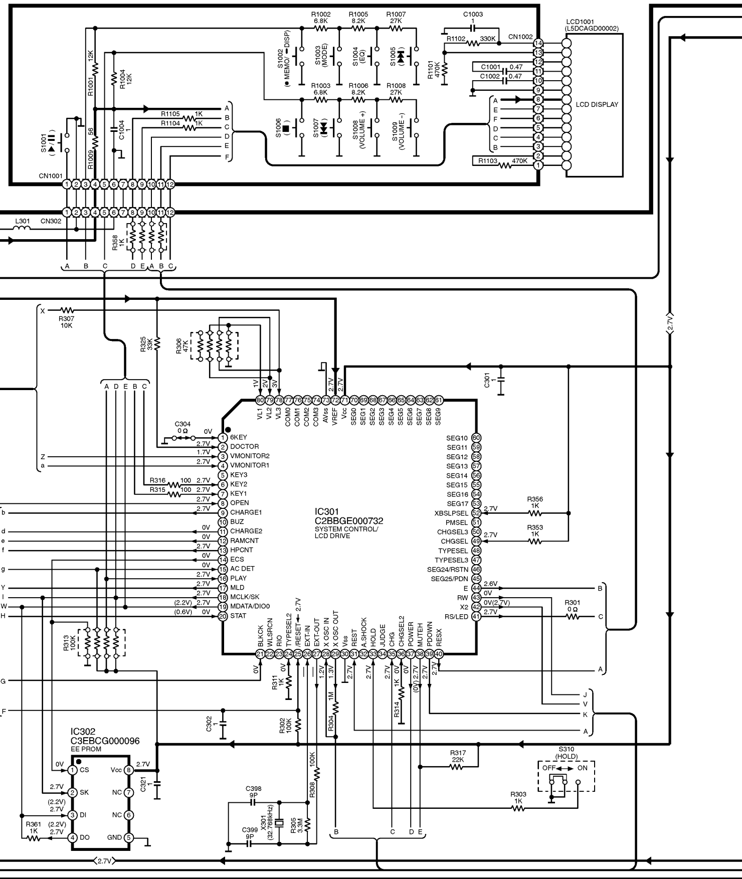
SL-MP76C(EB,EG) MAIN,OPERATION CIRCUIT DIAGRAM
