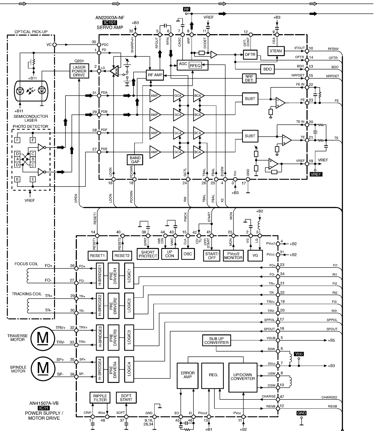
SL-SV570(EB,EG,GN)/SV572(GC,GS) BLOCK DIAGRAM
