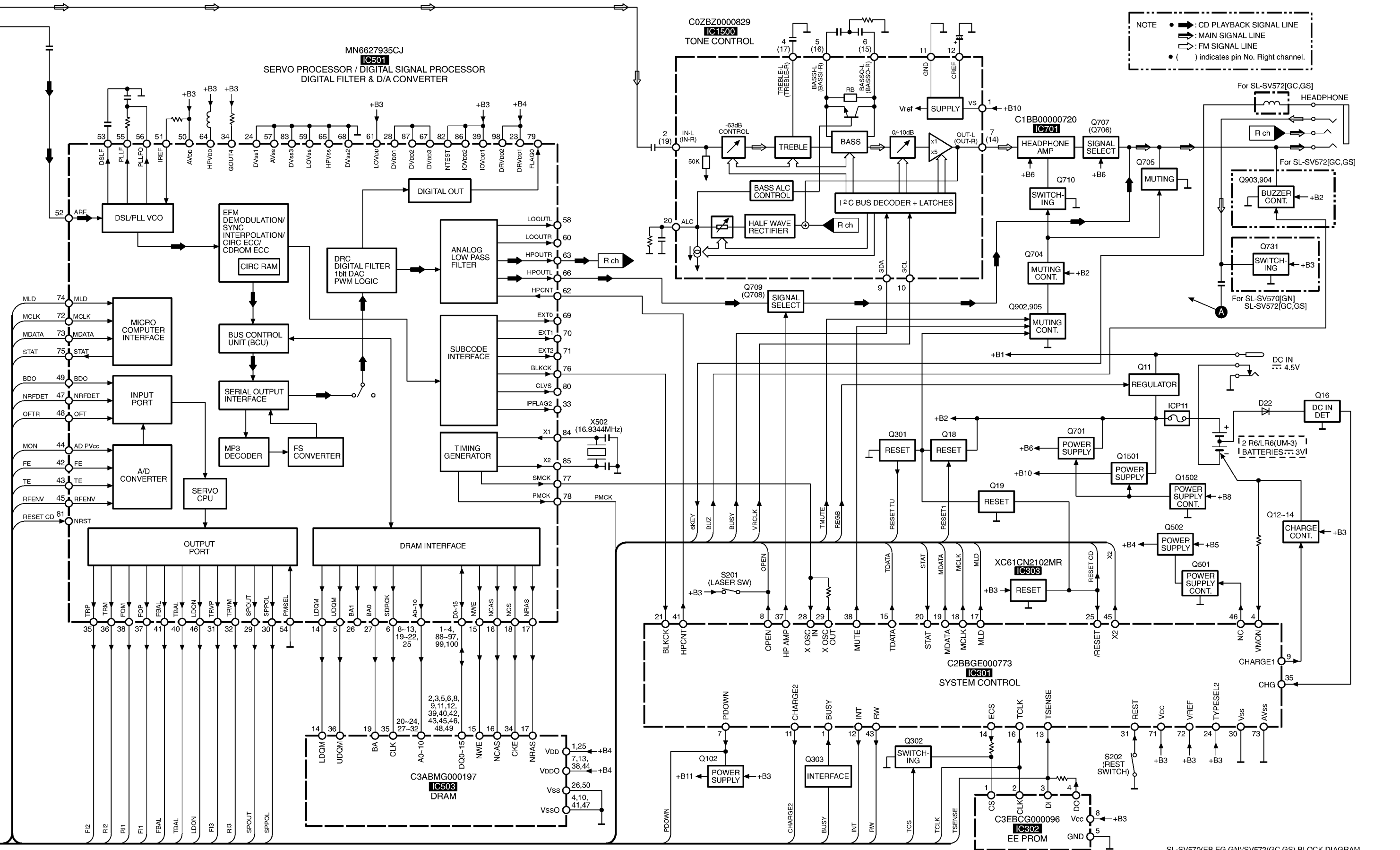
SL-SV570(EB,EG,GN)/SV572(GC,GS) BLOCK DIAGRAM
