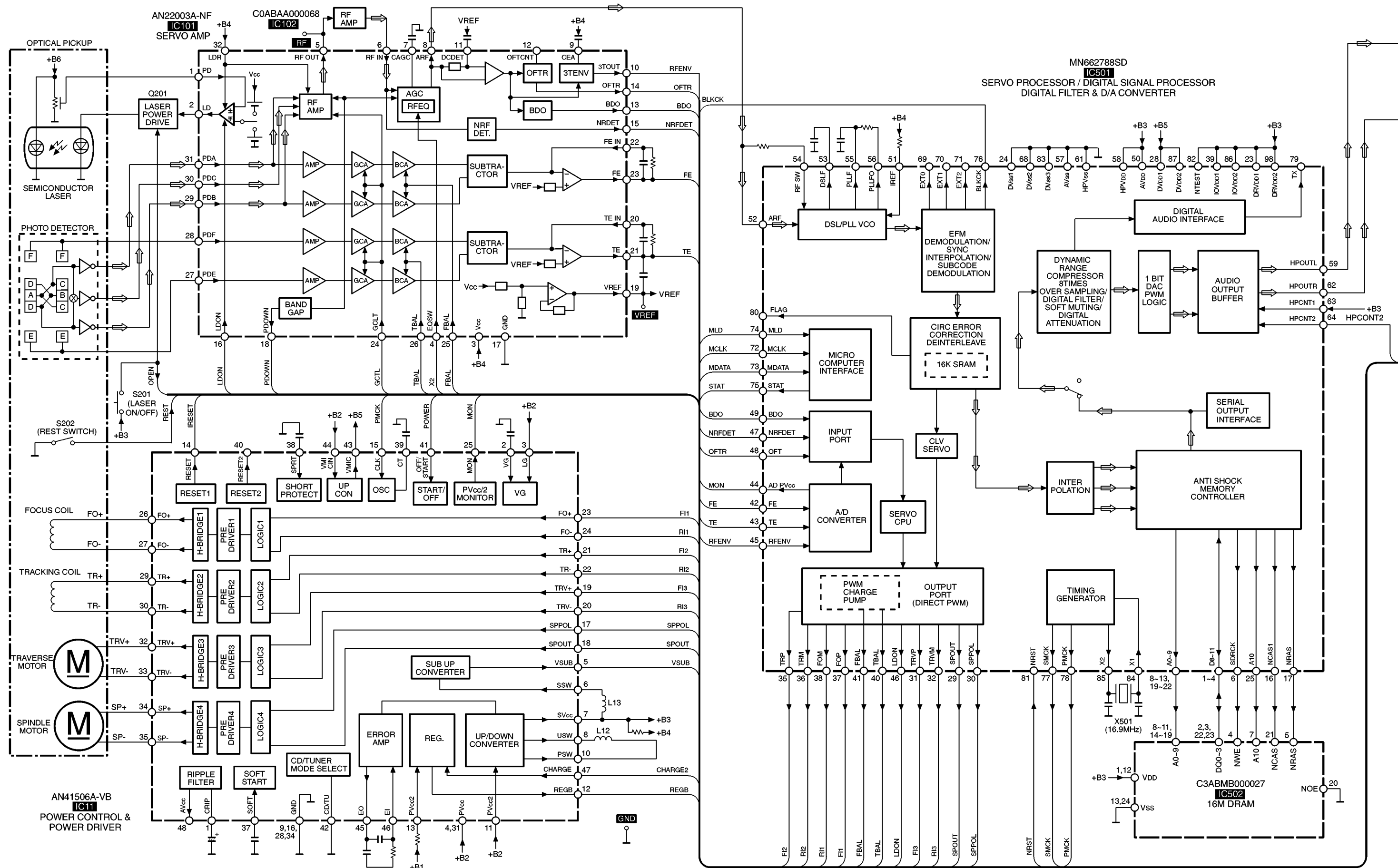
SL-SX315(EB,EG,E2)BLOCK DIAGRAM
