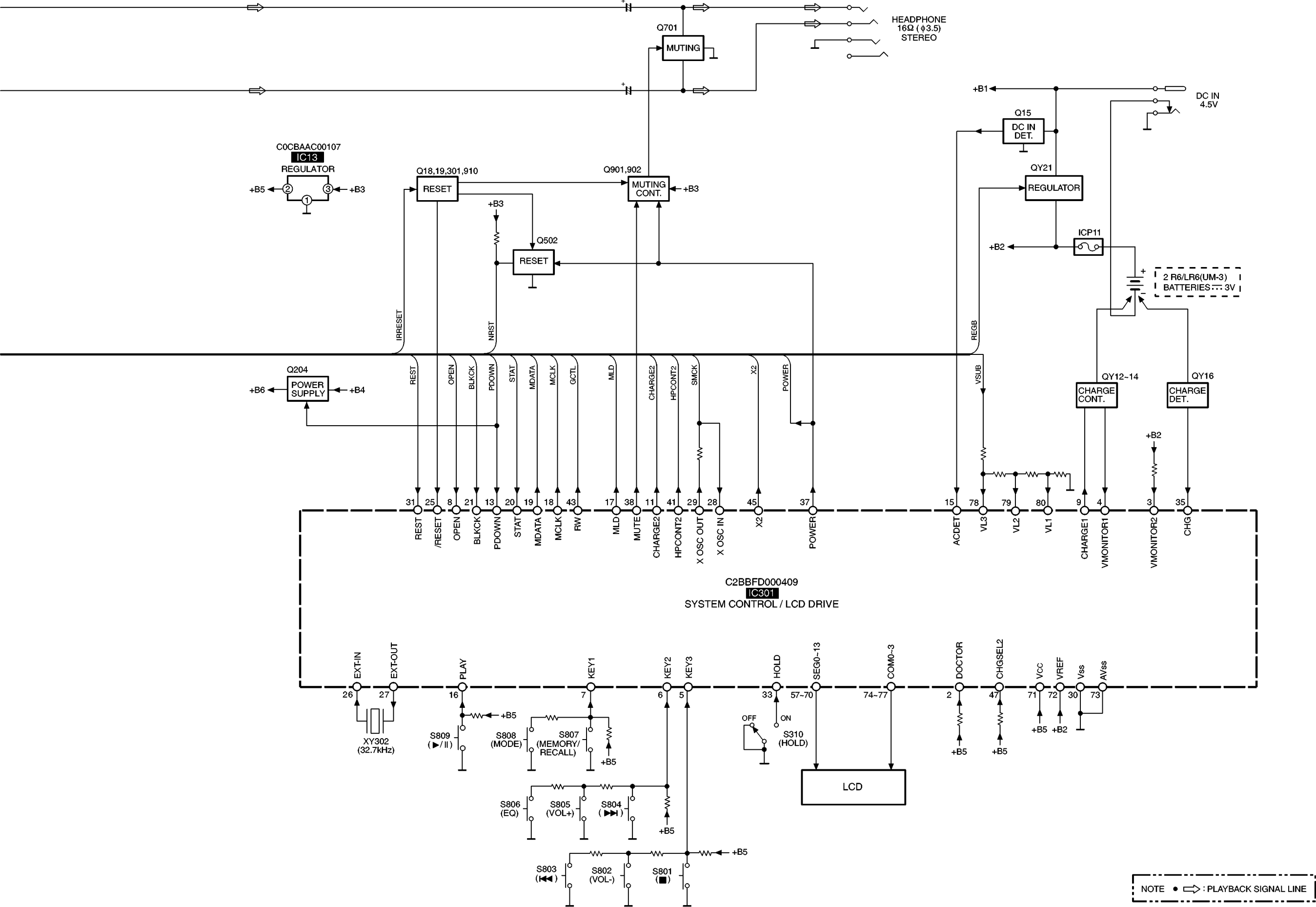
SL-SX320(EB,EG)BLOCK DIAGRAM
