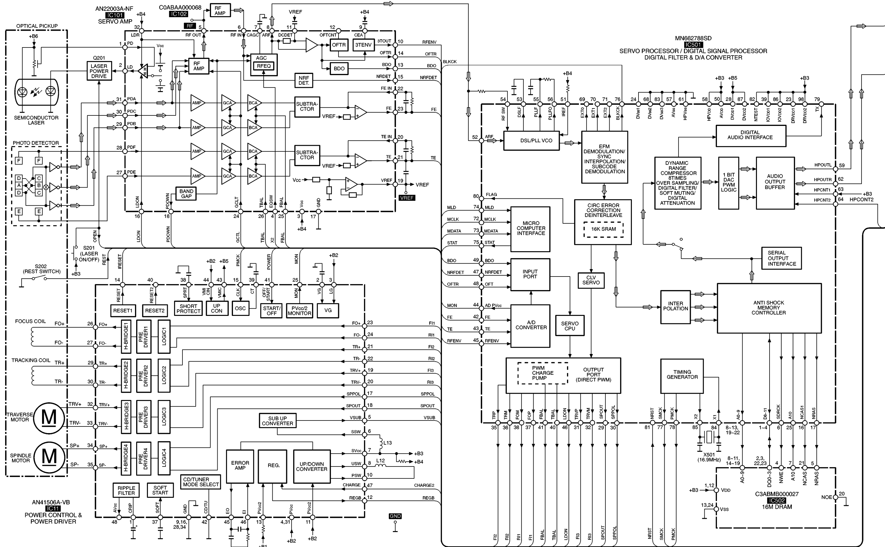
SL-SX320(EB,EG)BLOCK DIAGRAM
