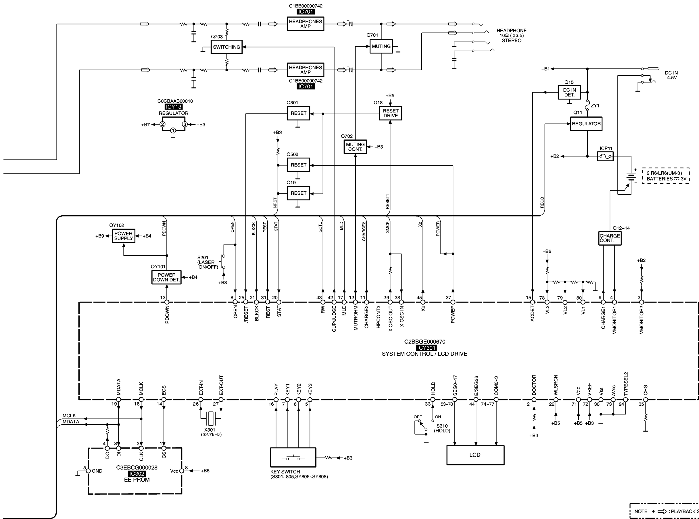
SL-SX419C(PC) BLOCK DIAGRAM
