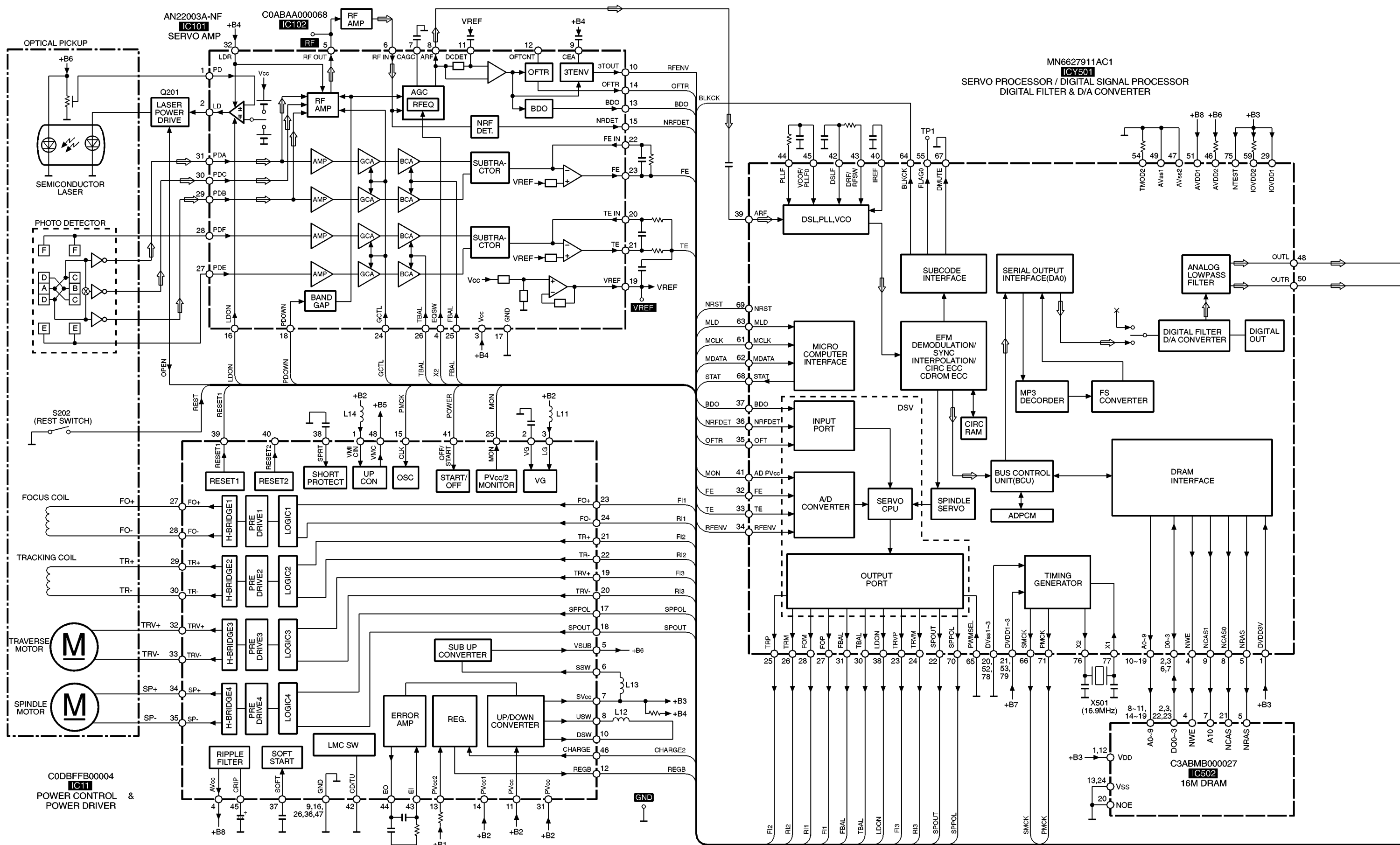
SL-SX419C(PC) BLOCK DIAGRAM
