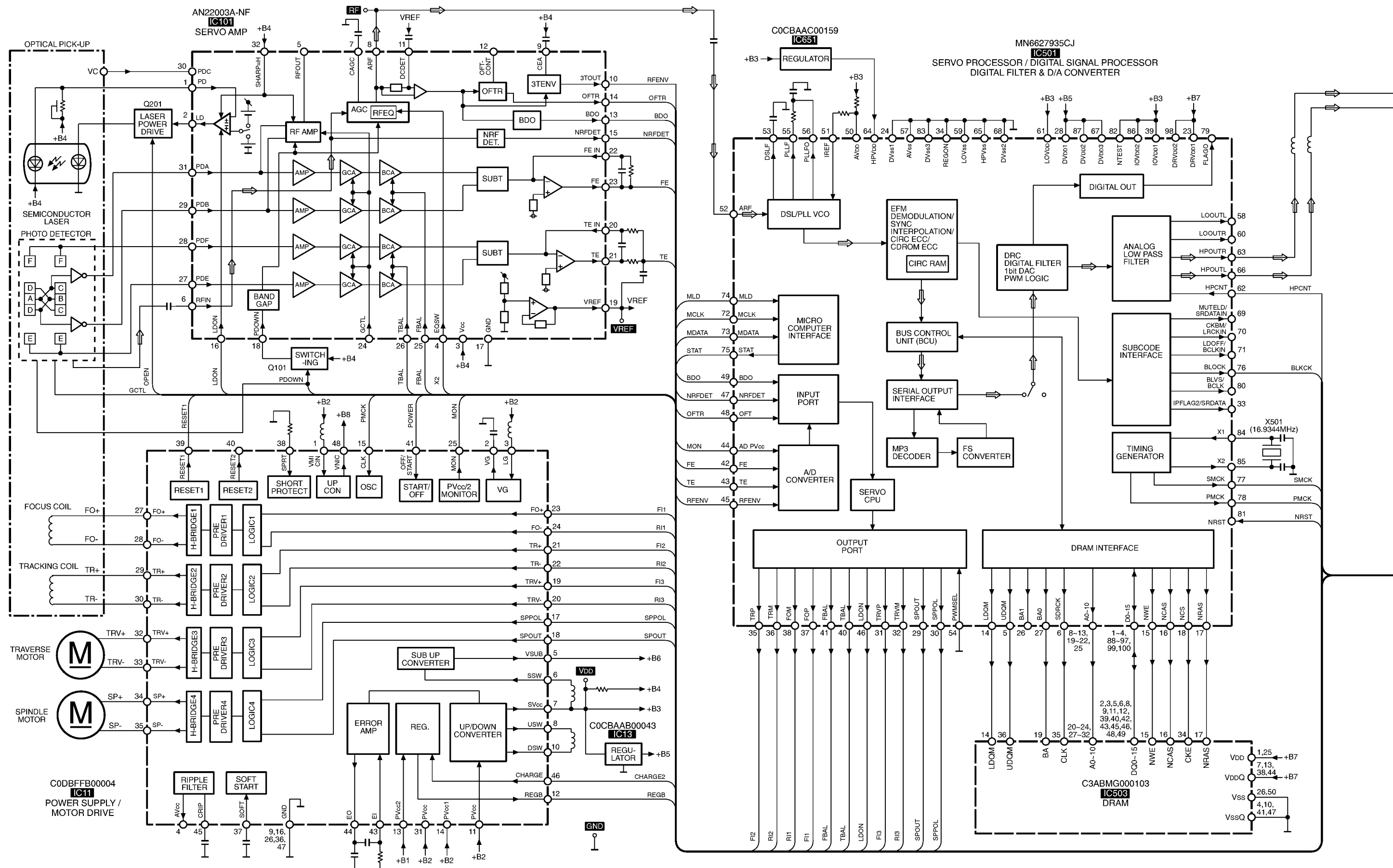
SL-SX428/429C(EB,EG,GN) BLOCK DIAGRAM
