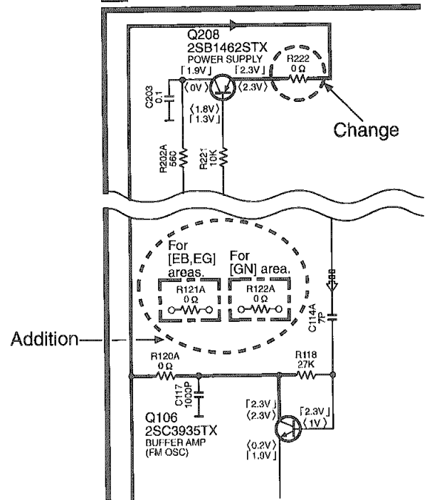
SCHEMATIC DIAGRAM-1
