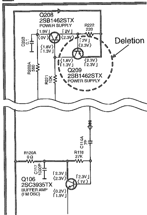
SCHEMATIC DIAGRAM-1
