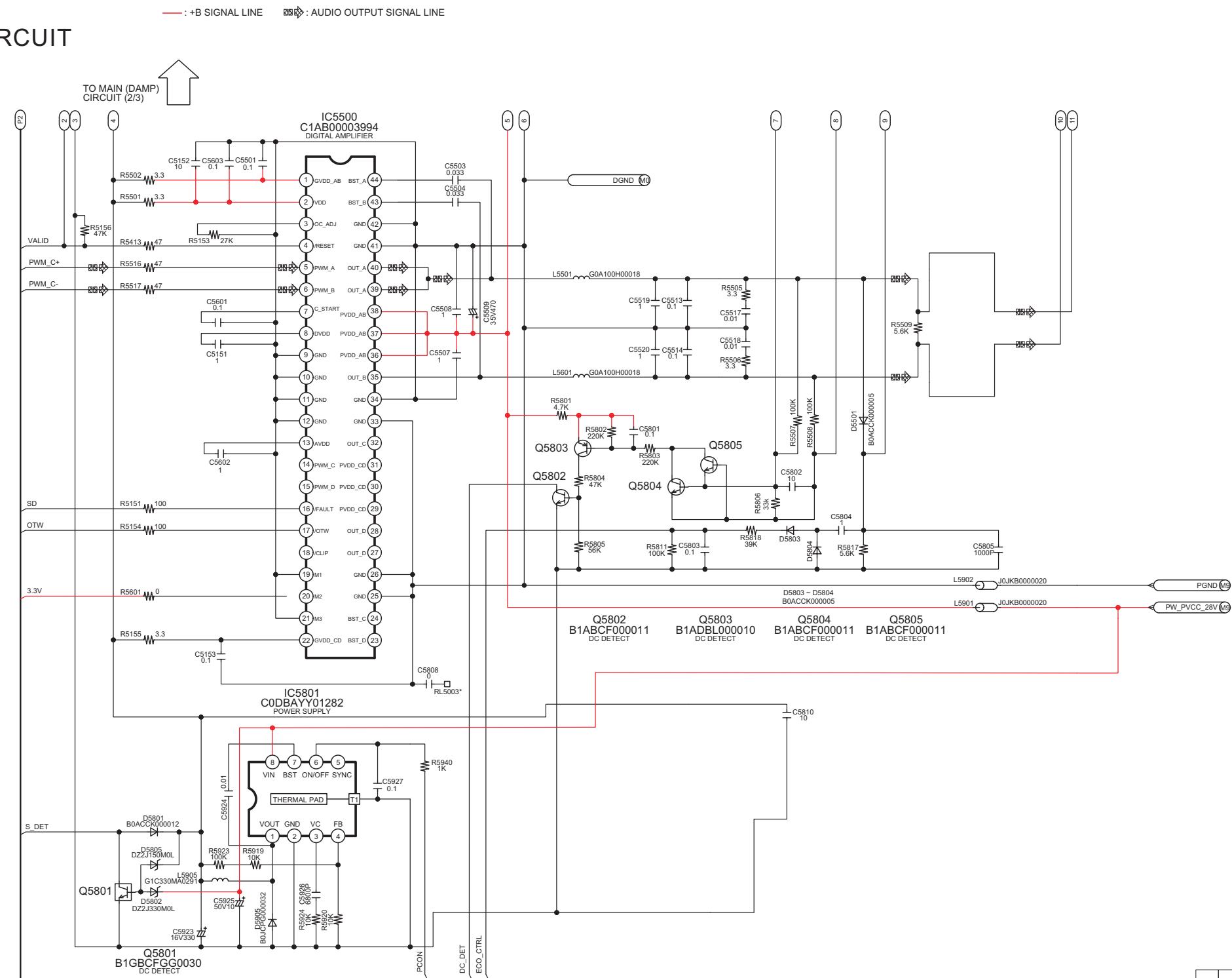
SCHEMATIC DIAGRAM - 9
