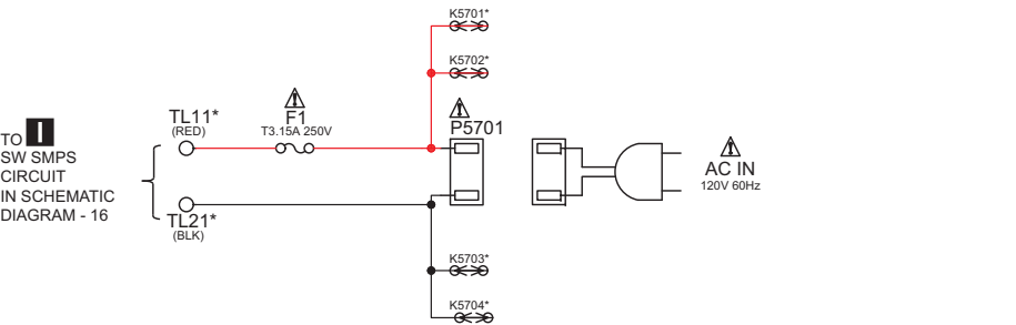
J SW AC INLET CIRCUIT
