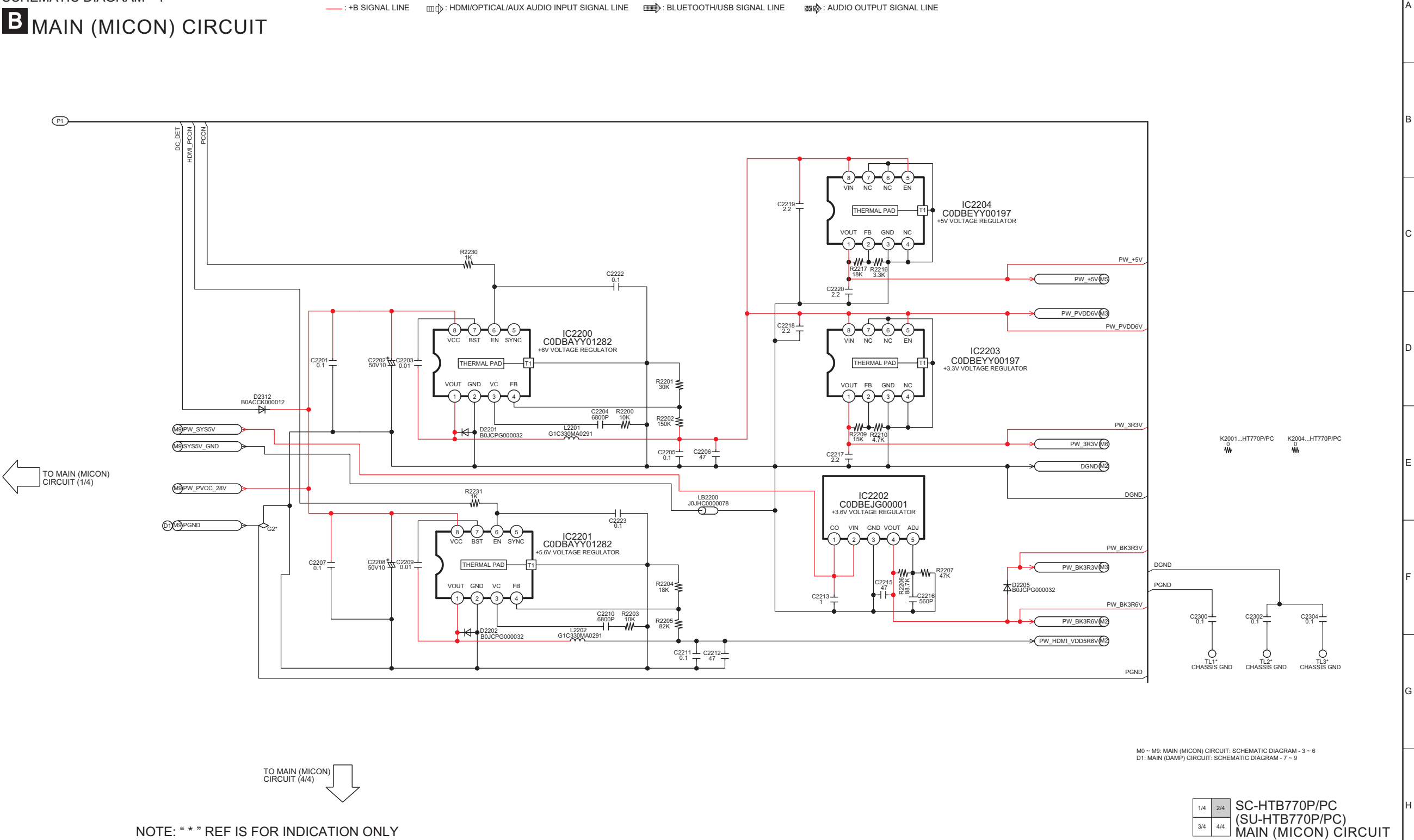
SCHEMATIC DIAGRAM - 4
