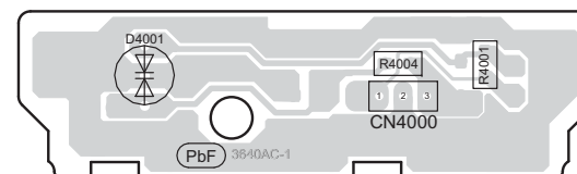
H SW LED P.C.B. (REP4869AC)
