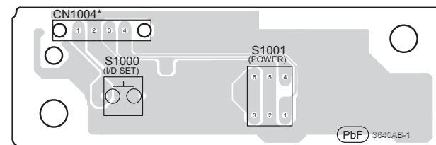
G SW POWER BUTTON P.C.B. (REP4869AB)
