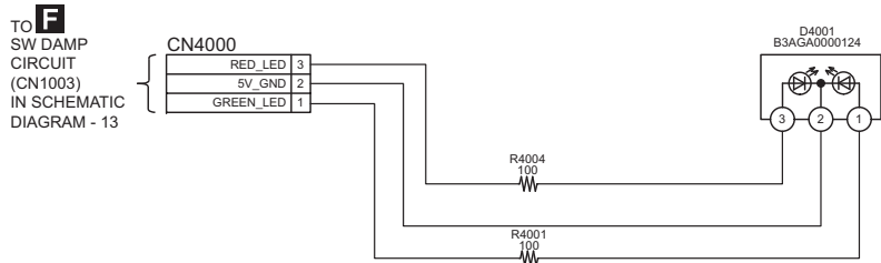
H SW LED CIRCUIT
