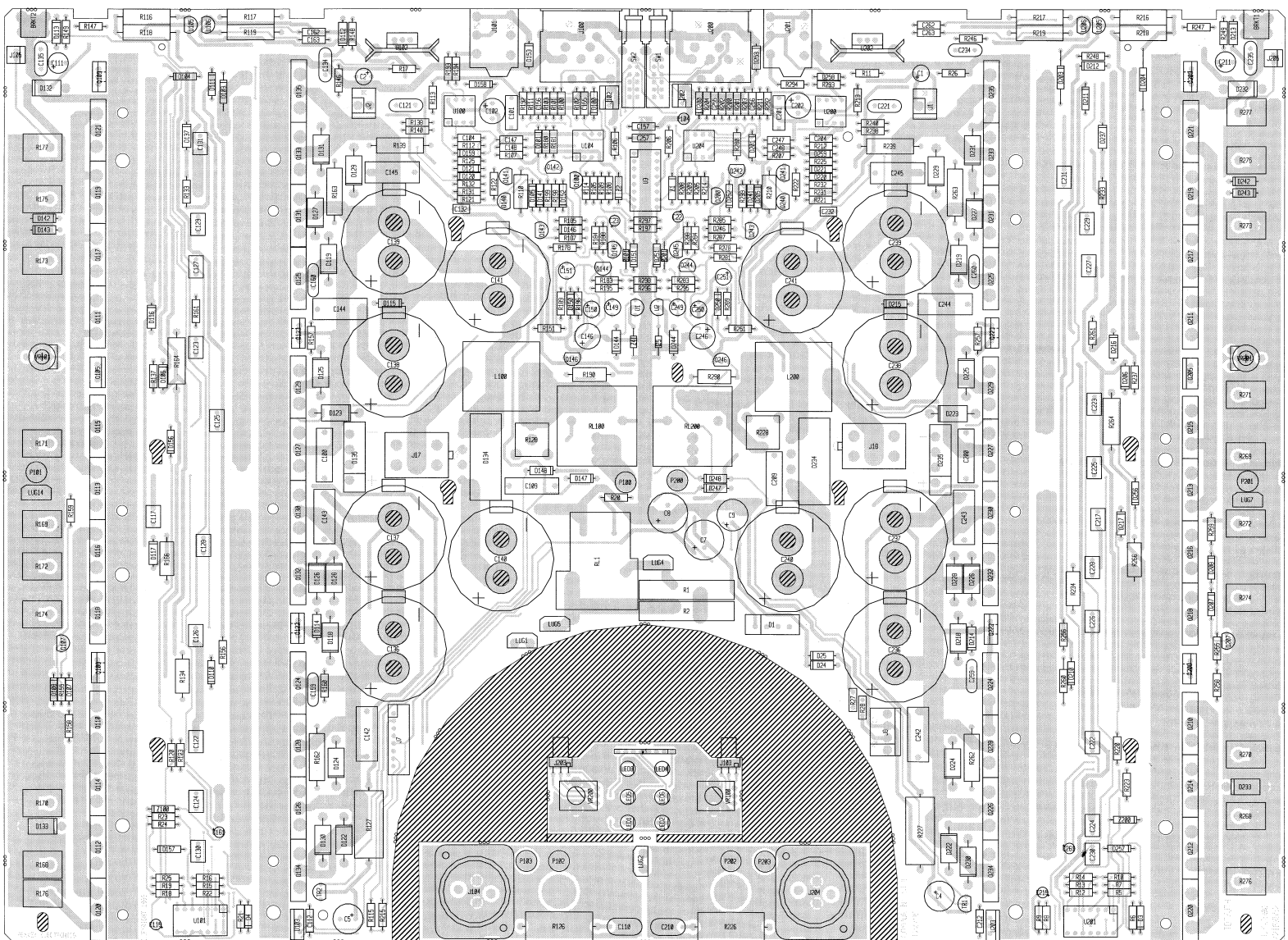
LAYER 1 COMPONENT SIDE
