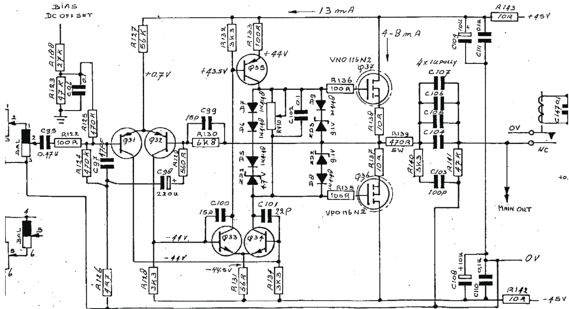
SM 2 PRE A Schematic © Perreux Indust
