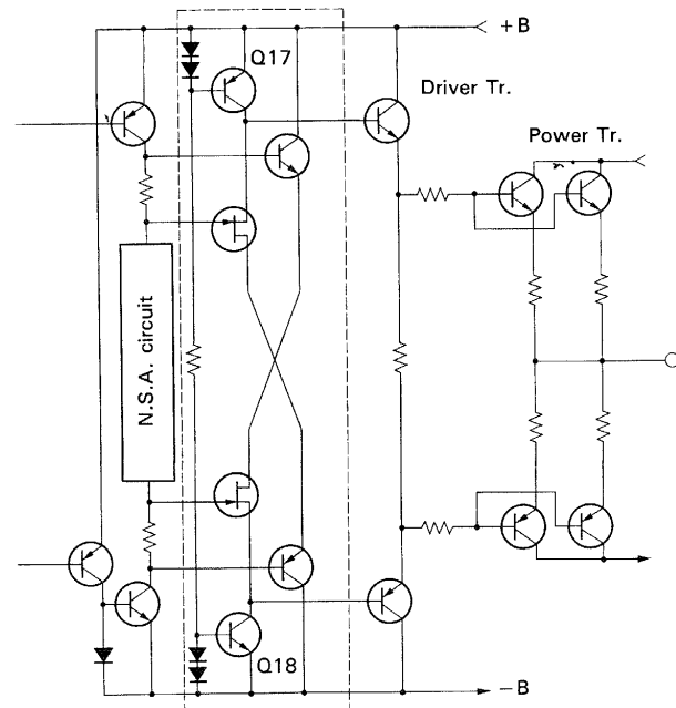
Fig. 33 Buffer circuits in A-90
