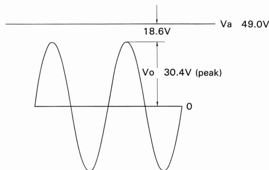
Fig. 10-b Output and power supply waveforms when DPS starts working
