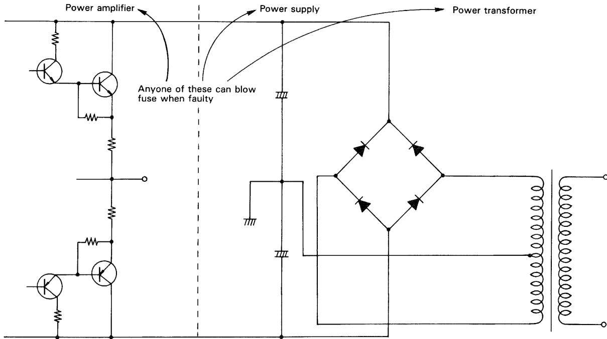
Fig. 77 Causes of blowing power fuse
