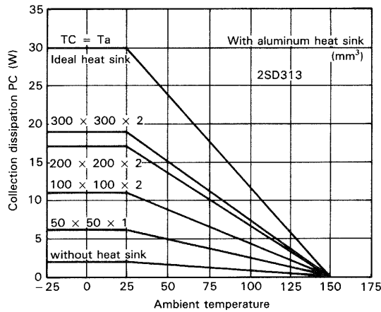
Fig. 60 Ambient temperature versus allowable collector dissipation (Pc)
