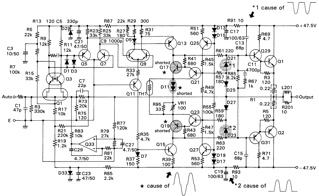
Fig. 96 Suspected components in the case output distorts
