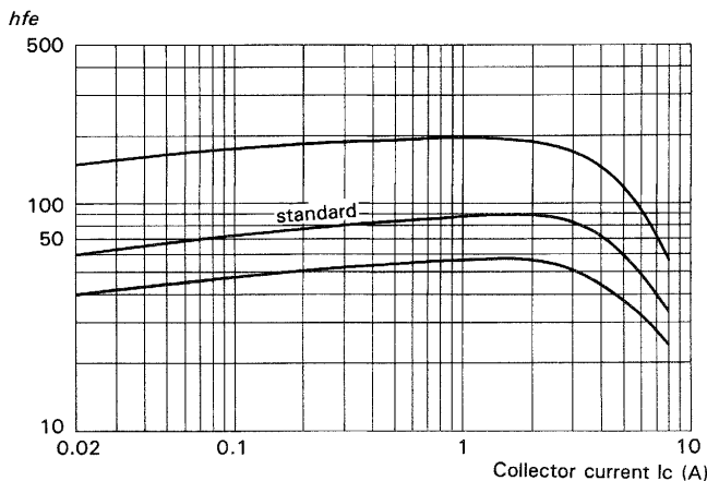
Fig. 32 hfe versus I_c characteristic
