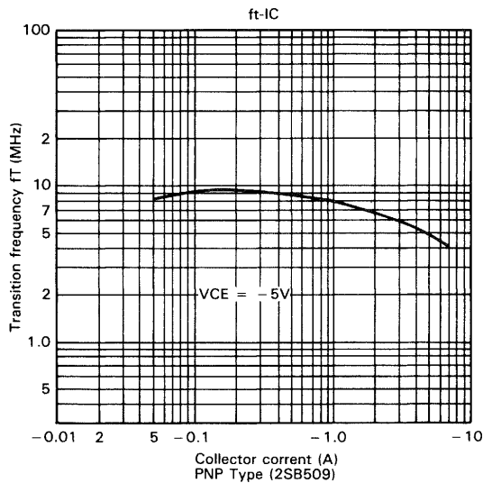
Fig. 56 f_T-I_C characteristics
