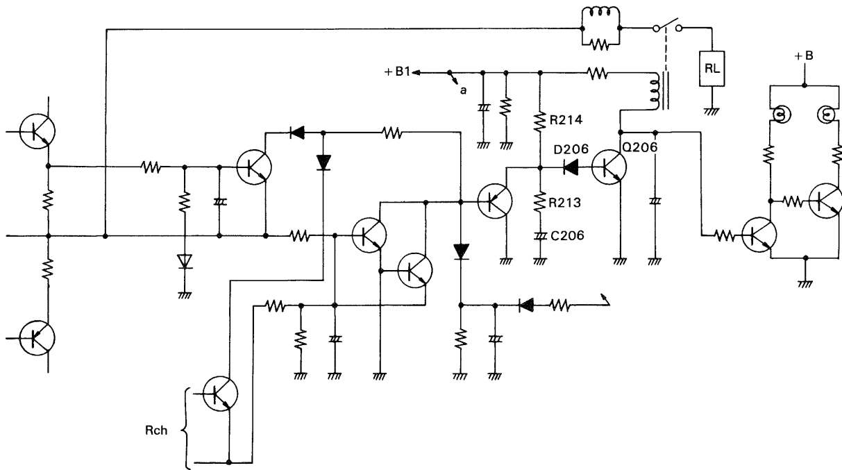
Fig. 100 Protection circuit
