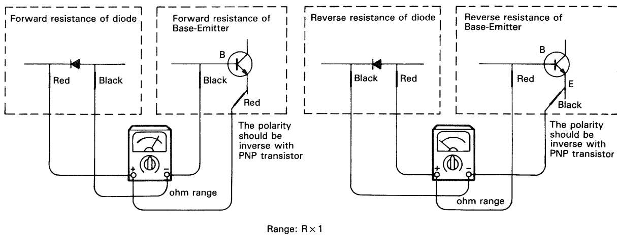
Fig. 73 Continuity test of transistors and diodes
