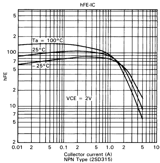
Fig. 55 h_{FE}-I_C characteristic
