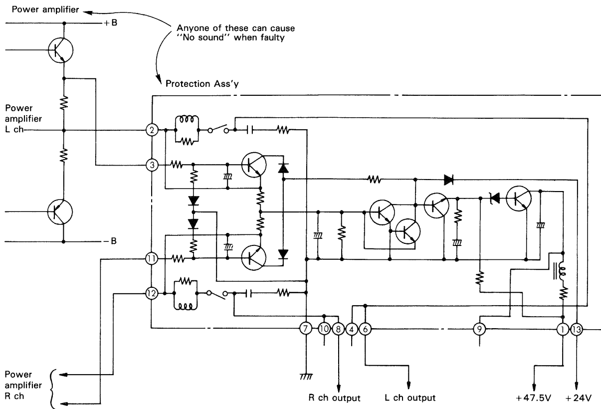
Fig. 78 Causes of no sound
