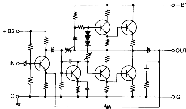
Fig. 2 Standard Single-Ended Push-Pull Amplifier
