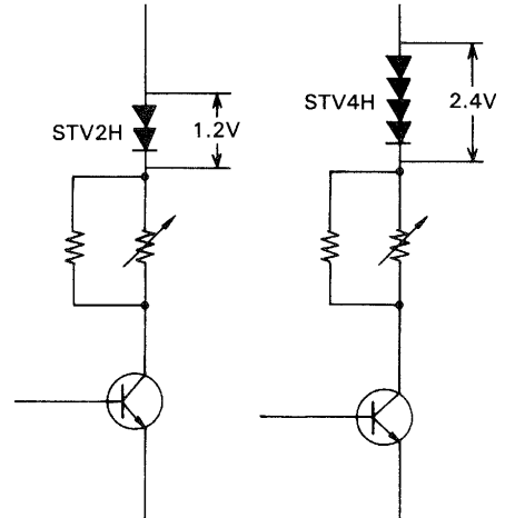
Fig. 75 Checking varistor (2)
