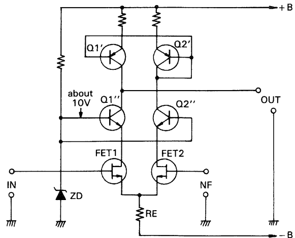
Fig. 53 Input stage circuit employing FETs.
