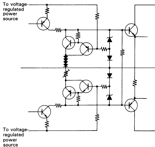
Fig. 27 Fed from voltage regulated power source
