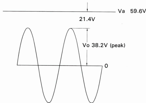
Fig. 11-b Output and power supply waveforms when speakers are disconnected
