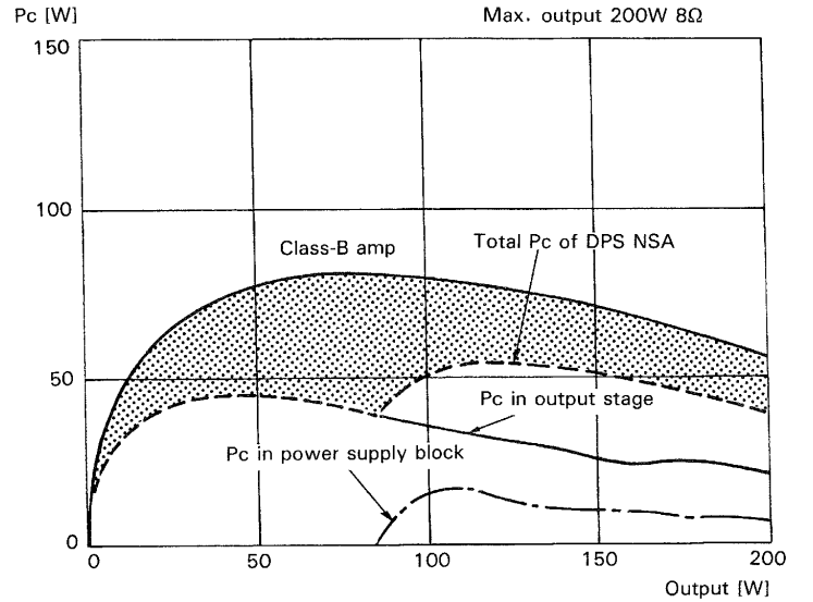
Fig. 5 Output power VS. dissipation
