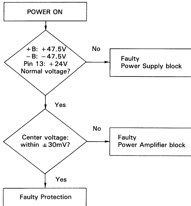
Fig. 81 Finding faulty block
