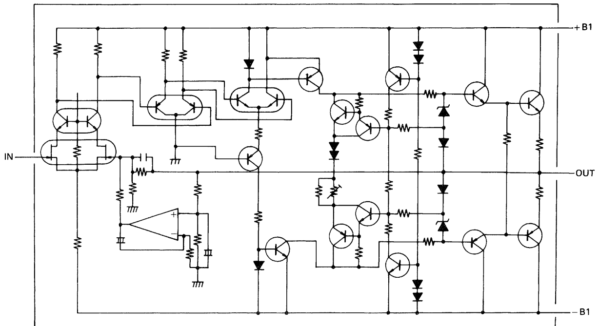
Fig. 6 Non-Switching Amplifier (with DC servo circuit)
