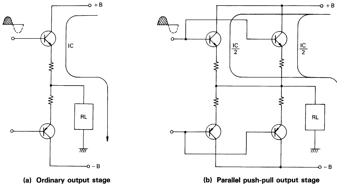
Fig. 54 Output circuit
