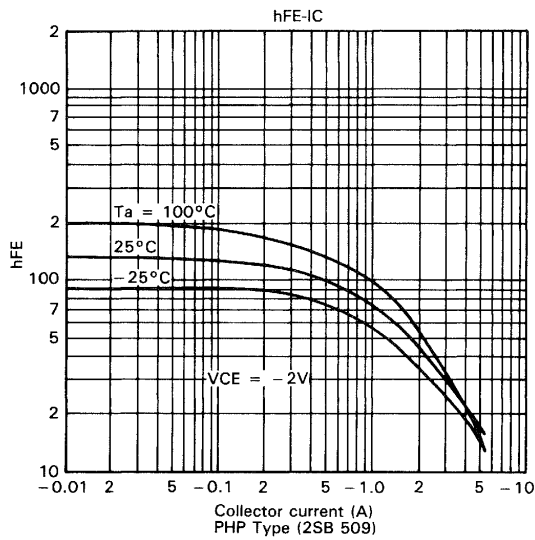
Fig. 55 h_{FE}-I_C characteristic
