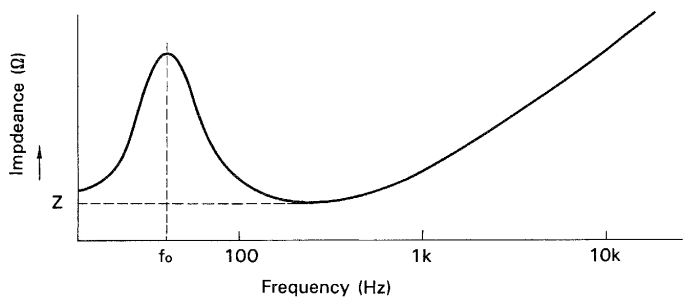
Fig. 31 Impedance characteristic of a bass reflex type speaker system
