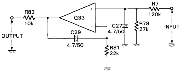
Fig. 30 DC servo circuit
