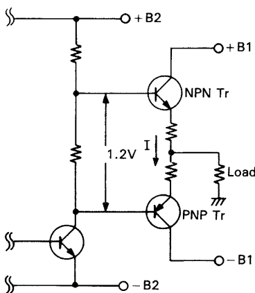
Fig. 16 Bias setting for idle current
