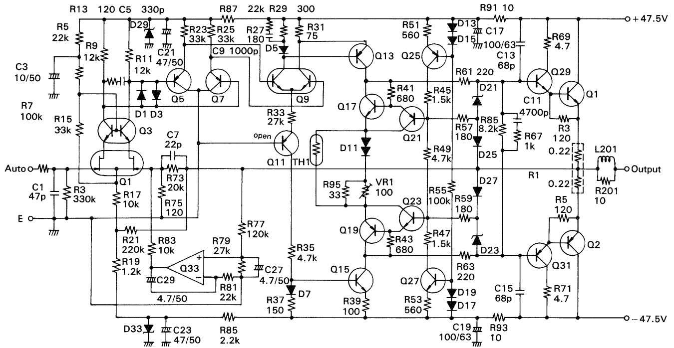
Fig. 93 Suspected components of "No sound although Protection Relay turns on."
