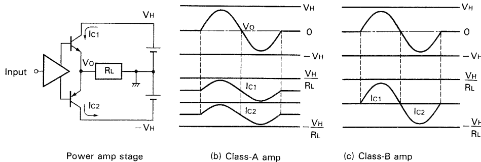
Fig. 3 Voltage (current) waveforms of class-A and class-B amplifiers
