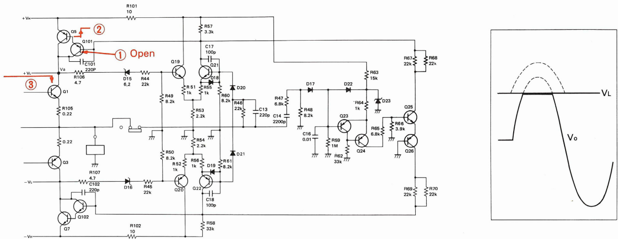
Fig. 23 V_o is clipped when Q101 opens
