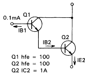
Fig. 50 Current of Darlington circuit
