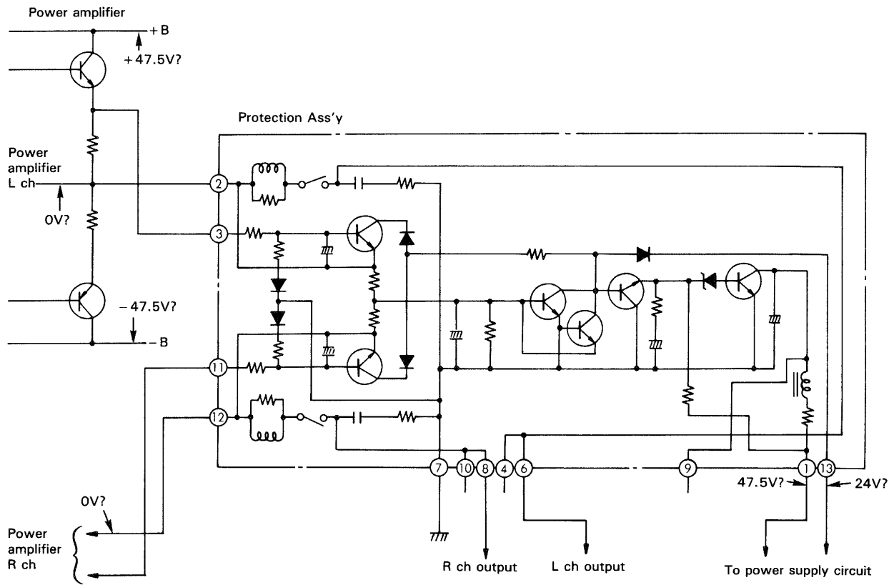
Fig. 80 Finding faulty block – No sound
