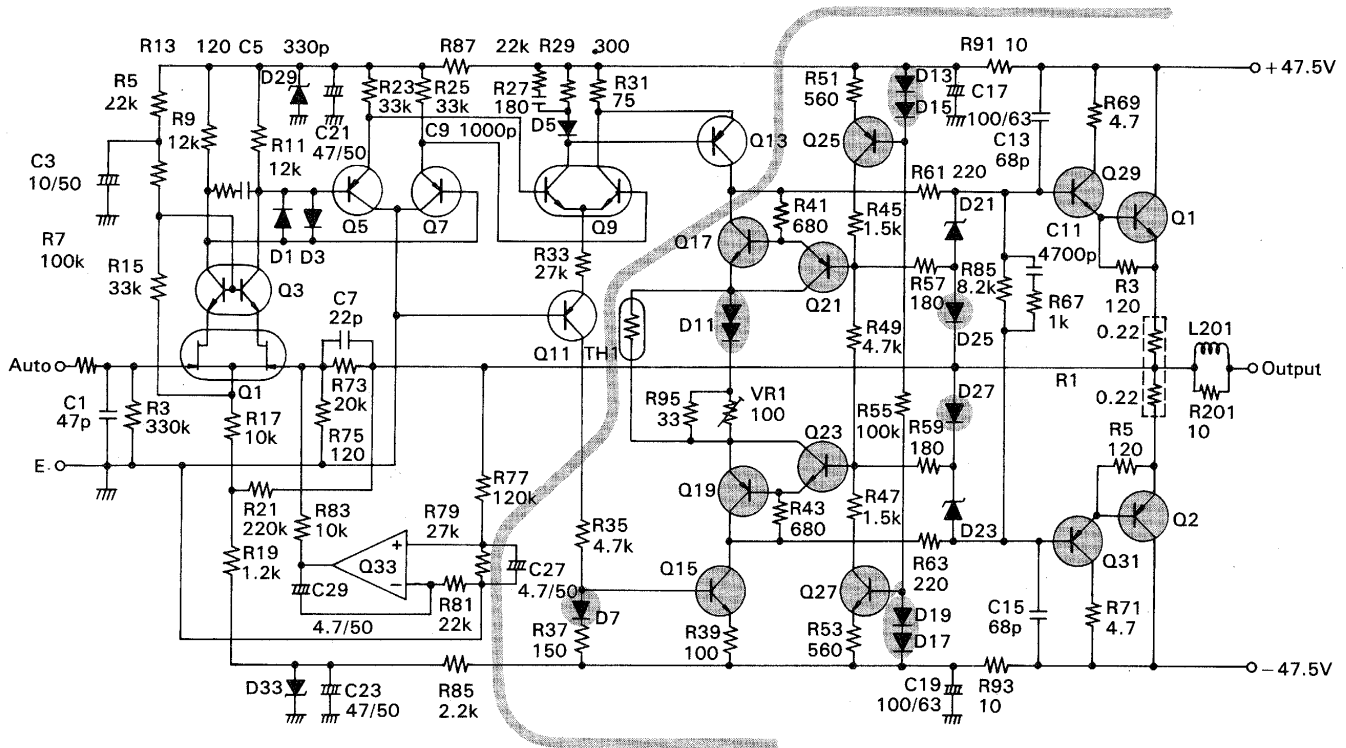
Fig. 85 Suspected components when fuse blows
