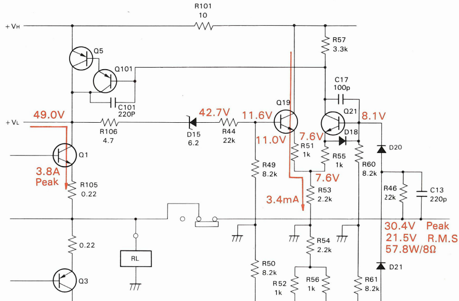
Fig. 10-a Voltage, current and waveforms when DPS starts working
