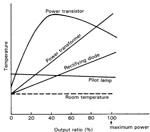
Fig. 59 Output ratio versus temperature rise
