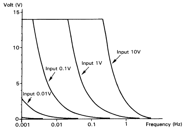
Input/Output characteristics of DC Servo Circuit
