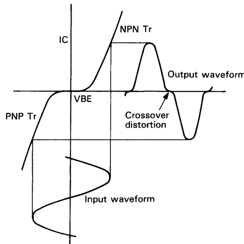
Fig. 14 Biasing in class-B mode
