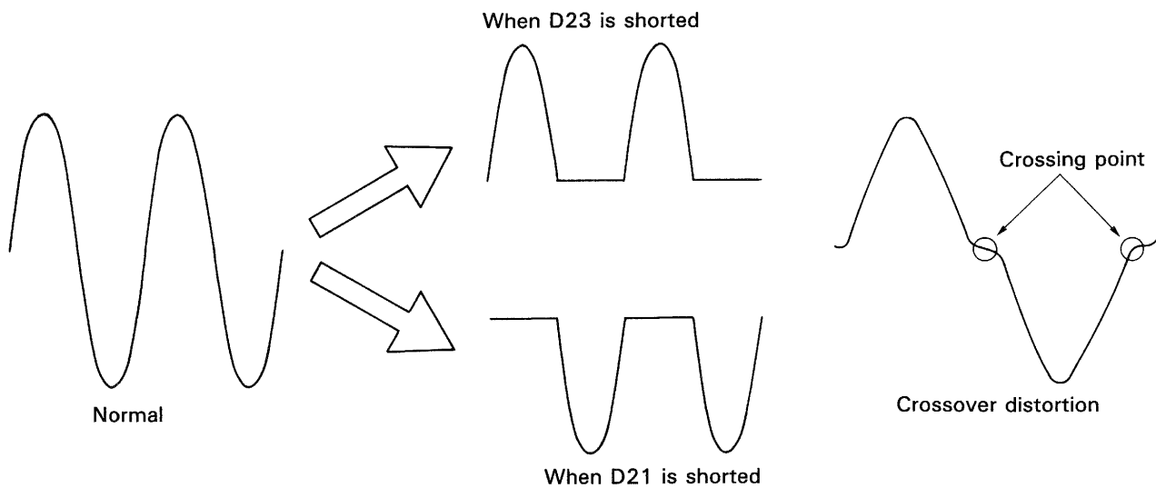
Fig. 95 Output waveform
