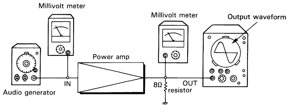
Fig. 87 Final check after repairing
