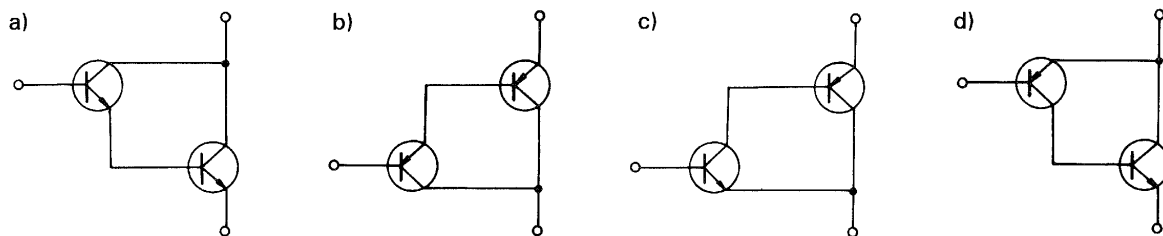
Fig. 49 Darlington connection
