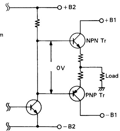
Fig. 15 Generation of crossover distortion
