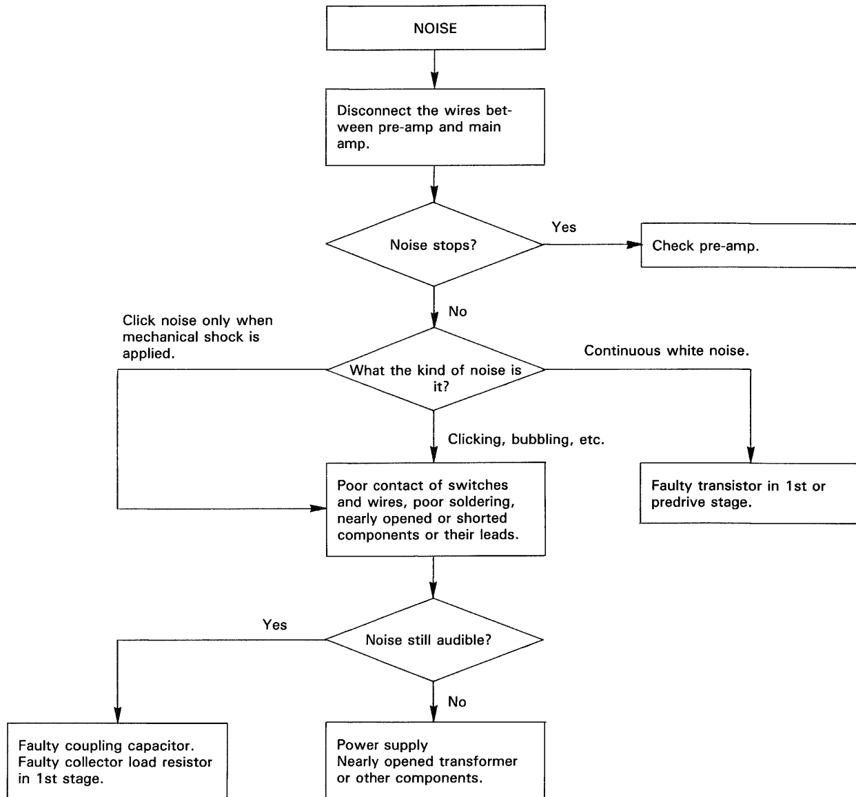
Fig. 99 Troubleshooting chart
