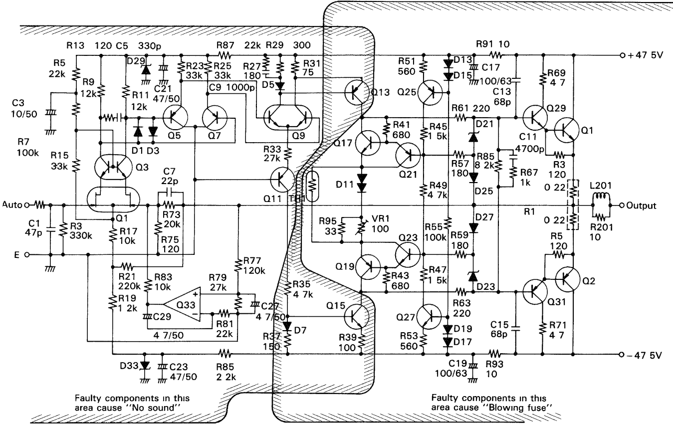
Fig. 83 Suspected area for each trouble
