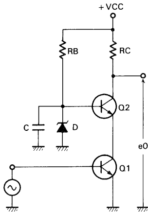
Fig. 37 Cascode amplifier
