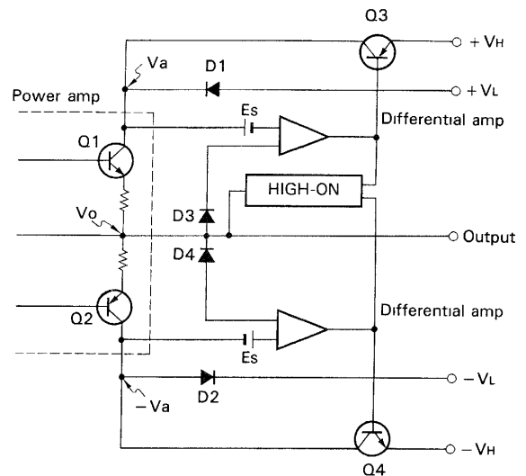
Fig. 6 Simplified circuit of DPS system
