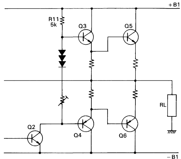
Fig. 45 Power Amplifier without bootstrap circuit
