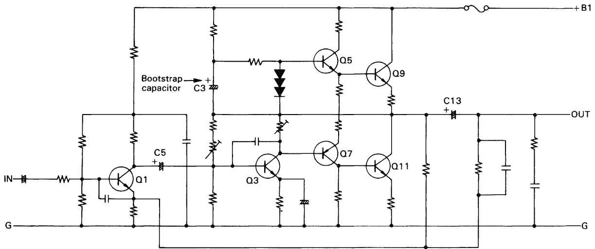
Fig. 7 Standard SEPP Amplifier
