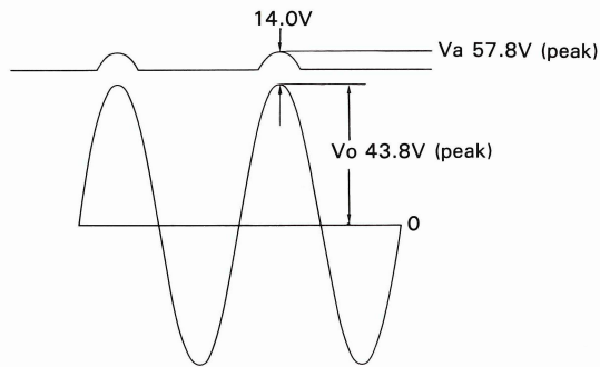
Fig. 13-b Output and power supply voltage waveforms
