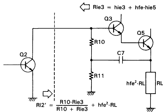
Fig. 48 Load of Q 2 with bootstrap circuit
