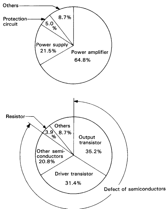
Fig. 58 Pie charts for faulty blocks and components
