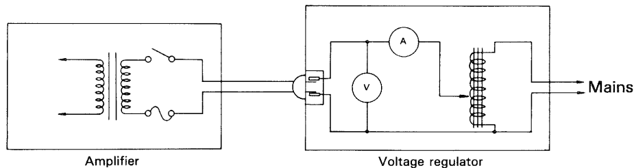
Fig. 82-a Detecting excessive current with a voltage regulator
