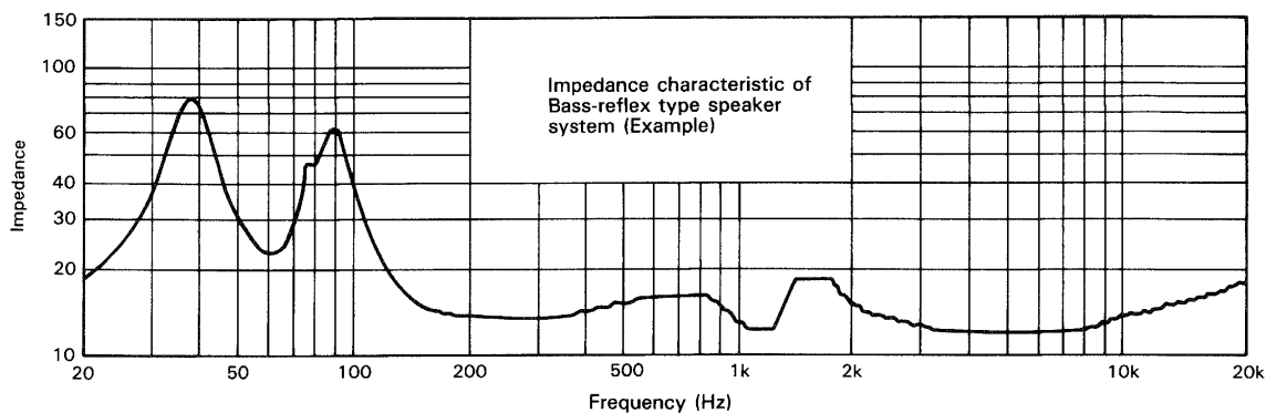
Fig. 69 Impedance characteristics of 3 way bass-reflex type speaker systems
