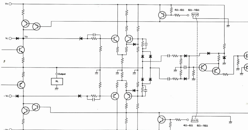
Fig. 24 A-70 Dynamic power supply circuit
