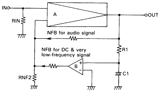
Fig. 29 Basic operation of amplifier with DC servo circuit
