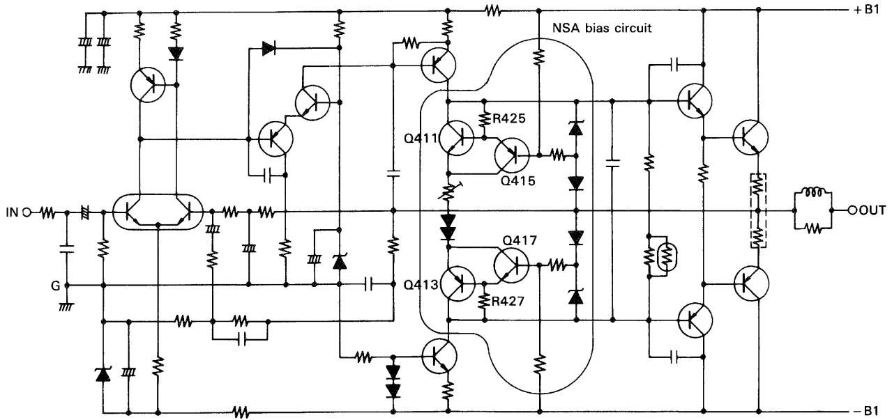
Fig. 11 Non-Switching Amplifier
