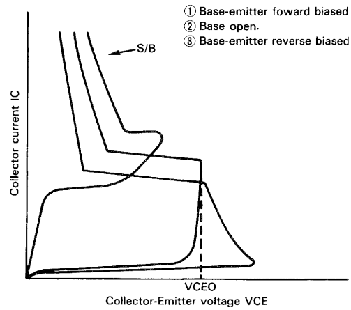
Fig. 65 Secondary breakdown of common emitter circuit
