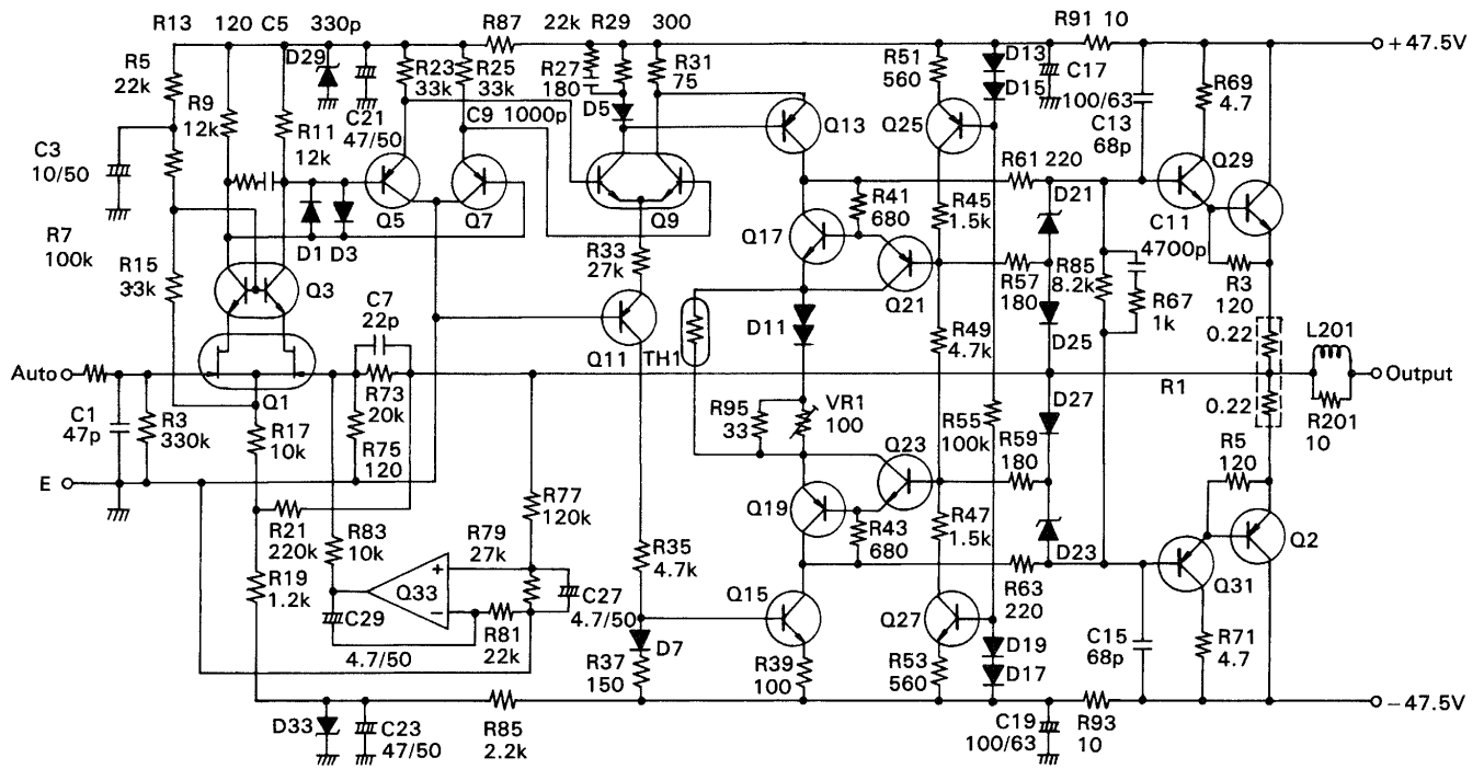
Fig. 103 Suspected components in the case amplifier becomes hot
