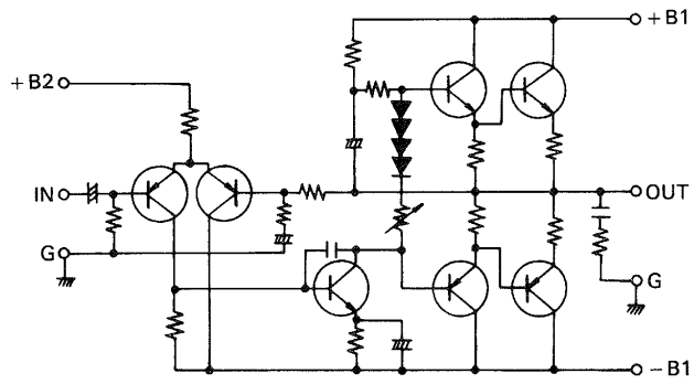
Fig. 3 All-Stage Direct-Coupled SEPP Amplifier
