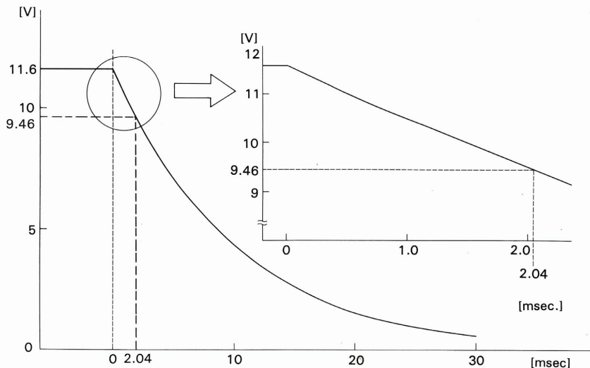
Fig. 19-b Discharging characteristic
