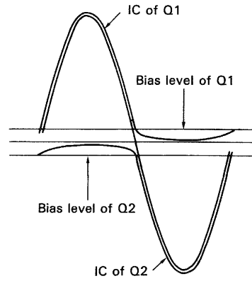
Fig. 24 Waveform of collector currents
