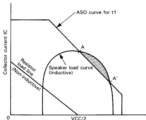
Fig. 67 Speaker load line and ASO
