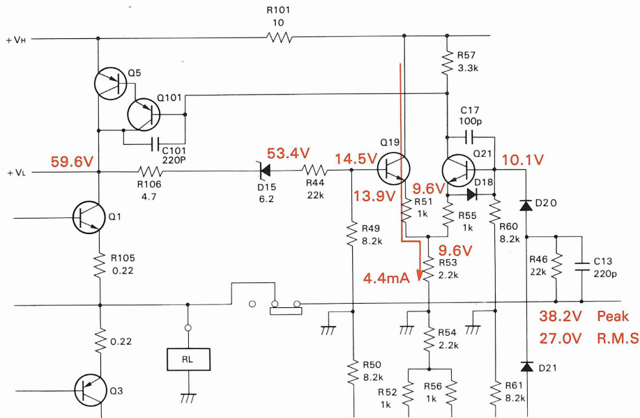
Fig. 11-a Voltage and current reading when speakers are disconnected and the output voltage is 38.2 V at the peak.
