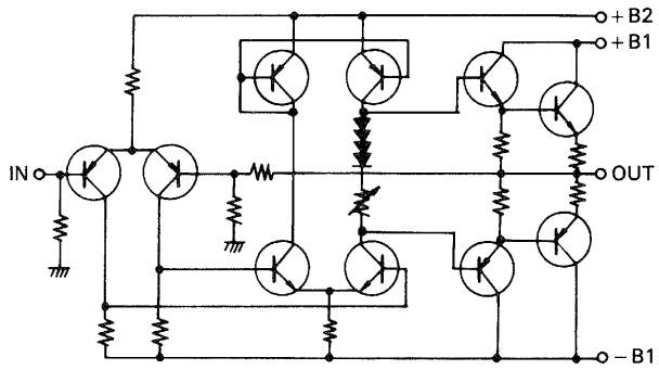
Fig. 4 All-Stage Direct-Coupled SEPP DC Amplifier
