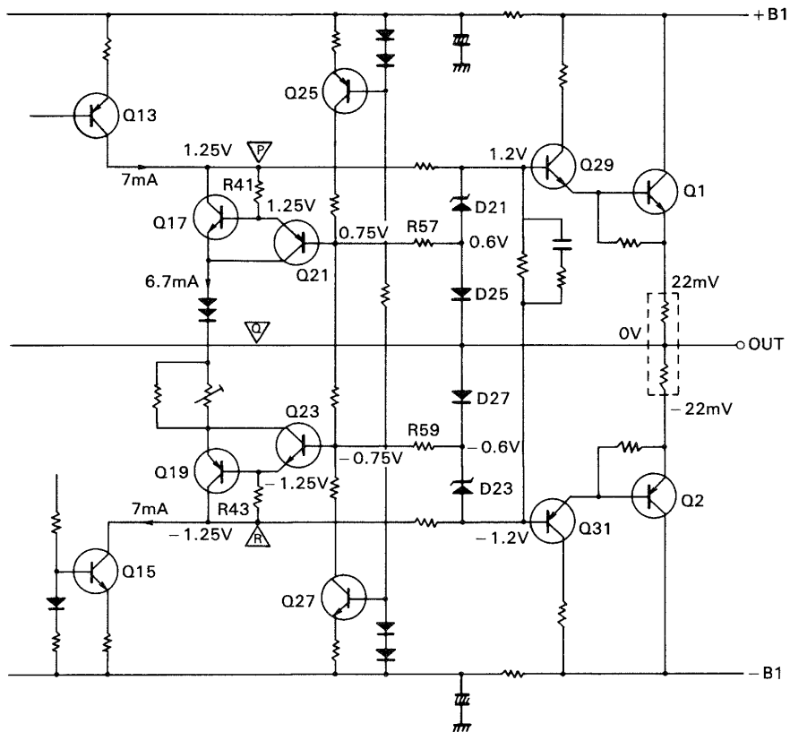
Fig. 22 Potential with no input
