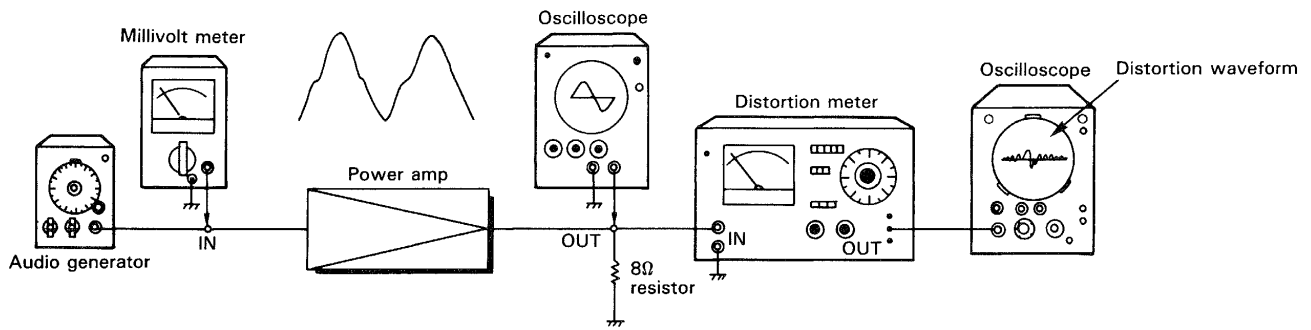
Fig. 98 Confirming output
