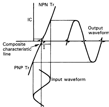
Fig. 17 Elimination of crossover distortion by flowing idle current
