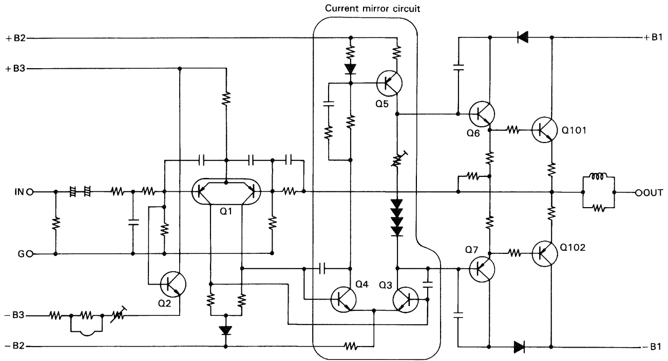
Fig. 10 All-Stage Direct-Coupled SEPP DC Amplifier
