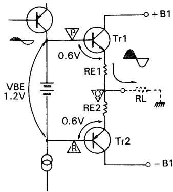
Fig. 20 Biasing of class-B Amplifier
