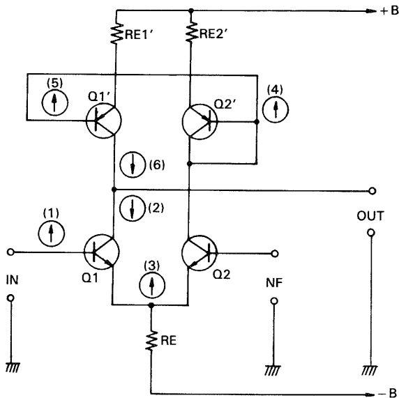
Fig. 51 Current mirror circuit in the input stage
