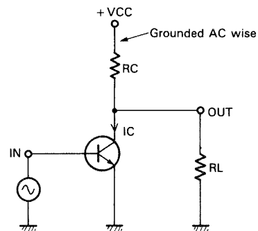
Fig. 40 Emitter-grounded amplifier
