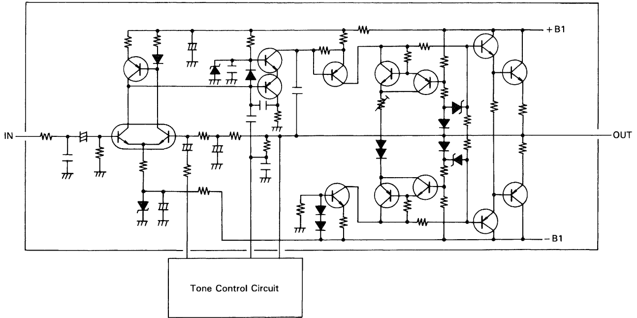
Fig. 5 Non-Switching Amplifier
