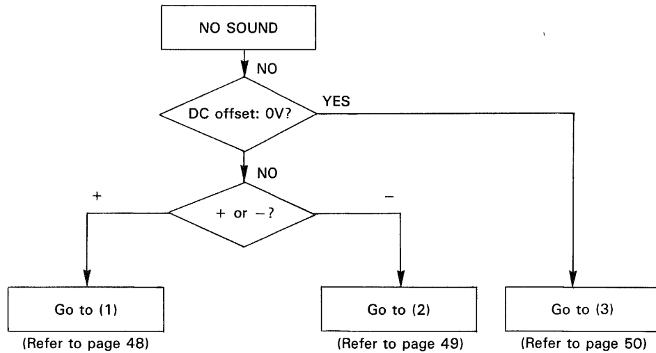
Fig. 89 Troubleshooting flowchart
