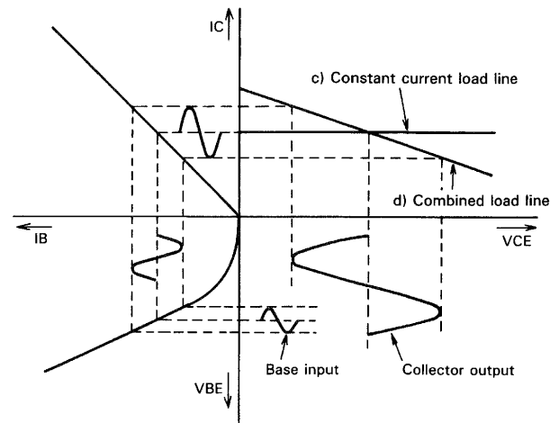
Fig. 43 Characteristics with constant-current load
