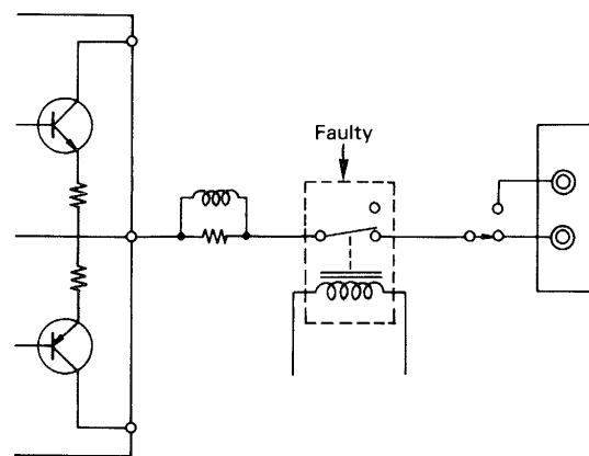
Fig. 101 Faulty component
