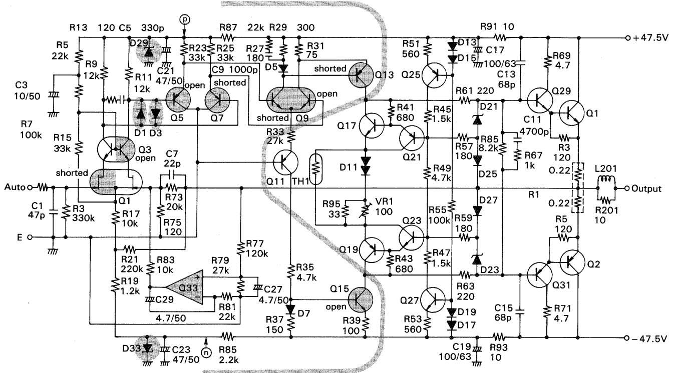
Fig. 90 Suspected components in the case DC offset voltage is positive.
