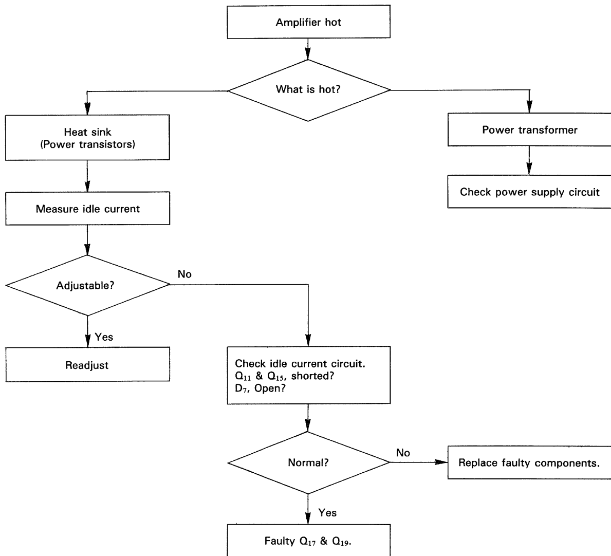
Fig. 102 Troubleshooting chart
