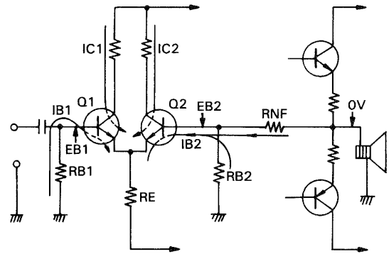
Fig. 52 1st-stage of All-stage Direct-coupled DC Amplifier
