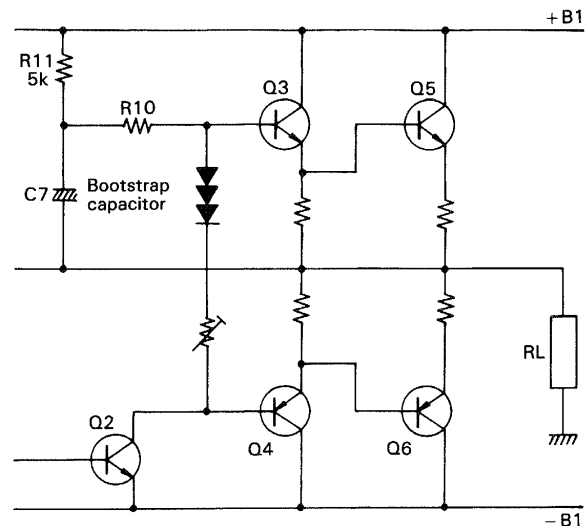
Fig. 46 Power Amplifier with bootstrap circuit. Refer to Fig. 48.
