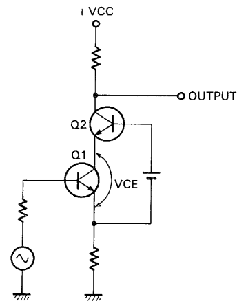
Fig. 39 V_{CE} setting of cascode amplifier
