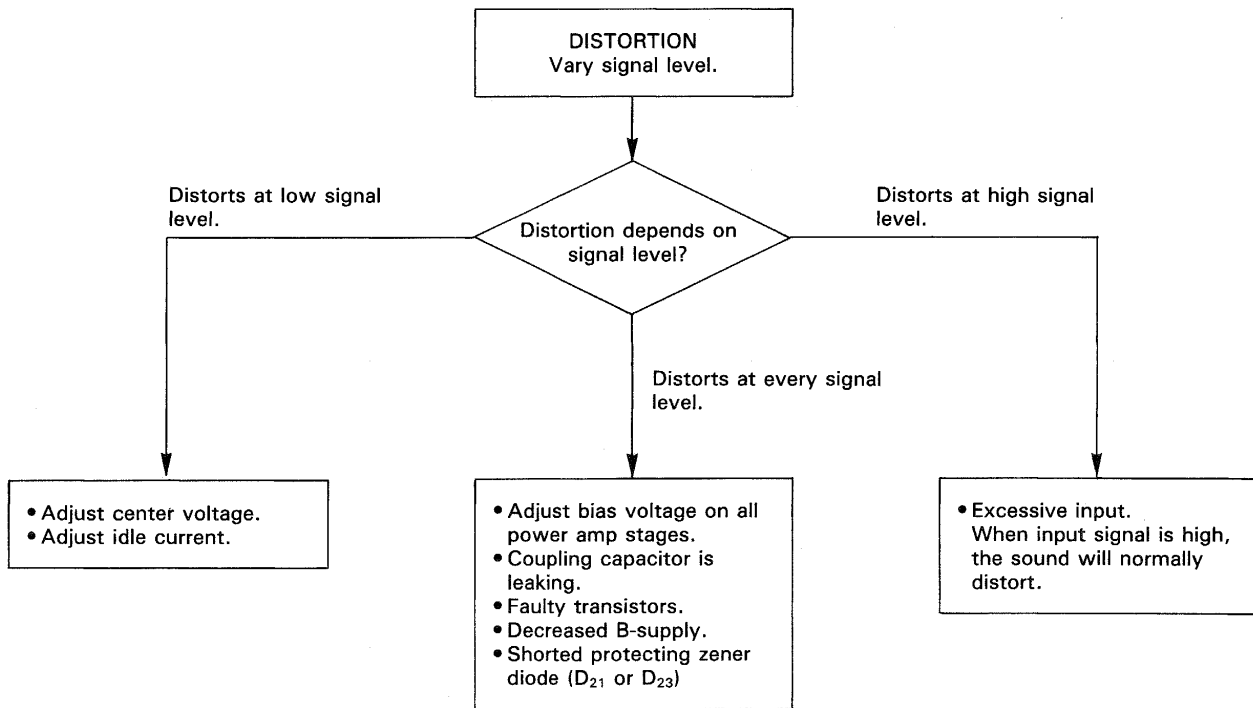
Fig. 97 Troubleshooting chart
