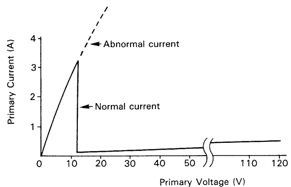
Fig. 82-c Primary voltage vs primary current
