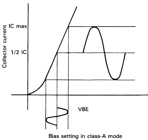
Fig. 13 Bias setting in class-A mode
