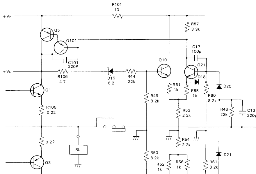
Fig. 7 DPS circuit of A-80
