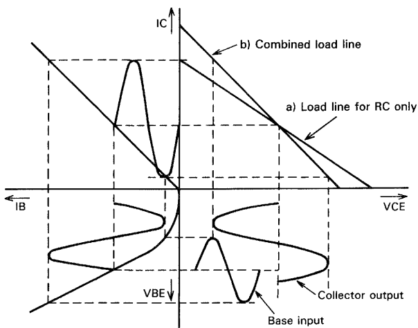
Fig. 42 Characteristics with ordinary resistor load
