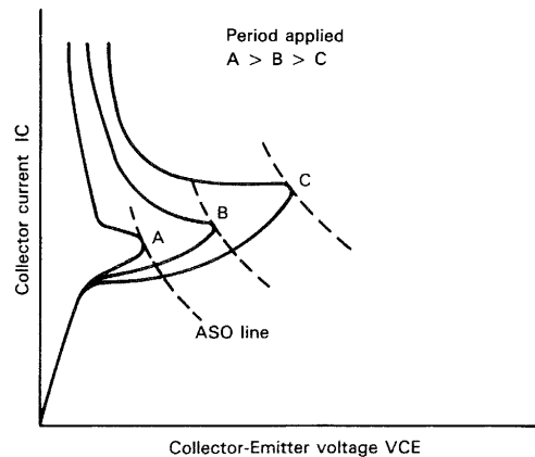
Fig. 66 Secondary breakdown point depends on the period the voltage applied.
