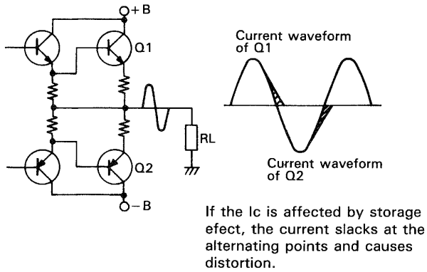
Fig. 63 Wave deformed by storage effect of electron
