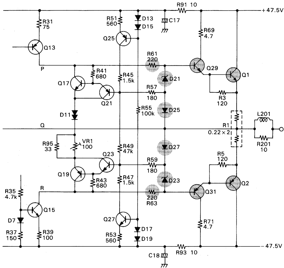
Fig. 86 Components liable to be damaged
