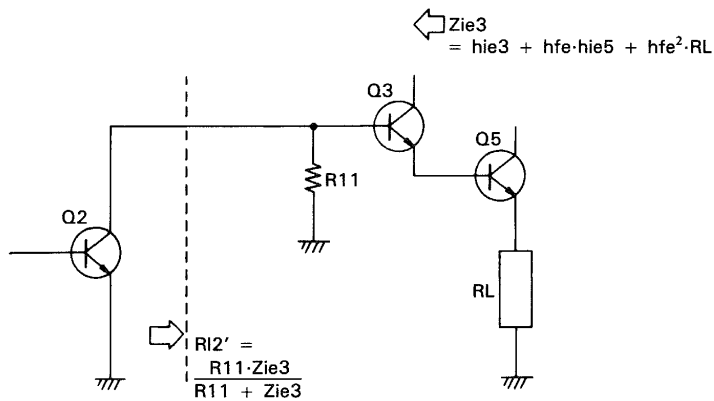
Fig. 47 Load of Q 2 without bootstrap circuit
