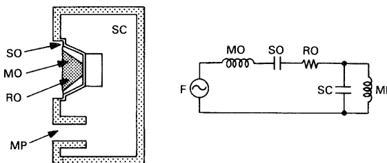
Fig. 68 Equivalent circuit of a single-cone speaker in bass-reflex type enclosure
