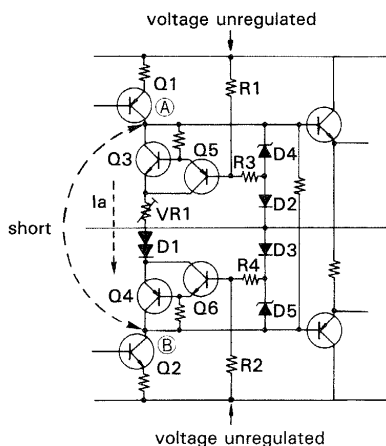
Fig. 82-b NSA bias circuit
