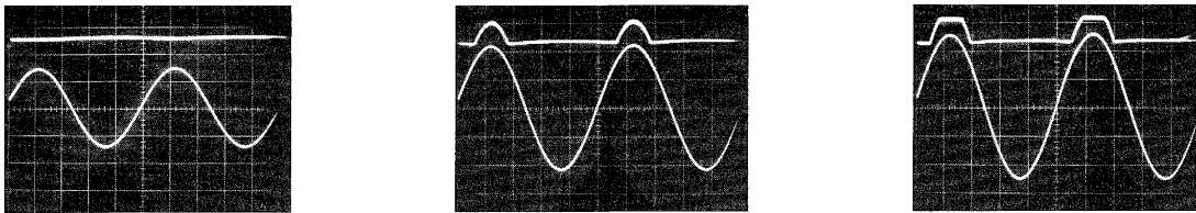
Photo 3 Supply voltage made by Differential Detector
