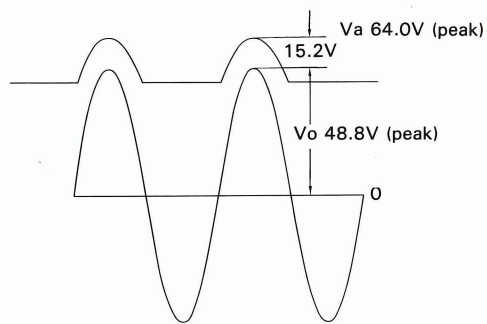
Fig. 12-b Output and power supply voltage waveforms
