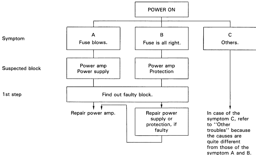
Fig. 76 Confirmation of defect
