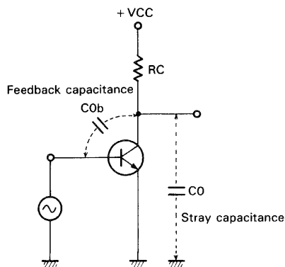
Fig. 38 Existence of equivalent capacitance
