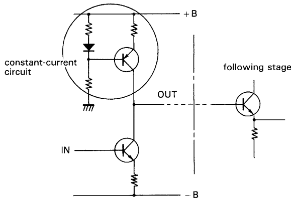
Fig. 44 Amplifying circuit with constant-current load
