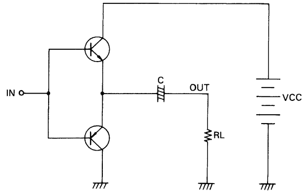
Fig. 1 SEPP circuit
