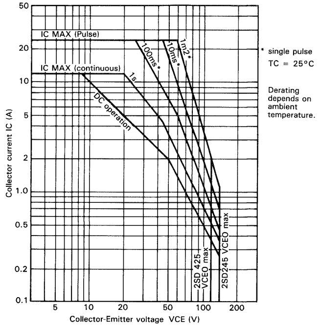
Fig. 64 ASO characteristic of power transistor
