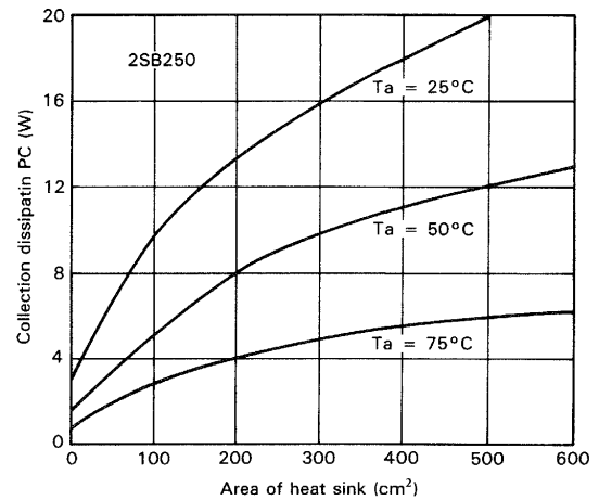
Fig. 61 Area of heat sink versus collector dissipation
