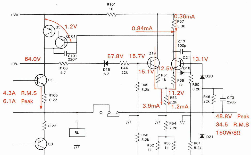
Fig. 12-a Voltage and current reading when producing 150W signals
