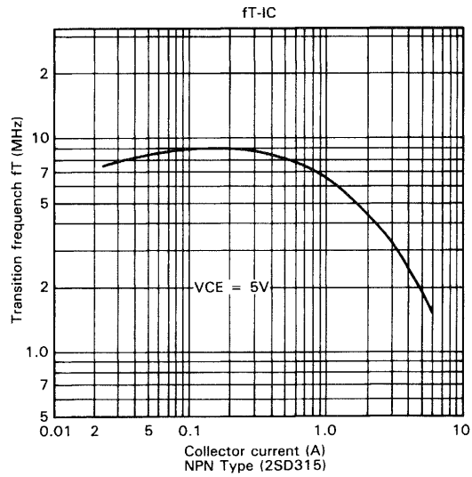
Fig. 56 f_T-I_C characteristics
