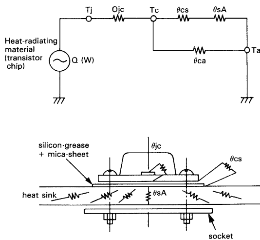
Fig. 62 Thermal resistance in the radiating route
