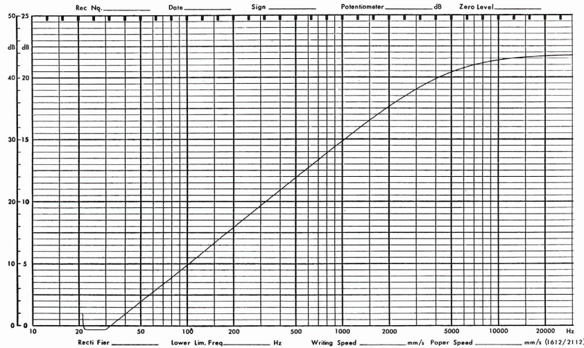
Fig. 16 Characteristic of High-pass filter
