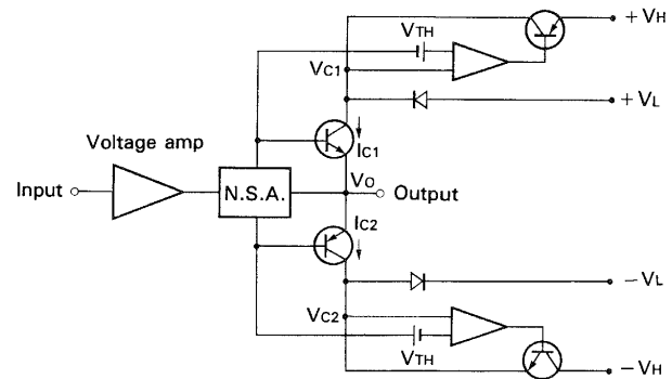
Fig. 2 Simplified diagram of DPS system
