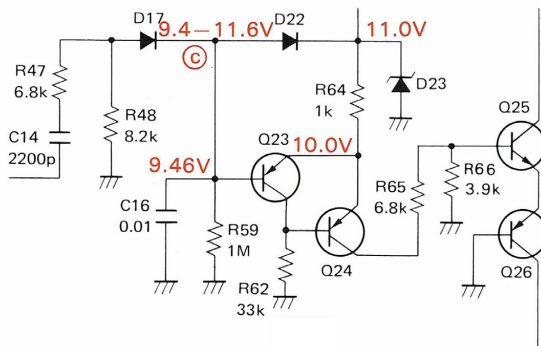
Fig. 19-a HIGH-ON circuit
