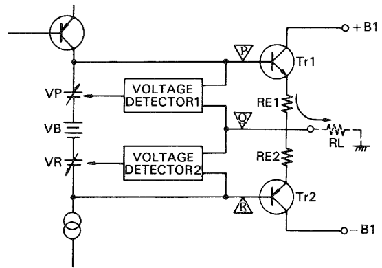
Fig. 21 Biasing of Non-Switching Amplifier
