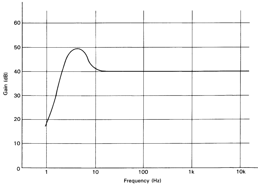
Fig. 9 Frequency response of standard SEPP amplifier
