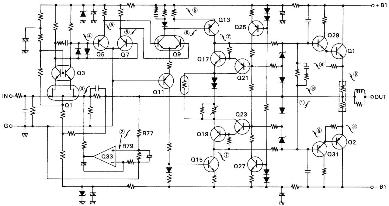
Fig. 34 Operation of DC servo circuit
