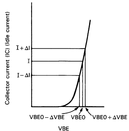
Fig. 18 Idle current setting
