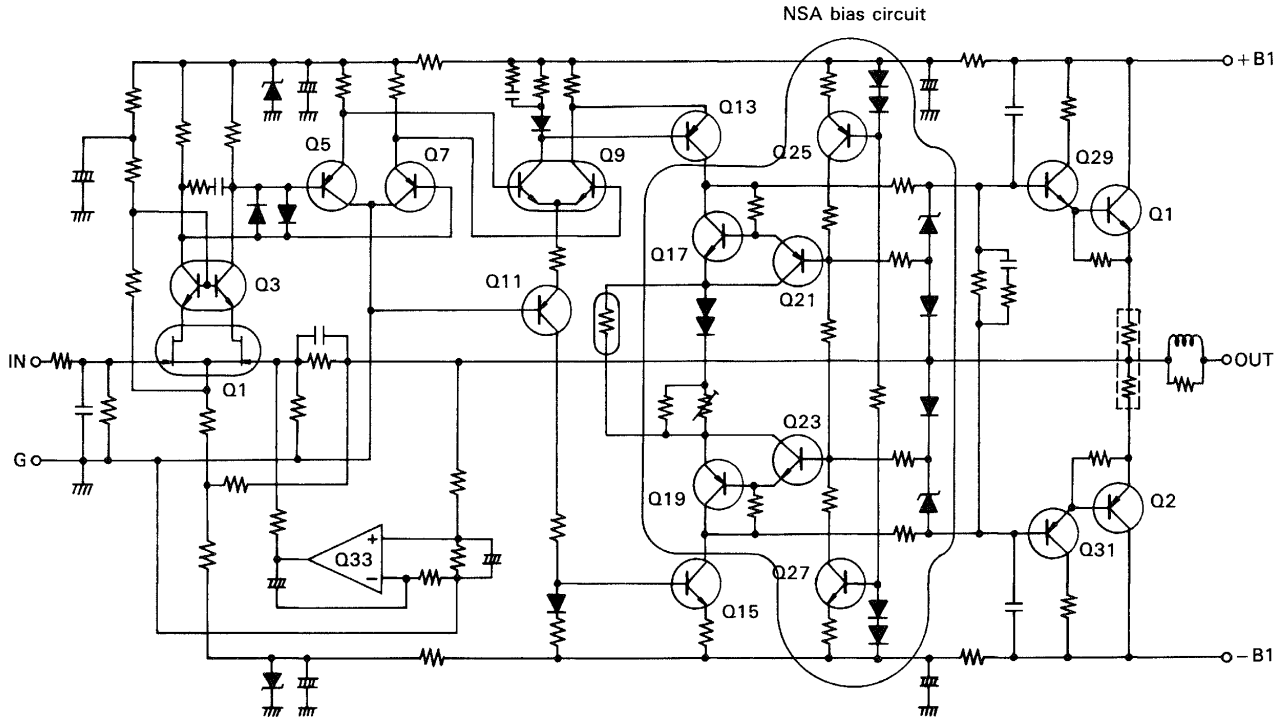
Fig. 12 Non-Switching Amplifier (with DC servo circuit)
