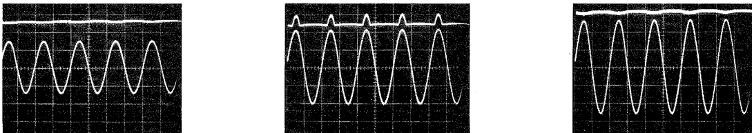
Photo 5 Operation of Differential circuit and HIGH-ON circuit
