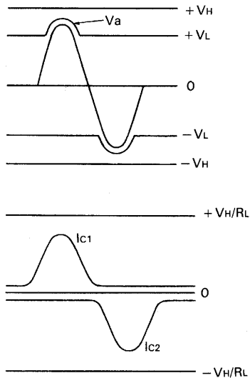
Fig. 4 Voltage (current) waveforms of DPS NSA.
