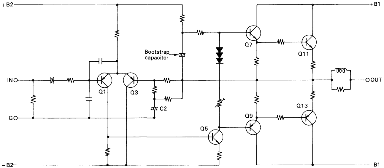
Fig. 8 All-Stage Direct-Coupled SEPP Amplifier
