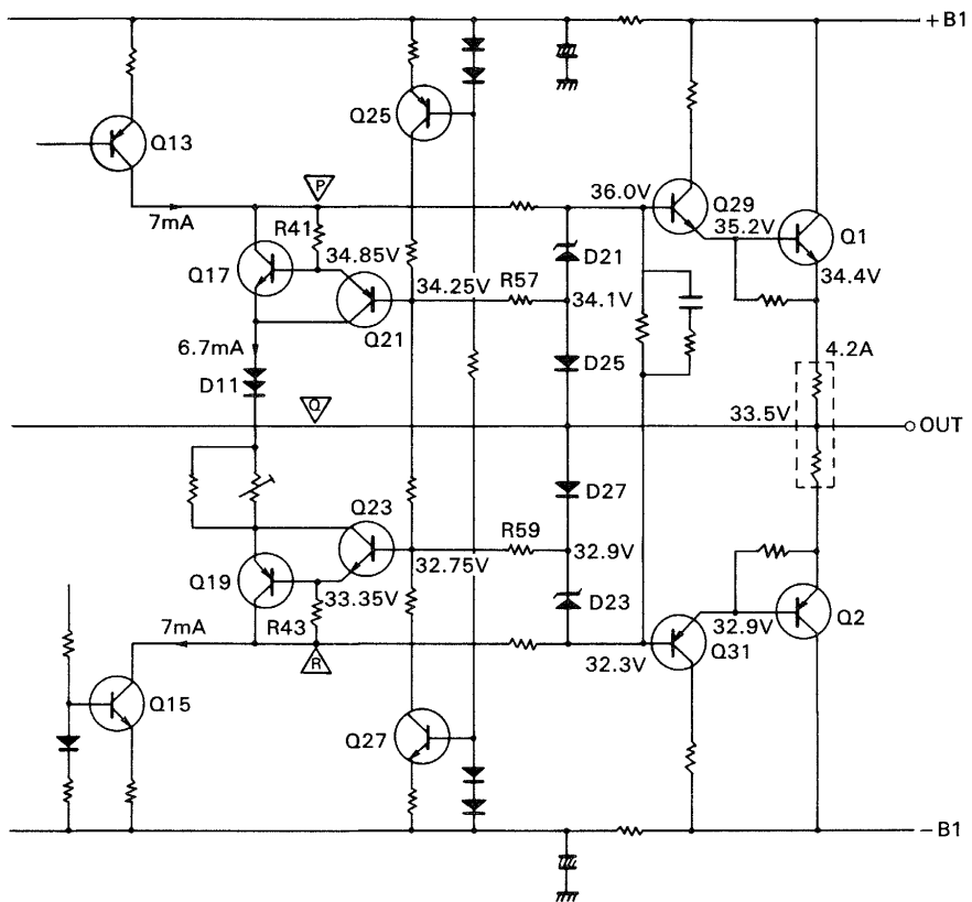
Fig. 23 Momentary potential at positive peak, 70W output
