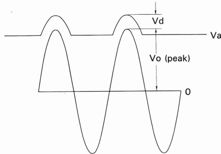
Fig. 8 When V_o becomes high
