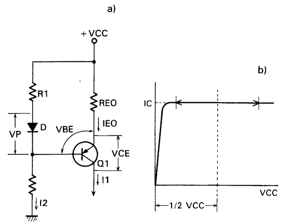
Fig. 41 V_{CC} - I_C Constant-current circuit and characteristic
