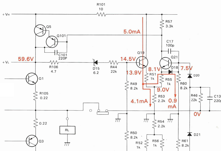
Fig. 9 Voltage and current values at each point
