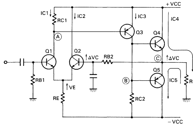
Fig. 36 Operation of DC offset cancellation
