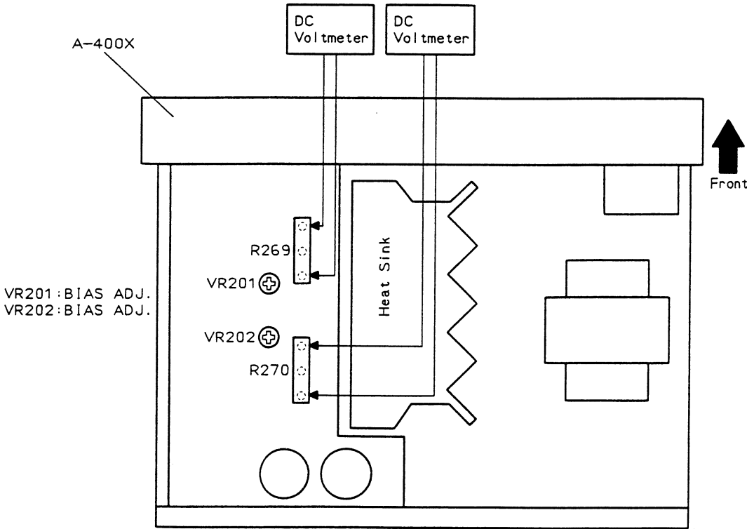
Fig. 6-1 Adjustment Drawing
