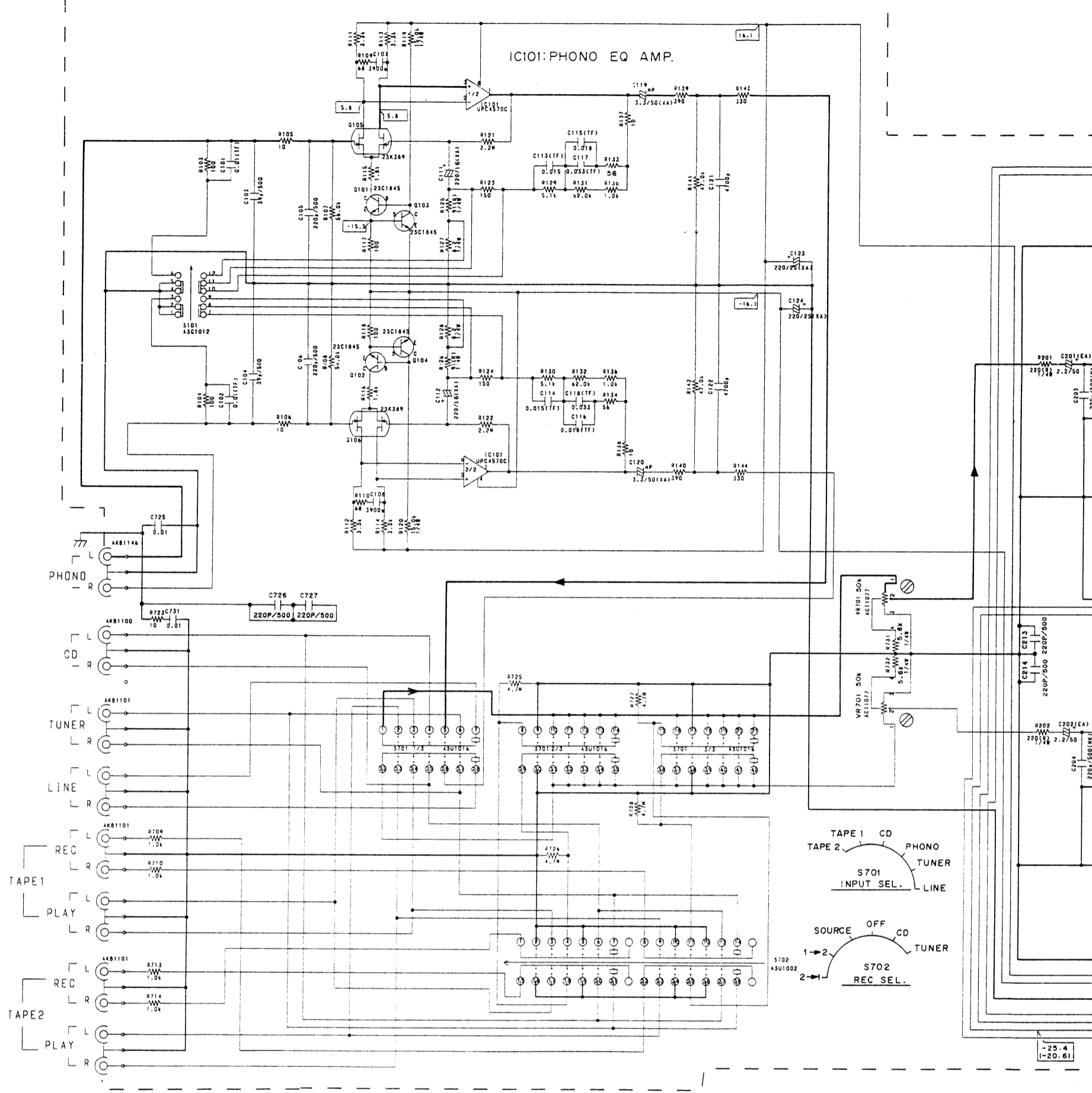
AF COMPLEX ASS'Y (AWZ4961:HB TYPE) (AWZ4962:HL AND YPW TYPES)
