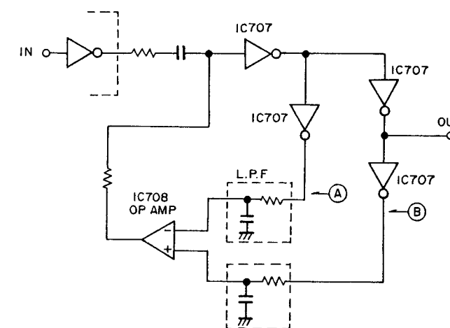
Fig 2 Optical Transmission Compensating Circuit
