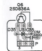
SOCKET Ass'y (B)
