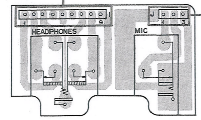
JACK Ass'y
