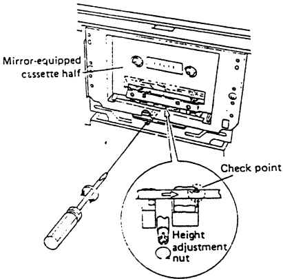
Fig. 11-5 Tape transport adjustment
