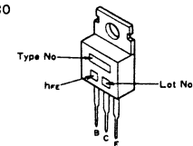
BA6109
